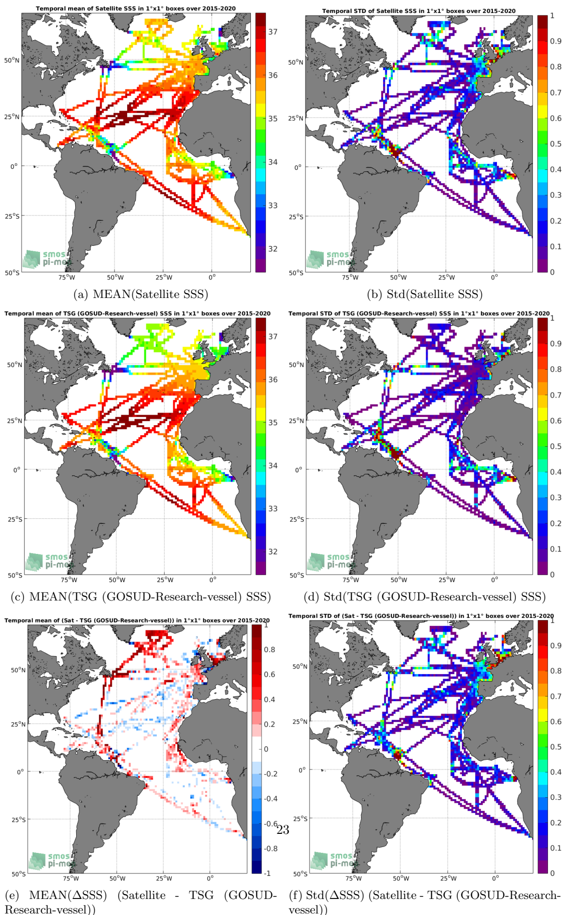
Figure 6: Temporal mean (left) and Std (right) of SSS from SMAP SSS L3 v5.0 - 8-Day running (JPL) (top), TSG (GOSUD-Research-vessel) (middle), and of \Delta SSS (Satellite - TSG (GOSUD-Research-vessel)). Only match-up pairs are used to generate these maps.
