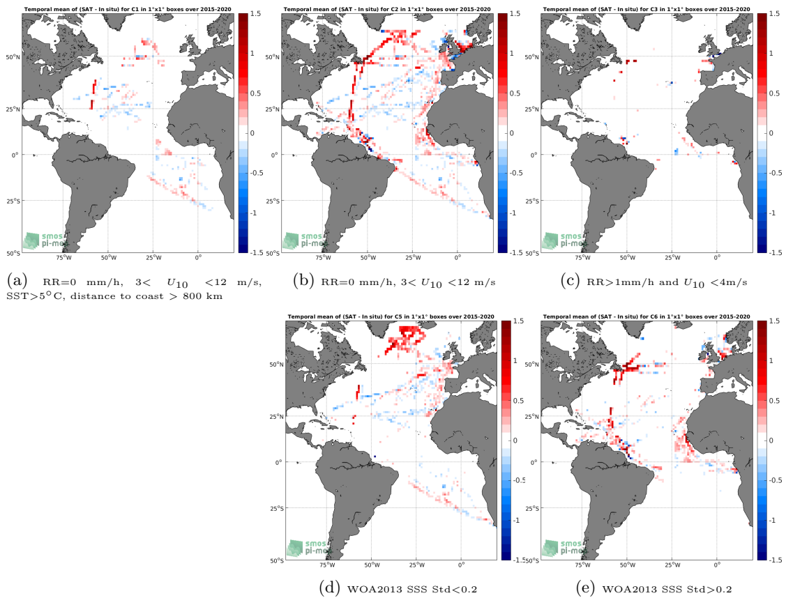
Figure 12: Temporal mean gridded over spatial boxes of size 1^\circ \times 1^\circ of \Delta SSS (SMAP SSS L3 v5.0 - 8-Day running (JPL) - TSG (GOSUD-Research-vessel)) for 5 different subdatasets corresponding to:RR=0 mm/h, 3 < U_{10} < 12 m/s, SST>5°C, distance to coast > 800 km (a), RR=0 mm/h, 3 < U_{10} < 12 m/s (b), RR>1mm/h and U_{10} < 4 m/s (c), WOA2013 SSS Std<0.2 (d), WOA2013 SSS Std>0.2 (e).
