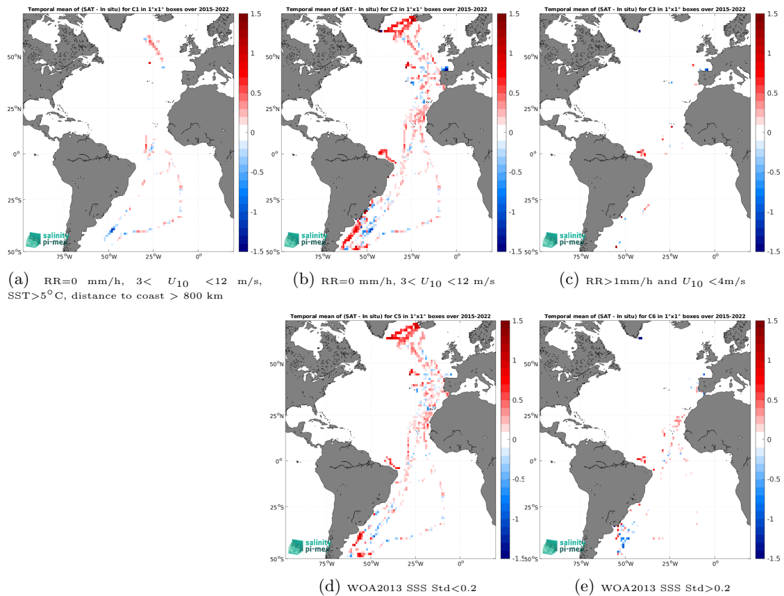
Figure 14: Temporal mean gridded over spatial boxes of size 1^\circ \times 1^\circ of \Delta SSS (SMAP SSS L3 v5.0 - 8-Day running (JPL) - TSG (CSIC-UTM)) for 5 different subdatasets corresponding to:RR=0 mm/h, 3 < U_{10} < 12 m/s, SST >5^\circ\text{C} , distance to coast > 800 km (a), RR=0 mm/h, 3 < U_{10} < 12 m/s (b), RR >1 mm/h and U_{10} < 4 m/s (c), WOA2013 SSS Std <0.2 (d), WOA2013 SSS Std >0.2 (e).
