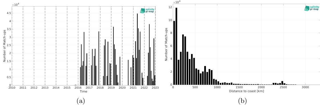
Figure 2: Number of match-ups between TSG (CSIC-UTM) and SMAP SSS L3 v5.0 - 8-Day running (JPL) SSS as a function of time (a) and as function of the distance to coast (b) over the Atlantic Ocean Pi-MEP region and for the full satellite product period.
