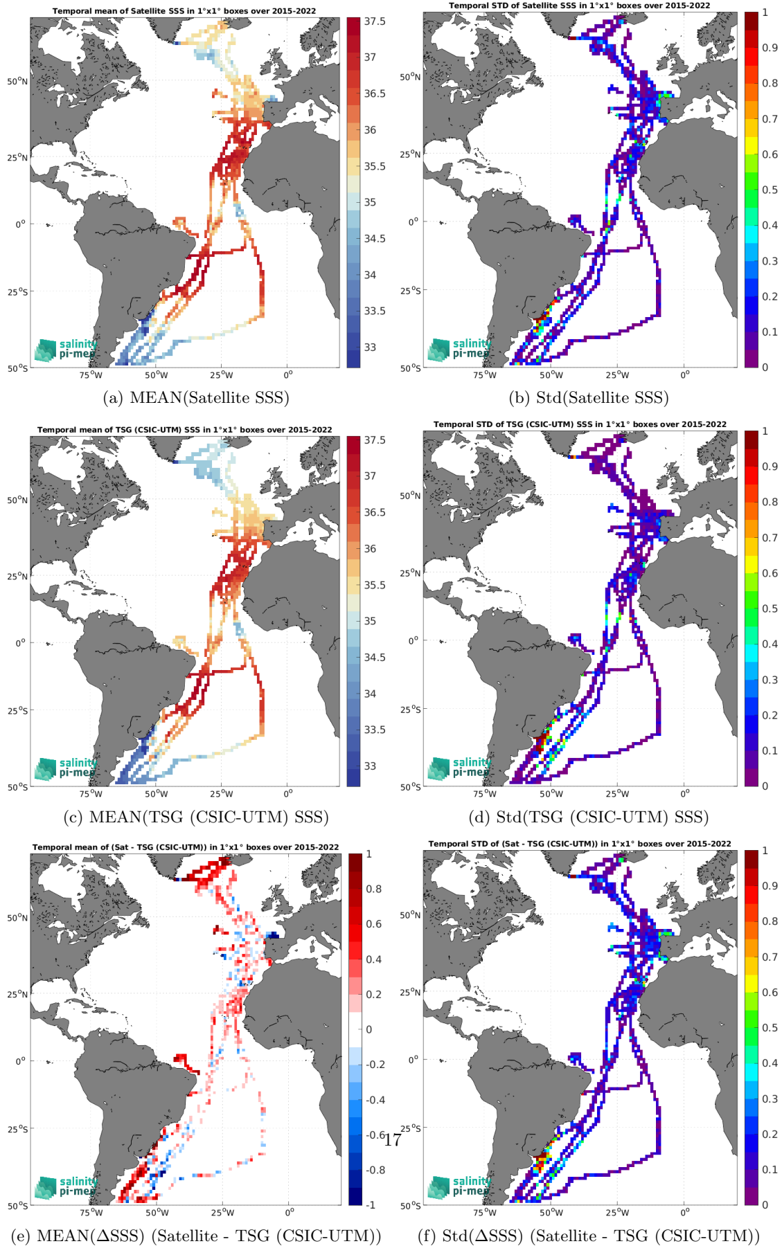
Figure 7: Temporal mean (left) and Std (right) of SSS from SMAP SSS L3 v5.0 - 8-Day running (JPL) (top), TSG (CSIC-UTM) (middle), and of \Delta SSS (Satellite - TSG (CSIC-UTM)). Only match-up pairs are used to generate these maps.
