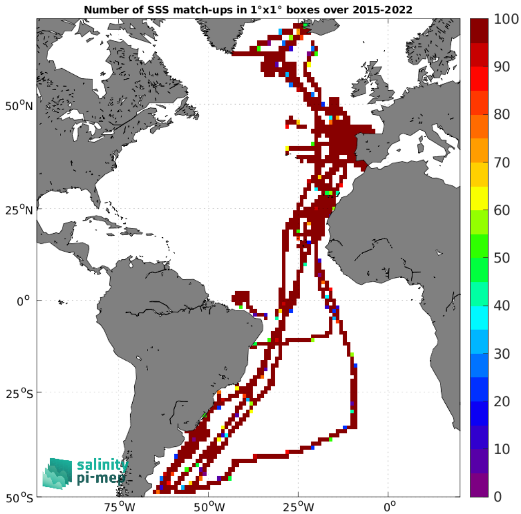
Figure 5: Number of SSS match-ups between TSG (CSIC-UTM) SSS and the SMAP SSS L3 v5.0 - 8-Day running (JPL) SSS product for the Atlantic Ocean Pi-MEP region over 1^\circ \times 1^\circ boxes and for the full satellite product period.
