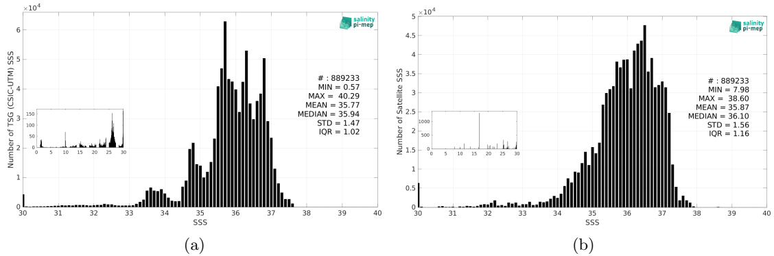
Figure 3: Histograms of SSS from TSG (CSIC-UTM) (a) and SMAP SSS L3 v5.0 - 8-Day running (JPL) (b) considering all match-up pairs per bins of 0.1 over the Atlantic Ocean Pi-MEP region and for the full satellite product period.
