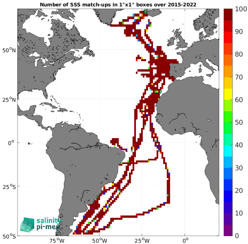
Figure 4: Number of SSS match-ups between TSG (CSIC-UTM) SSS and the SMAP SSS L3 v5.0 - 8-Day running (JPL) SSS product for the Atlantic Ocean Pi-MEP region over 1^\circ \times 1^\circ boxes and for the full satellite product period.
