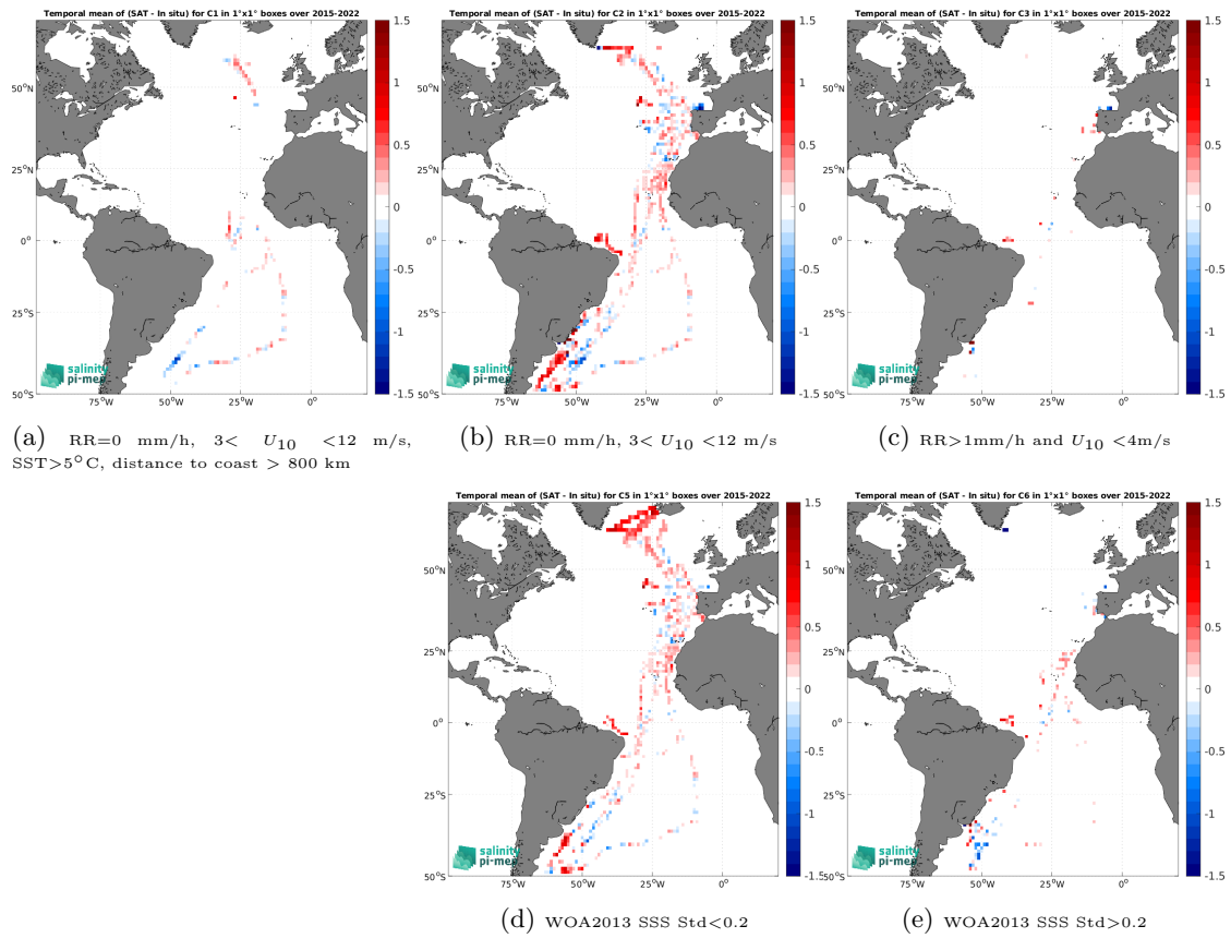
Figure 12: Temporal mean gridded over spatial boxes of size 1^\circ \times 1^\circ of \Delta SSS (SMAP SSS L3 v5.0 - 8-Day running (JPL) - TSG (CSIC-UTM)) for 5 different subdatasets corresponding to:RR=0 mm/h, 3 < U_{10} < 12 m/s, SST >5^\circ\text{C} , distance to coast > 800 km (a), RR=0 mm/h, 3 < U_{10} < 12 m/s (b), RR >1 mm/h and U_{10} < 4 m/s (c), WOA2013 SSS Std <0.2 (d), WOA2013 SSS Std >0.2 (e).
