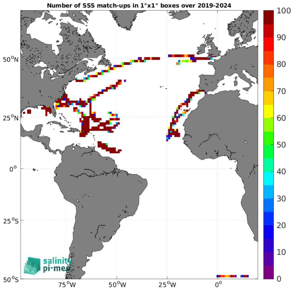
Figure 5: Number of SSS match-ups between Saildrone SSS and the SMAP SSS L3 v5.0 - 8-Day running (JPL) SSS product for the Atlantic Ocean Pi-MEP region over 1^\circ \times 1^\circ boxes and for the full satellite product period.
