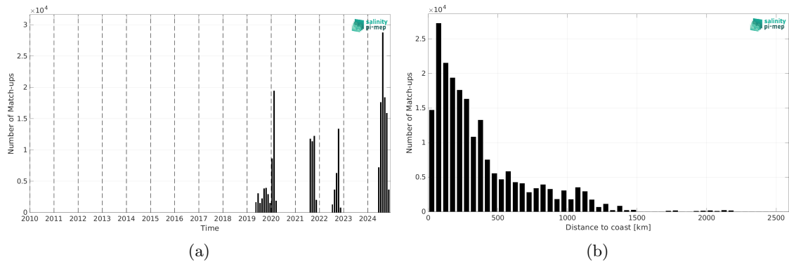
Figure 2: Number of match-ups between Sairdrone and SMAP SSS L3 v5.0 - 8-Day running (JPL) SSS as a function of time (a) and as function of the distance to coast (b) over the Atlantic Ocean Pi-MEP region and for the full satellite product period.
