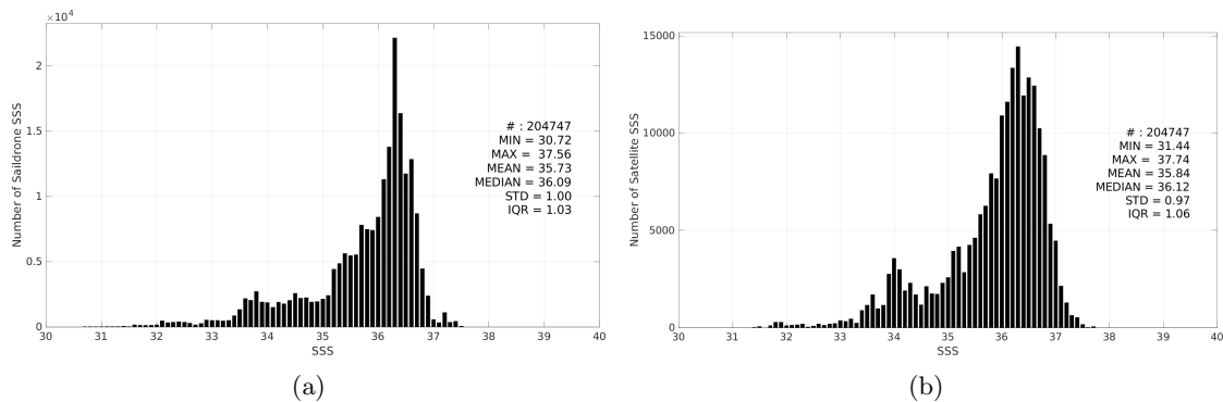
Figure 3: Histograms of SSS from Sairdrone (a) and SMAP SSS L3 v5.0 - 8-Day running (JPL) (b) considering all match-up pairs per bins of 0.1 over the Atlantic Ocean Pi-MEP region and for the full satellite product period.
