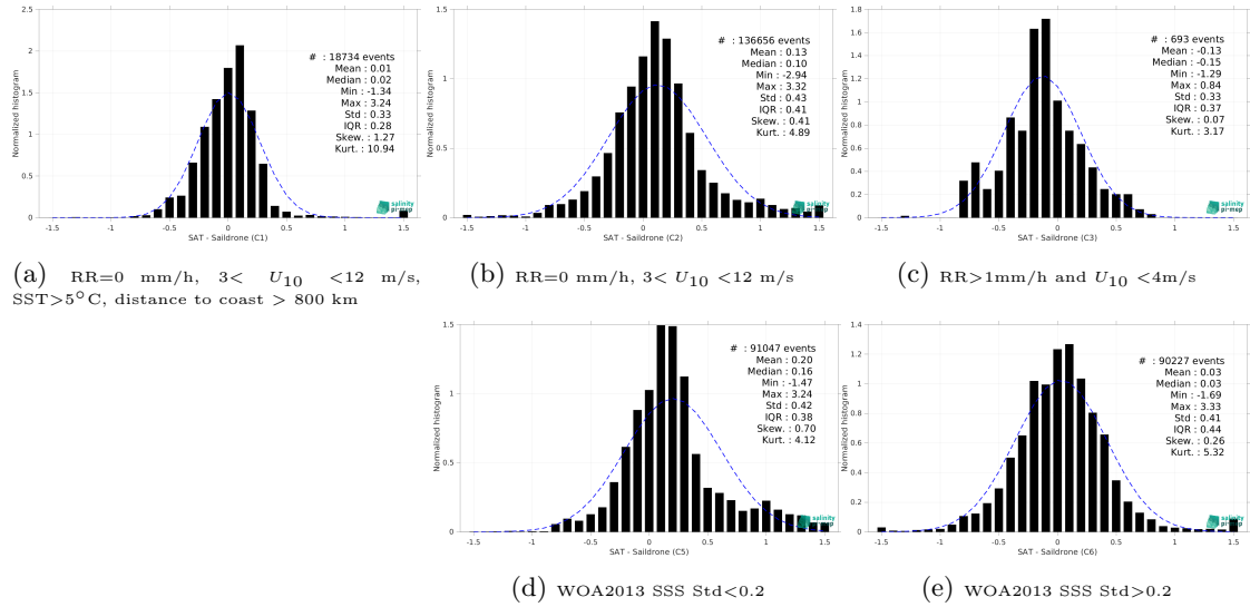
Figure 15: Normalized histogram of \Delta\text{SSS} (SMAP SSS L3 v5.0 - 8-Day running (JPL) - Saiclone) for 5 different subdatasets corresponding to: RR=0 mm/h, 3 < U_{10} < 12 m/s, SST>5°C, distance to coast > 800 km (a), RR=0 mm/h, 3 < U_{10} < 12 m/s (b), RR>1mm/h and U_{10} < 4 m/s (c), WOA2013 SSS Std<0.2 (d), WOA2013 SSS Std>0.2 (e).
