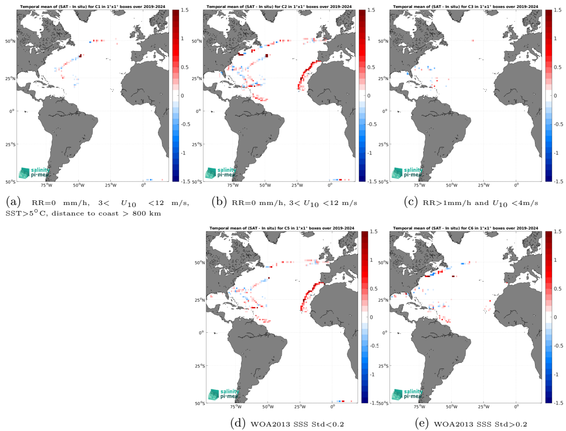
Figure 14: Temporal mean gridded over spatial boxes of size 1^\circ \times 1^\circ of \Delta SSS (SMAP SSS L3 v5.0 - 8-Day running (JPL) - Saicdrone) for 5 different subdatasets corresponding to:RR=0 mm/h, 3 < U_{10} < 12 m/s, SST>5°C, distance to coast > 800 km (a), RR=0 mm/h, 3 < U_{10} < 12 m/s (b), RR>1mm/h and U_{10} < 4 m/s (c), WOA2013 SSS Std<0.2 (d), WOA2013 SSS Std>0.2 (e).
