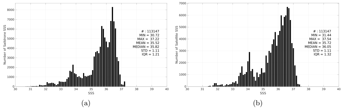
Figure 3: Histograms of SSS from Sairdrone (a) and SMAP SSS L3 v5.0 - 8-Day running (JPL) (b) considering all match-up pairs per bins of 0.1 over the Atlantic Ocean Pi-MEP region and for the full satellite product period.
