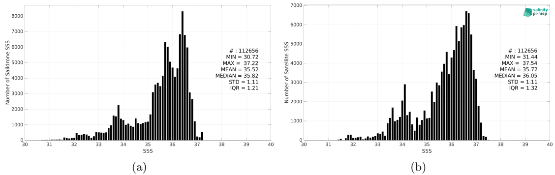
Figure 2: Histograms of SSS from Sairdrone (a) and SMAP SSS L3 v5.0 - 8-Day running (JPL) (b) considering all match-up pairs per bins of 0.1 over the Atlantic Ocean Pi-MEP region and for the full satellite product period.
