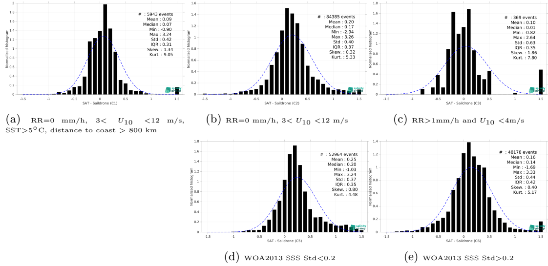
Figure 13: Normalized histogram of \Delta SSS (SMAP SSS L3 v5.0 - 8-Day running (JPL) - Salsdrone) for 5 different subdatasets corresponding to: RR=0 mm/h, 3 < U_{10} < 12 m/s, SST > 5°C, distance to coast > 800 km (a), RR=0 mm/h, 3 < U_{10} < 12 m/s (b), RR > 1mm/h and U_{10} < 4 m/s (c), WOA2013 SSS Std < 0.2 (d), WOA2013 SSS Std > 0.2 (e).
