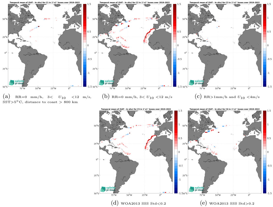
Figure 12: Temporal mean gridded over spatial boxes of size 1^\circ \times 1^\circ of \Delta SSS (SMAP SSS L3 v5.0 - 8-Day running (JPL) - Saicdrone) for 5 different subdatasets corresponding to:RR=0 mm/h, 3 < U_{10} < 12 m/s, SST >5^\circ\text{C} , distance to coast > 800 km (a), RR=0 mm/h, 3 < U_{10} < 12 m/s (b), RR >1 mm/h and U_{10} < 4 m/s (c), WOA2013 SSS Std <0.2 (d), WOA2013 SSS Std >0.2 (e).
