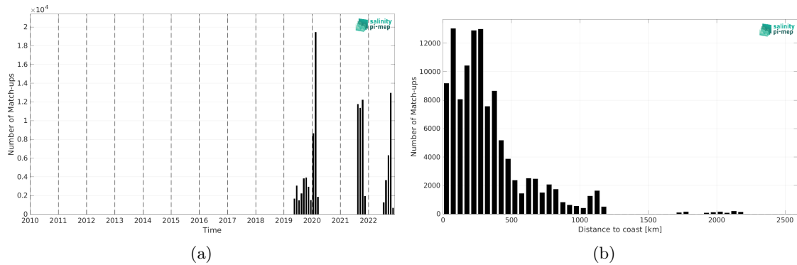
Figure 1: Number of match-ups between Sairdrone and SMAP SSS L3 v5.0 - 8-Day running (JPL) SSS as a function of time (a) and as function of the distance to coast (b) over the Atlantic Ocean Pi-MEP region and for the full satellite product period.
