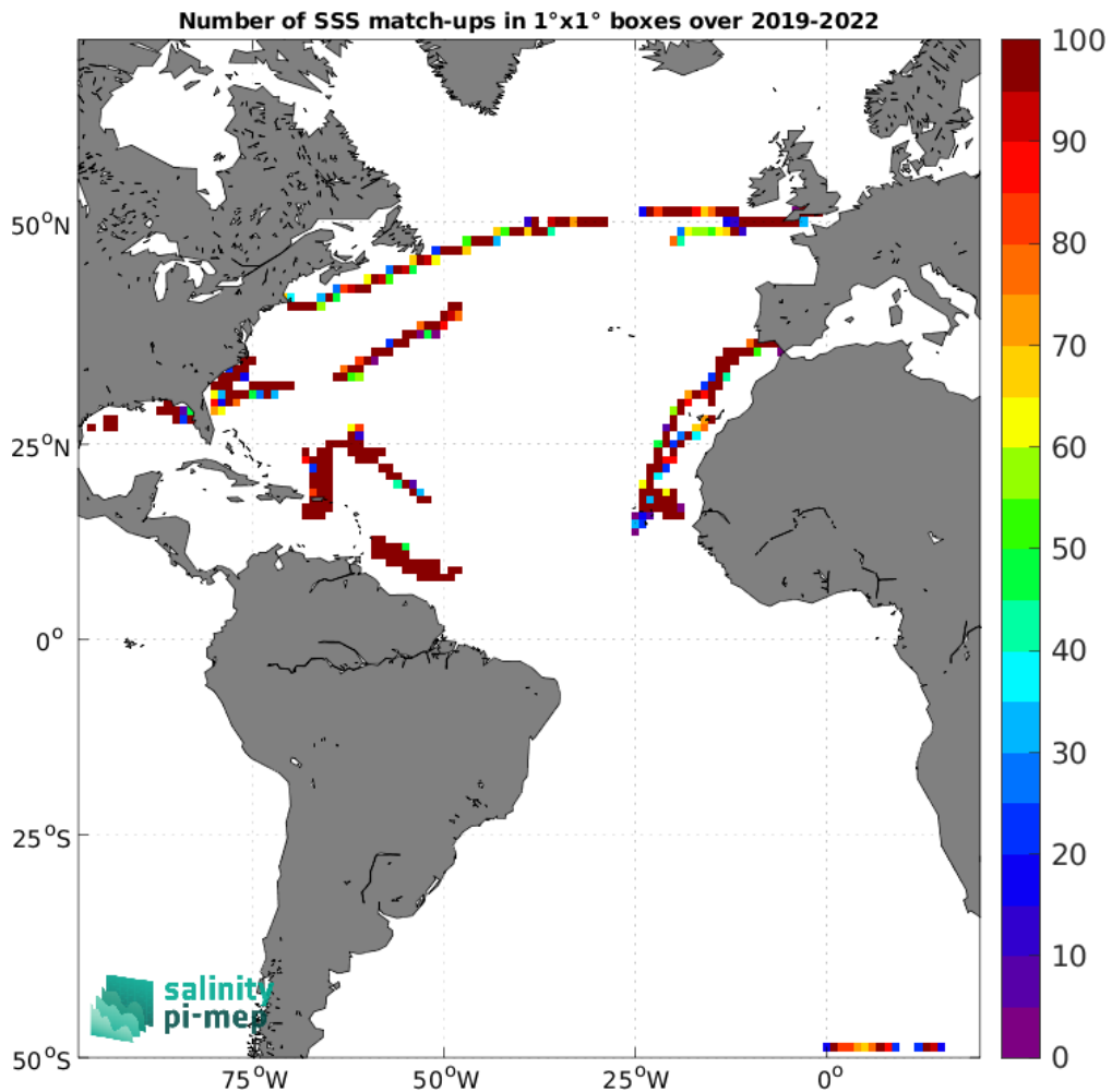
Figure 4: Number of SSS match-ups between Saildrone SSS and the SMAP SSS L3 v5.0 - 8-Day running (JPL) SSS product for the Atlantic Ocean Pi-MEP region over 1^\circ \times 1^\circ boxes and for the full satellite product period.
