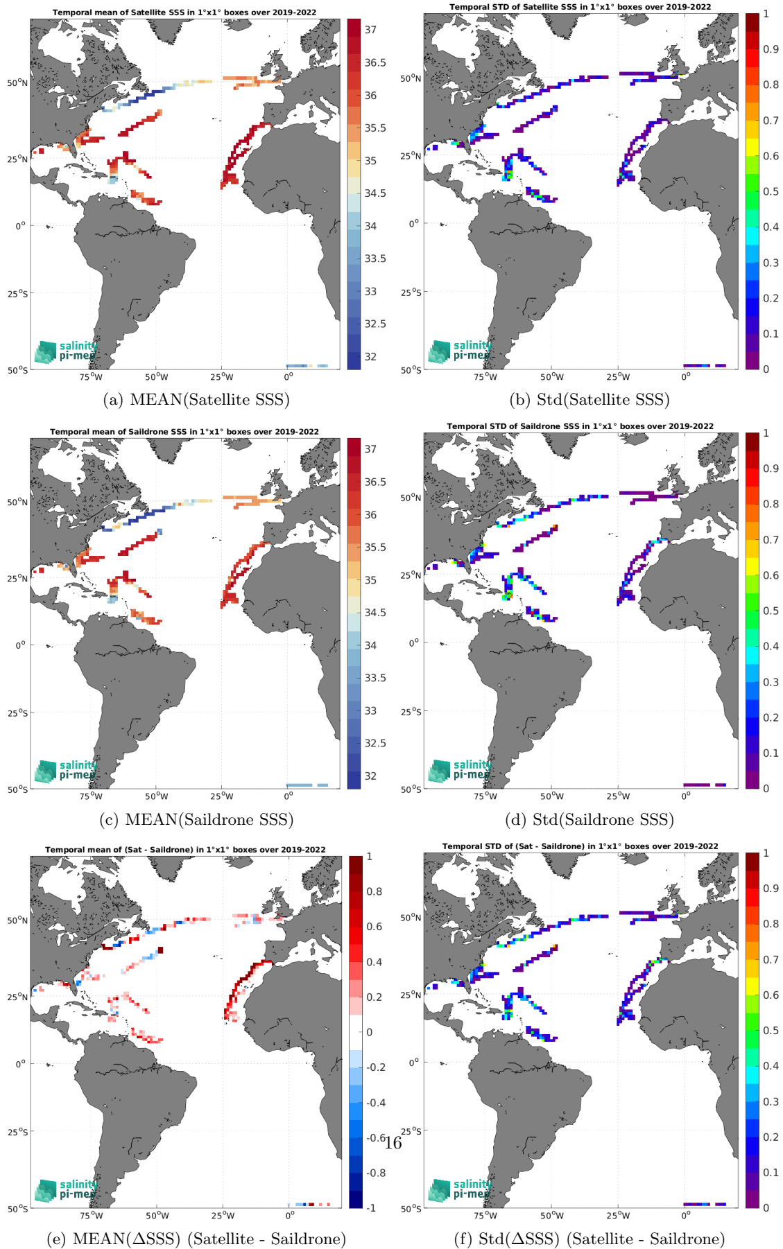
Figure 6: Temporal mean (left) and Std (right) of SSS from SMAP SSS L3 v5.0 - 8-Day running (JPL) (top), Saildrone (middle), and of \Delta SSS (Satellite - Saildrone). Only match-up pairs are used to generate these maps.
