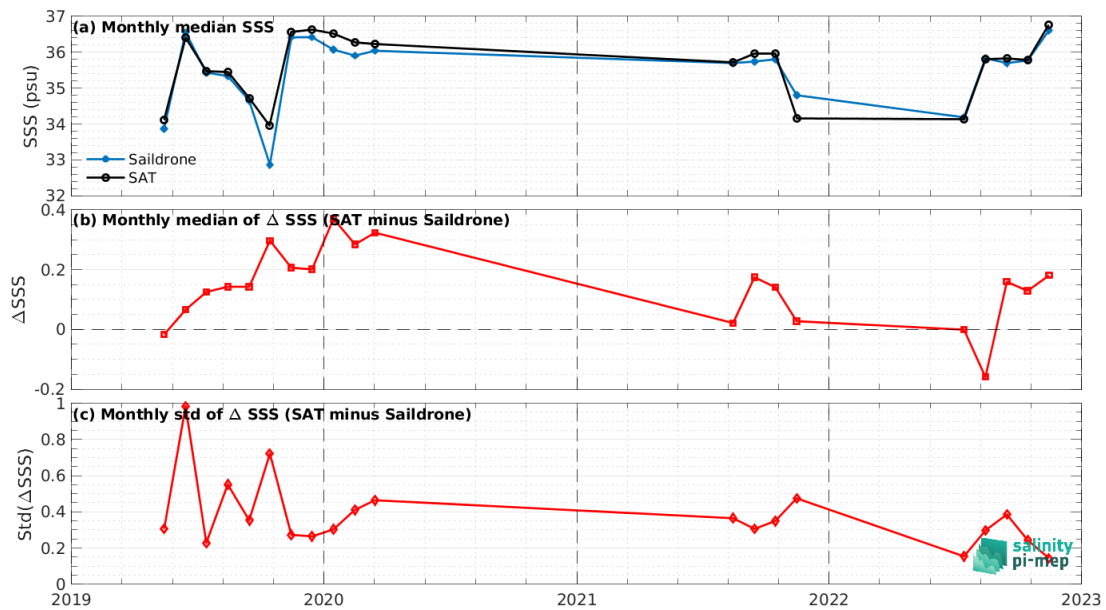
Figure 7: Time series of the monthly median SSS (top), median of \Delta SSS (Satellite - Sairdronne) and Std of \Delta SSS (Satellite - Sairdronne) over the Atlantic Ocean Pi-MEP region considering all match-ups collected by the Pi-MEP.
