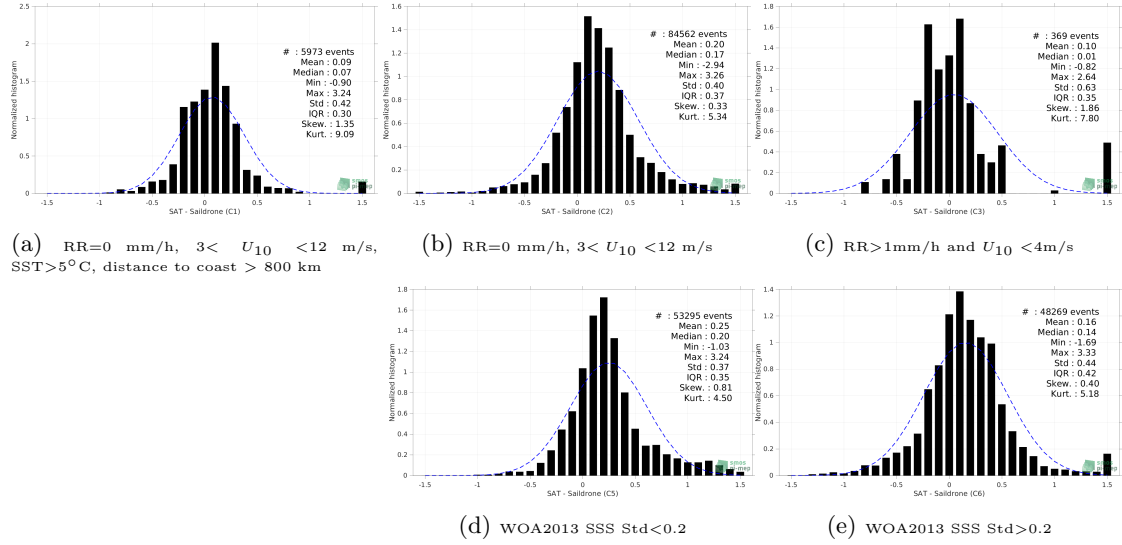
Figure 13: Normalized histogram of \Delta SSS (SMAP SSS L3 v5.0 - 8-Day running (JPL) - Salsdrone) for 5 different subdatasets corresponding to: RR=0 mm/h, 3 < U_{10} < 12 m/s, SST>5°C, distance to coast > 800 km (a), RR=0 mm/h, 3 < U_{10} < 12 m/s (b), RR>1mm/h and U_{10} < 4 m/s (c), WOA2013 SSS Std<0.2 (d), WOA2013 SSS Std>0.2 (e).
