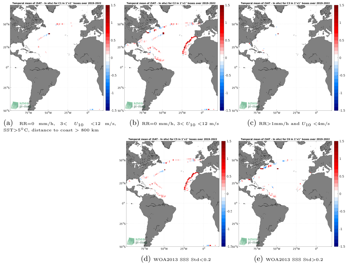
Figure 12: Temporal mean gridded over spatial boxes of size 1^\circ \times 1^\circ of \Delta SSS (SMAP SSS L3 v5.0 - 8-Day running (JPL) - Saicdrone) for 5 different subdatasets corresponding to:RR=0 mm/h, 3 < U_{10} < 12 m/s, SST >5^\circ\text{C} , distance to coast > 800 km (a), RR=0 mm/h, 3 < U_{10} < 12 m/s (b), RR >1 mm/h and U_{10} < 4 m/s (c), WOA2013 SSS Std <0.2 (d), WOA2013 SSS Std >0.2 (e).
