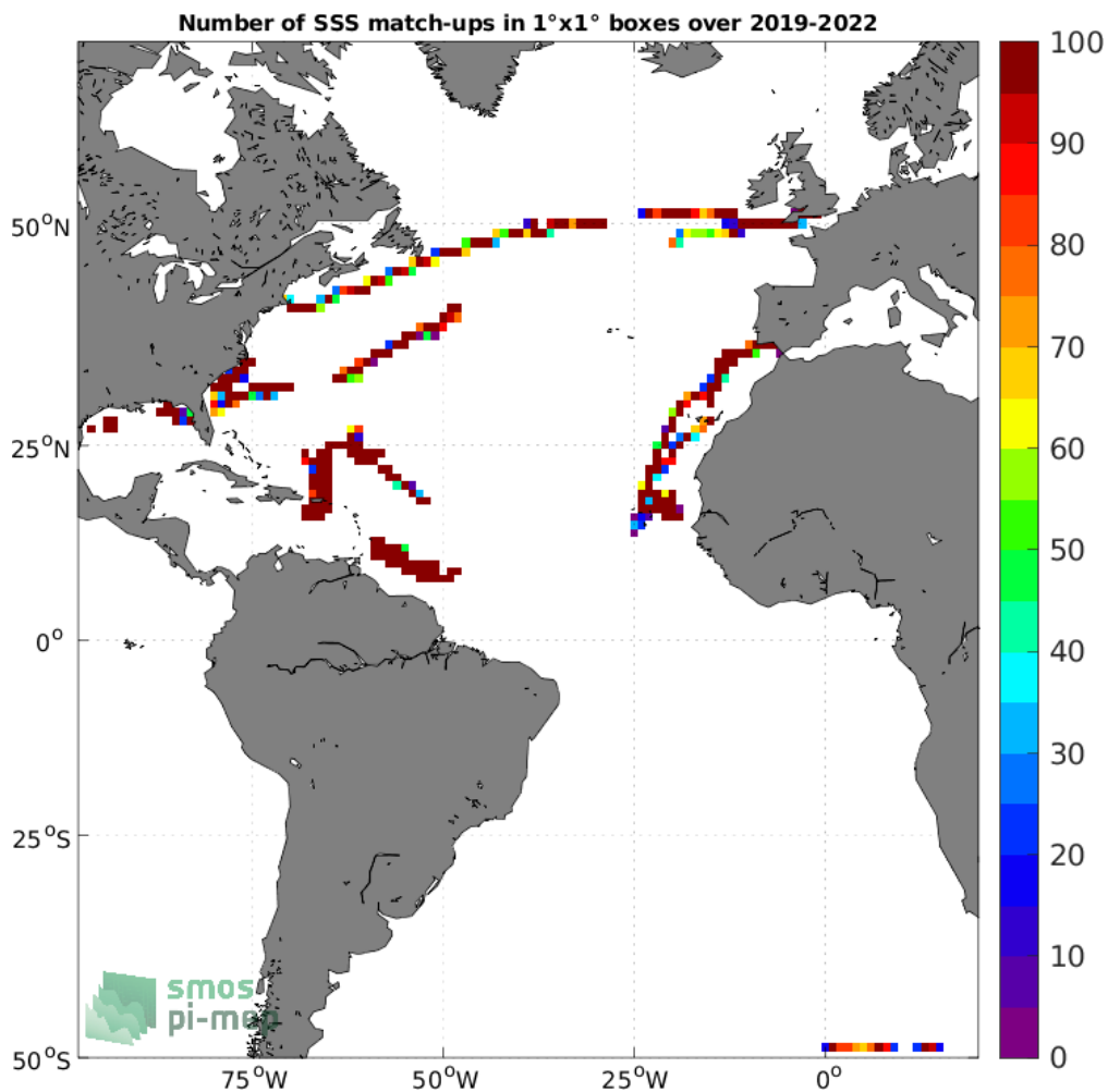
Figure 4: Number of SSS match-ups between Saildrone SSS and the SMAP SSS L3 v5.0 - 8-Day running (JPL) SSS product for the Atlantic Ocean Pi-MEP region over 1°×1° boxes and for the full satellite product period.
