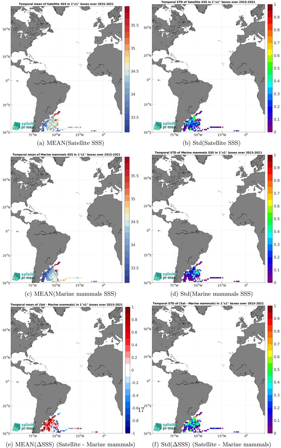
Figure 7: Temporal mean (left) and Std (right) of SSS from SMAP SSS L3 v5.0 - 8-Day running (JPL) (top), Marine mammals (middle), and of \Delta\text{SSS} (Satellite - Marine mammals). Only match-up pairs are used to generate these maps.
