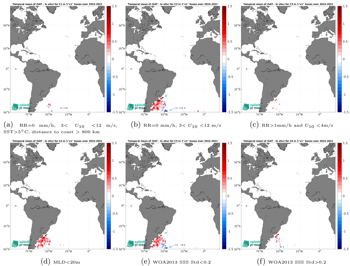
Figure 14: Temporal mean gridded over spatial boxes of size 1^\circ \times 1^\circ of \Delta SSS (SMAP SSS L3 v5.0 - 8-Day running (JPL) - Marine mammals) for 6 different subdatasets corresponding to:RR=0 mm/h, 3 < U_{10} < 12 m/s, SST >5^\circ C, distance to coast > 800 km (a), RR=0 mm/h, 3 < U_{10} < 12 m/s (b), RR >1 mm/h and U_{10} < 4 m/s (c),MLD <20 m (d),WOA2013 SSS Std <0.2 (e),WOA2013 SSS Std >0.2 (f).
