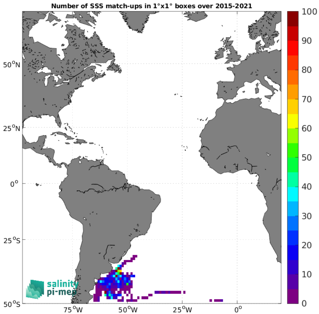
Figure 5: Number of SSS match-ups between Marine mammals SSS and the SMAP SSS L3 v5.0 - 8-Day running (JPL) SSS product for the Atlantic Ocean Pi-MEP region over 1°×1° boxes and for the full satellite product period.
