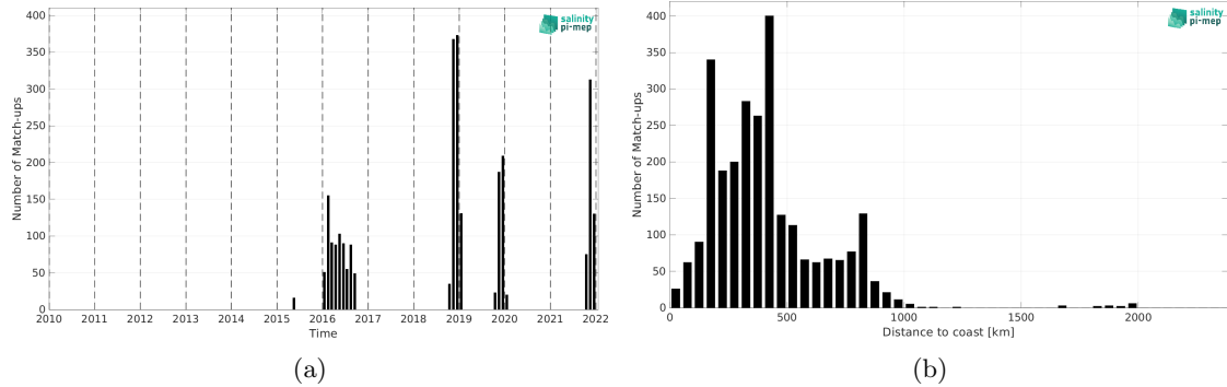
Figure 2: Number of match-ups between Marine mammals and SMAP SSS L3 v5.0 - 8-Day running (JPL) SSS as a function of time (a) and as function of the distance to coast (b) over the Atlantic Ocean Pi-MEP region and for the full satellite product period.
