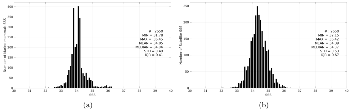
Figure 3: Histograms of SSS from Marine mammals (a) and SMAP SSS L3 v5.0 - 8-Day running (JPL) (b) considering all match-up pairs per bins of 0.1 over the Atlantic Ocean Pi-MEP region and for the full satellite product period.
