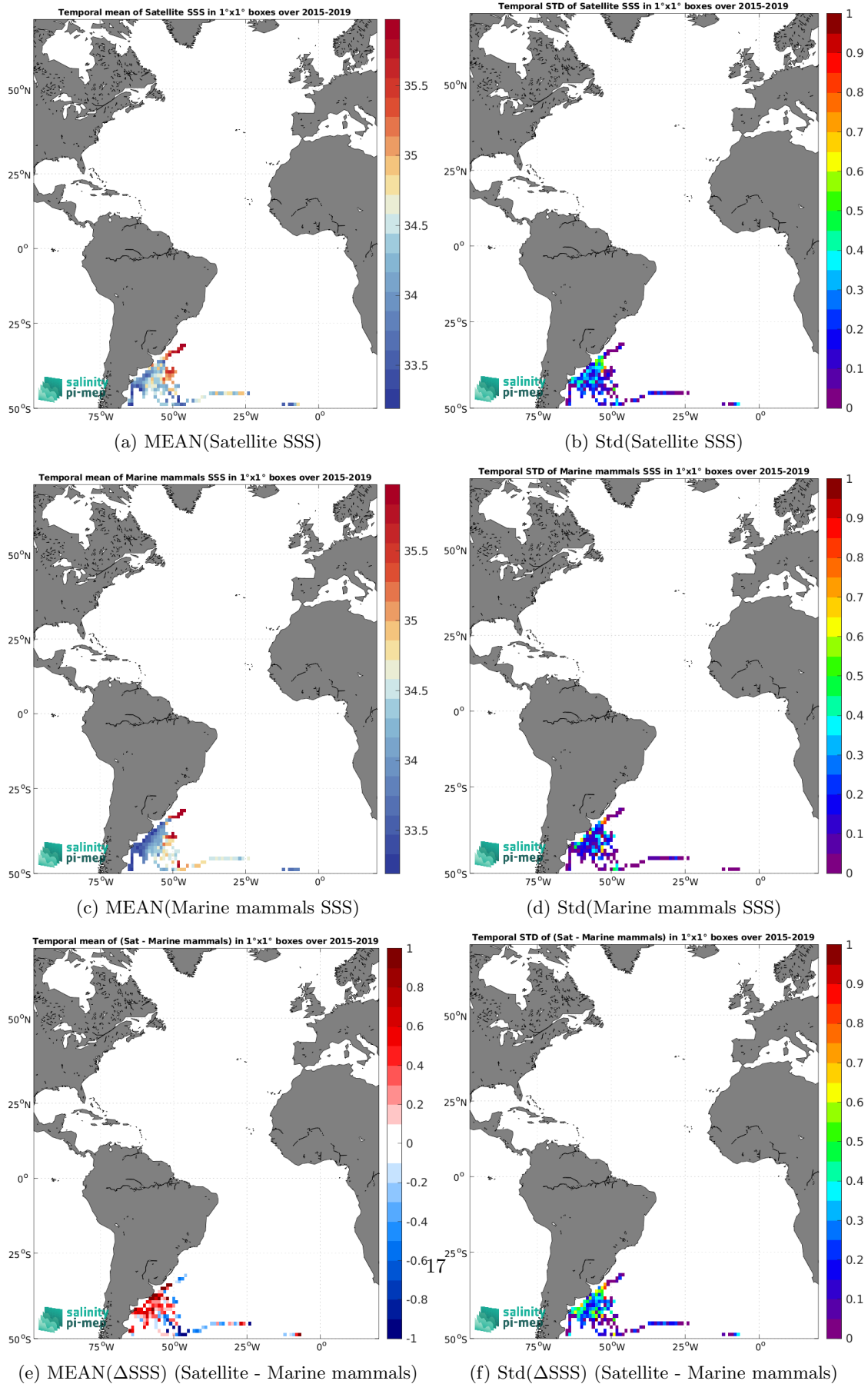
Figure 6: Temporal mean (left) and Std (right) of SSS from SMAP SSS L3 v5.0 - 8-Day running (JPL) (top), Marine mammals (middle), and of \Delta\text{SSS} (Satellite - Marine mammals). Only match-up pairs are used to generate these maps.
