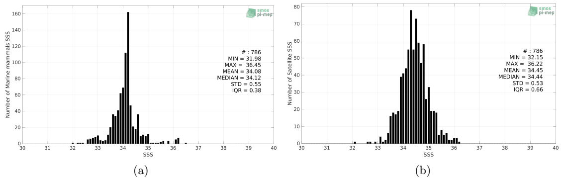
Figure 2: Histograms of SSS from Marine mammals (a) and SMAP SSS L3 v5.0 - 8-Day running (JPL) (b) considering all match-up pairs per bins of 0.1 over the Atlantic Ocean Pi-MEP region and for the full satellite product period.
