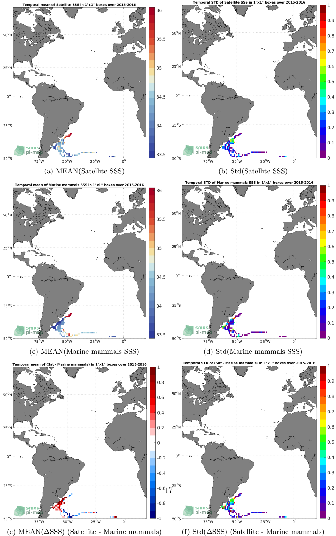
Figure 6: Temporal mean (left) and Std (right) of SSS from SMAP SSS L3 v5.0 - 8-Day running (JPL) (top), Marine mammals (middle), and of \Delta SSS (Satellite - Marine mammals). Only match-up pairs are used to generate these maps.
