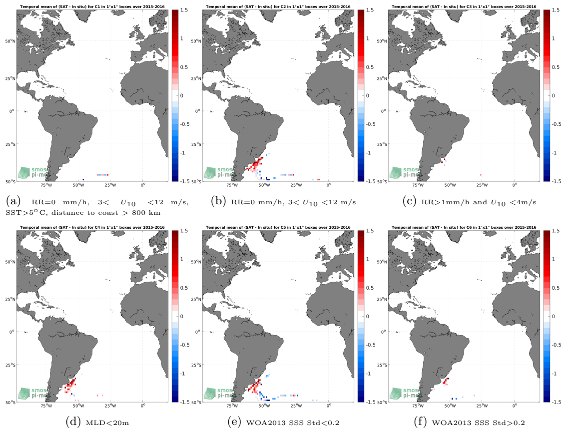
Figure 12: Temporal mean gridded over spatial boxes of size 1^\circ \times 1^\circ of \Delta SSS (SMAP SSS L3 v5.0 - 8-Day running (JPL) - Marine mammals) for 6 different subdatasets corresponding to:RR=0 mm/h, 3 < U_{10} < 12 m/s, SST >5^\circ C, distance to coast > 800 km (a), RR=0 mm/h, 3 < U_{10} < 12 m/s (b), RR >1 mm/h and U_{10} < 4 m/s (c),MLD <20 m (d),WOA2013 SSS Std <0.2 (e),WOA2013 SSS Std >0.2 (f).
