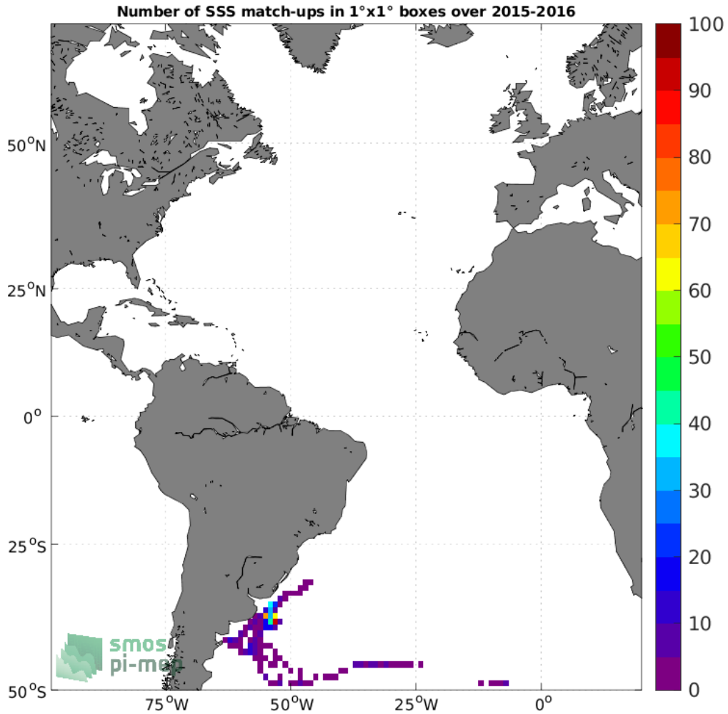
Figure 4: Number of SSS match-ups between Marine mammals SSS and the SMAP SSS L3 v5.0 - 8-Day running (JPL) SSS product for the Atlantic Ocean Pi-MEP region over 1°×1° boxes and for the full satellite product period.
