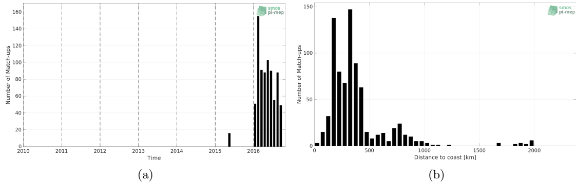
Figure 1: Number of match-ups between Marine mammals and SMAP SSS L3 v5.0 - 8-Day running (JPL) SSS as a function of time (a) and as function of the distance to coast (b) over the Atlantic Ocean Pi-MEP region and for the full satellite product period.
