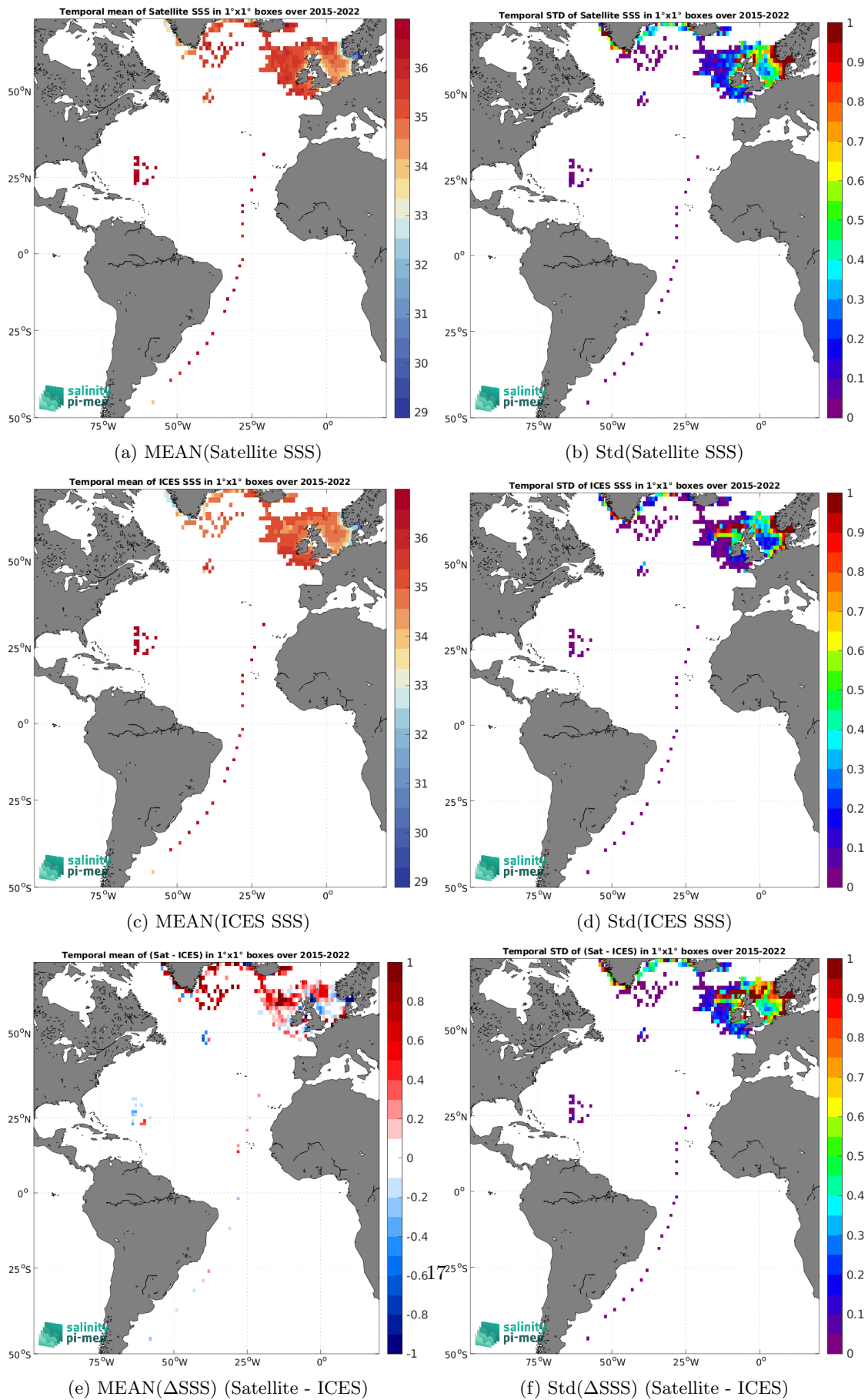
Figure 7: Temporal mean (left) and Std (right) of SSS from SMAP SSS L3 v5.0 - 8-Day running (JPL) (top), ICES (middle), and of \Delta\text{SSS} (Satellite - ICES). Only match-up pairs are used to generate these maps.
