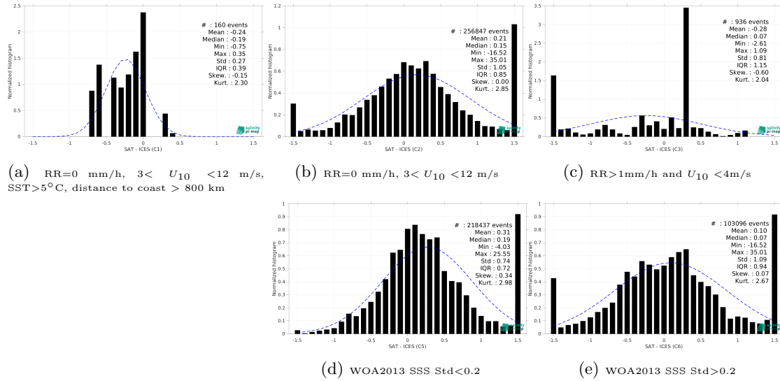
Figure 13: Normalized histogram of \Delta SSS (SMAP SSS L3 v5.0 - 8-Day running (JPL) - ICES) for 5 different subdatasets corresponding to: RR=0 mm/h, 3 < U_{10} < 12 m/s, SST > 5°C, distance to coast > 800 km (a), RR=0 mm/h, 3 < U_{10} < 12 m/s (b), RR > 1mm/h and U_{10} < 4 m/s (c), WOA2013 SSS Std < 0.2 (d), WOA2013 SSS Std > 0.2 (e).
