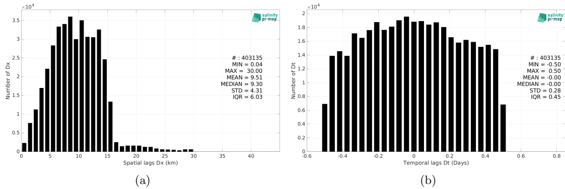
Figure 5: Histograms of the spatial (a) and temporal (b) lags between the location/time of the ICES measurement and the date of the corresponding SMAP SSS L3 v5.0 - 8-Day running (JPL) SSS pixel.
