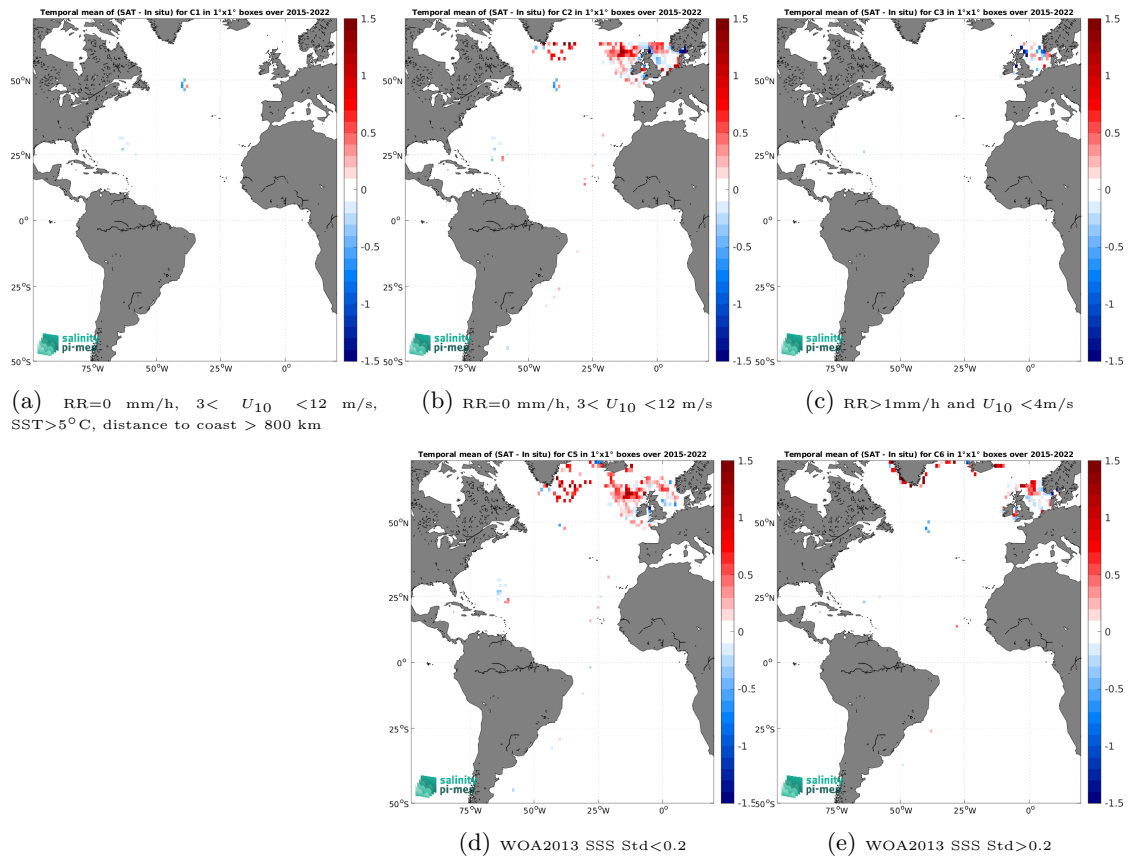
Figure 12: Temporal mean gridded over spatial boxes of size 1^\circ \times 1^\circ of \Delta SSS (SMAP SSS L3 v5.0 - 8-Day running (JPL) - ICES) for 5 different subdatasets corresponding to:RR=0 mm/h, 3 < U_{10} < 12 m/s, SST >5^\circ\text{C} , distance to coast > 800 km (a), RR=0 mm/h, 3 < U_{10} < 12 m/s (b), RR >1 mm/h and U_{10} < 4 m/s (c), WOA2013 SSS Std <0.2 (d), WOA2013 SSS Std >0.2 (e).
