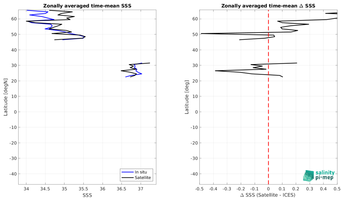
Figure 8: Left panel: Zonal mean SSS from SMAP SSS L3 v5.0 - 8-Day running (JPL) satellite product (black) and from ICES (blue). Right panel: Zonal mean of \Delta SSS (Satellite - ICES) for all the collected Pi-MEP match-up pairs estimated over the full satellite product period.
