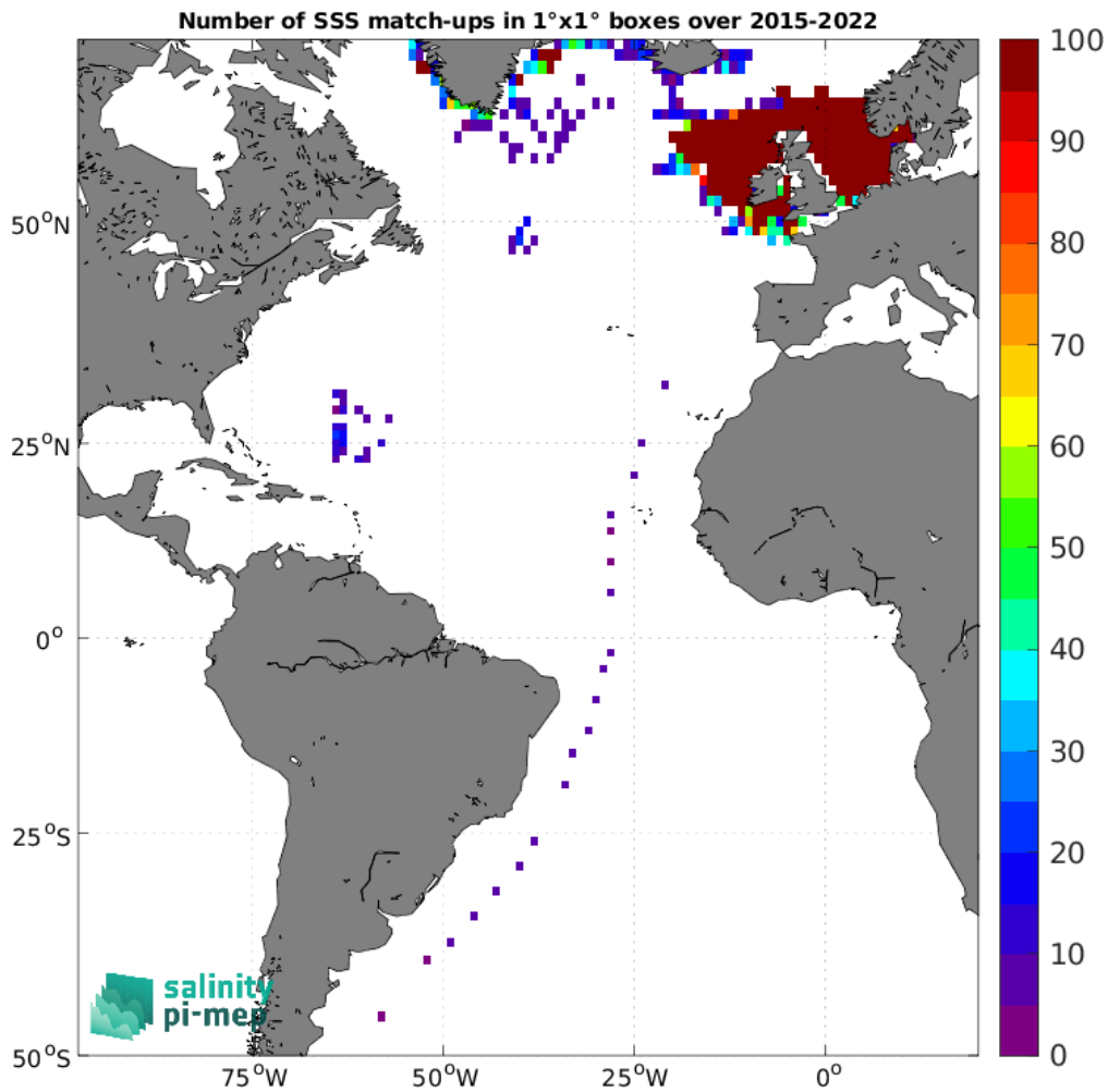
Figure 4: Number of SSS match-ups between ICES SSS and the SMAP SSS L3 v5.0 - 8-Day running (JPL) SSS product for the Atlantic Ocean Pi-MEP region over 1^\circ \times 1^\circ boxes and for the full satellite product period.
