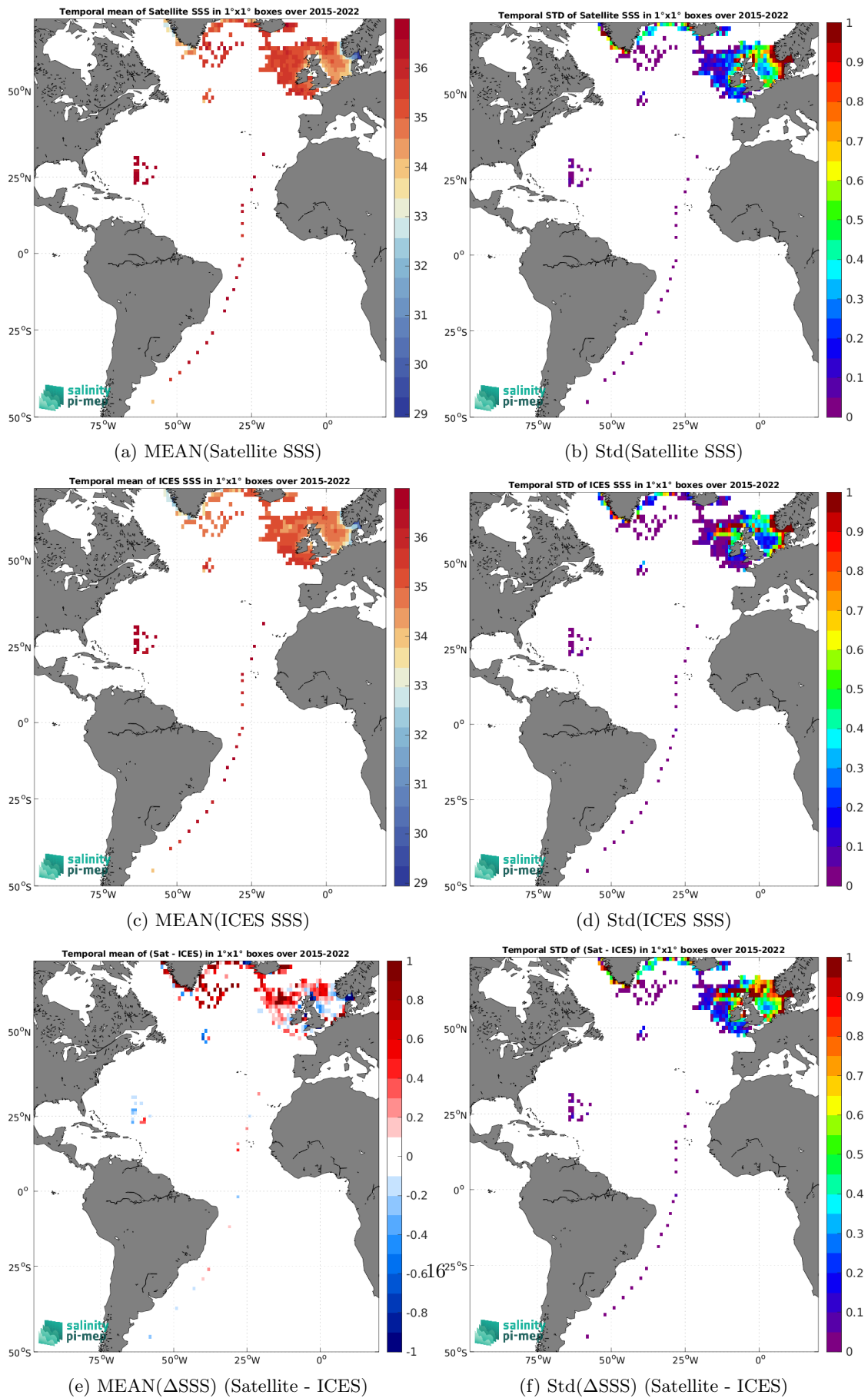
Figure 6: Temporal mean (left) and Std (right) of SSS from SMAP SSS L3 v5.0 - 8-Day running (JPL) (top), ICES (middle), and of \Delta SSS (Satellite - ICES). Only match-up pairs are used to generate these maps.
