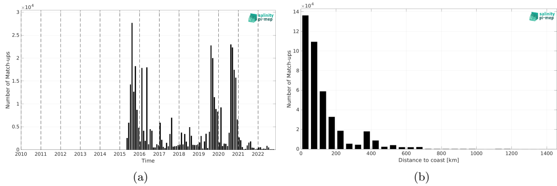
Figure 1: Number of match-ups between ICES and SMAP SSS L3 v5.0 - 8-Day running (JPL) SSS as a function of time (a) and as function of the distance to coast (b) over the Atlantic Ocean Pi-MEP region and for the full satellite product period.
