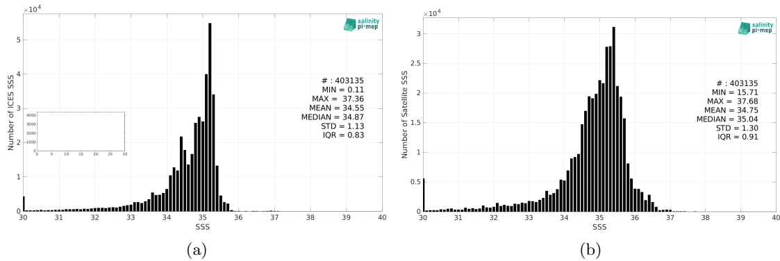
Figure 2: Histograms of SSS from ICES (a) and SMAP SSS L3 v5.0 - 8-Day running (JPL) (b) considering all match-up pairs per bins of 0.1 over the Atlantic Ocean Pi-MEP region and for the full satellite product period.
