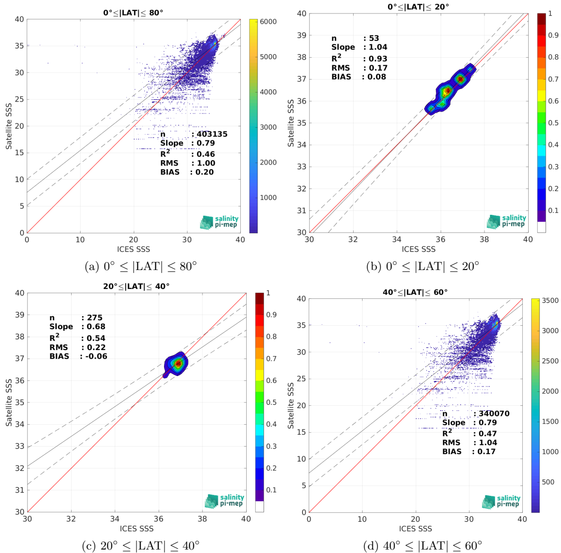
Figure 9: Contour maps of the concentration of SMAP SSS L3 v5.0 - 8-Day running (JPL) SSS (y-axis) versus ICES SSS (x-axis) at match-up pairs for different latitude bands. For each plot, the red line shows x=y . The black thin and dashed lines indicate a linear fit through the data cloud and the \pm 95\% confidence levels, respectively. The number match-up pairs n , the slope and R^2 coefficient of the linear fit, the root mean square (RMS) and the mean bias between satellite and in situ data are indicated for each latitude band in each plots.
