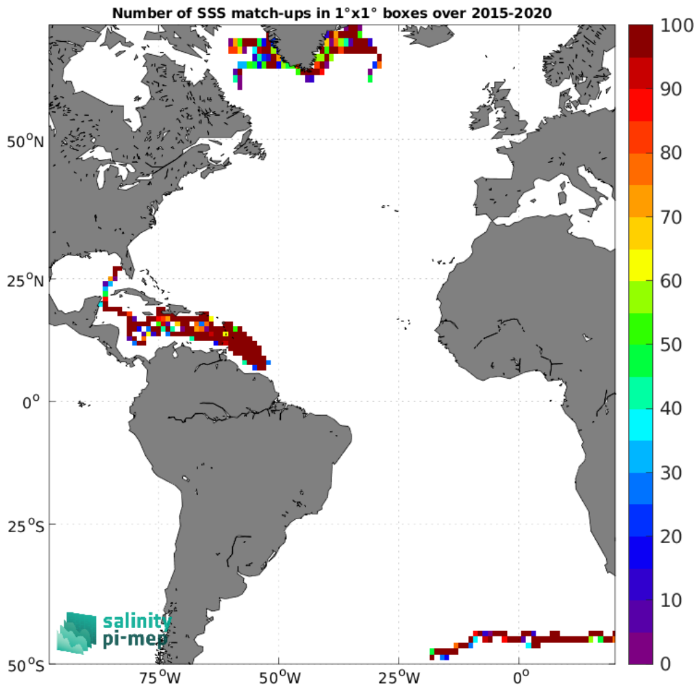
Figure 4: Number of SSS match-ups between Surface drifters SSS and the SMAP SSS L3 v5.0 - 8-Day running (JPL) SSS product for the Atlantic Ocean Pi-MEP region over 1°×1° boxes and for the full satellite product period.
