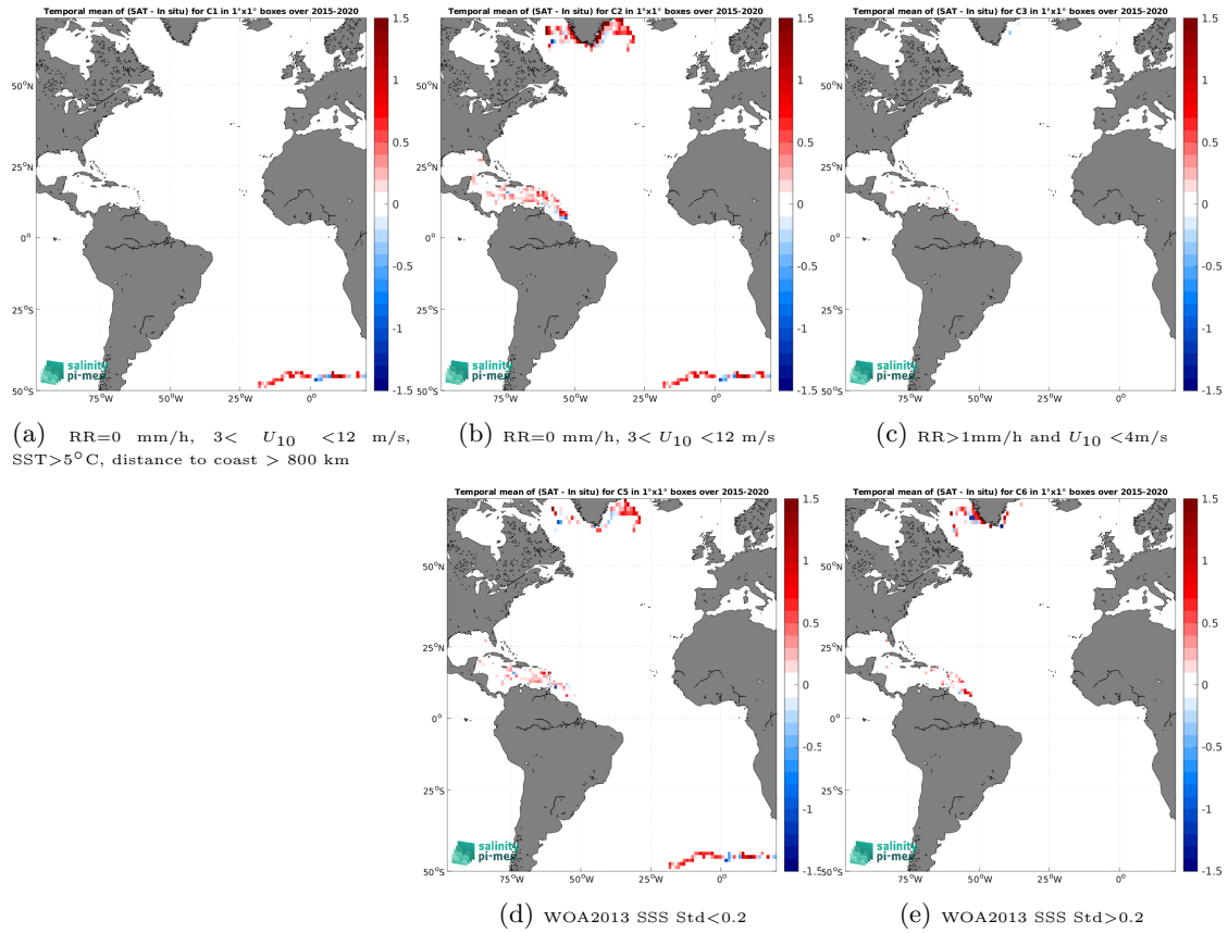
Figure 13: Temporal mean gridded over spatial boxes of size 1^\circ \times 1^\circ of \Delta\text{SSS} (SMAP SSS L3 v5.0 - 8-Day running (JPL) - Surface drifters) for 5 different subdatasets corresponding to:RR=0 mm/h, 3 < U_{10} < 12 m/s, SST >5^\circ\text{C} , distance to coast > 800 km (a), RR=0 mm/h, 3 < U_{10} < 12 m/s (b), RR >1 mm/h and U_{10} < 4 m/s (c), WOA2013 SSS Std <0.2 (d), WOA2013 SSS Std >0.2 (e).
