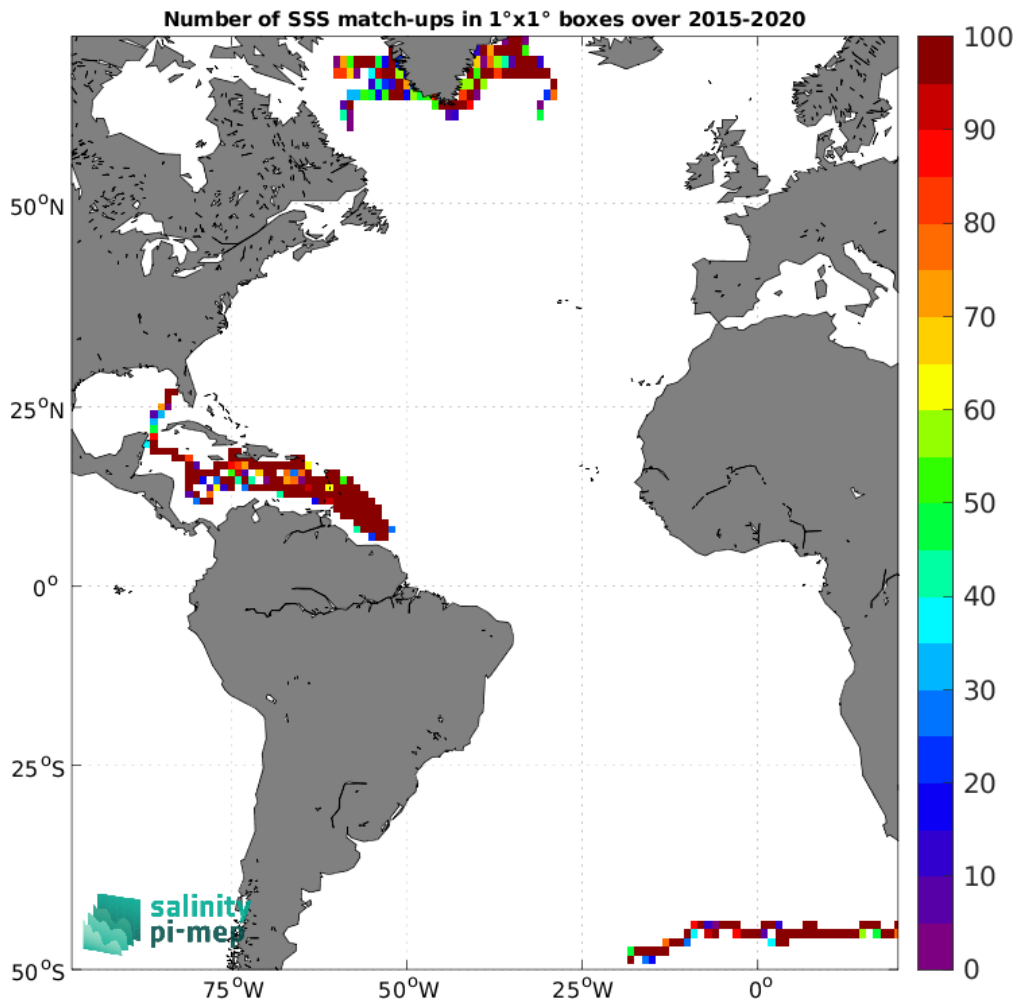
Figure 4: Number of SSS match-ups between Surface drifters SSS and the SMAP SSS L3 v5.0 - 8-Day running (JPL) SSS product for the Atlantic Ocean Pi-MEP region over 1^\circ \times 1^\circ boxes and for the full satellite product period.
