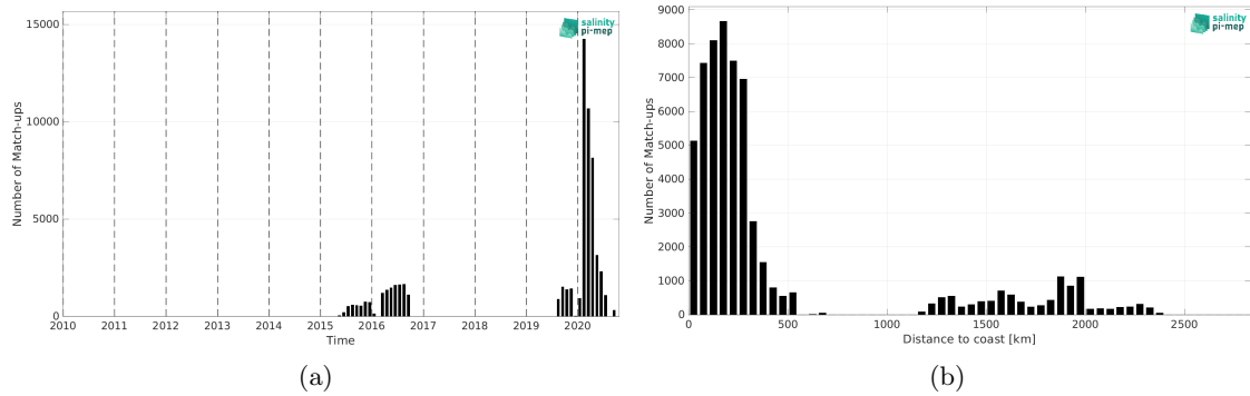
Figure 2: Number of match-ups between Surface drifters and SMAP SSS L3 v5.0 - 8-Day running (JPL) SSS as a function of time (a) and as function of the distance to coast (b) over the Atlantic Ocean Pi-MEP region and for the full satellite product period.
