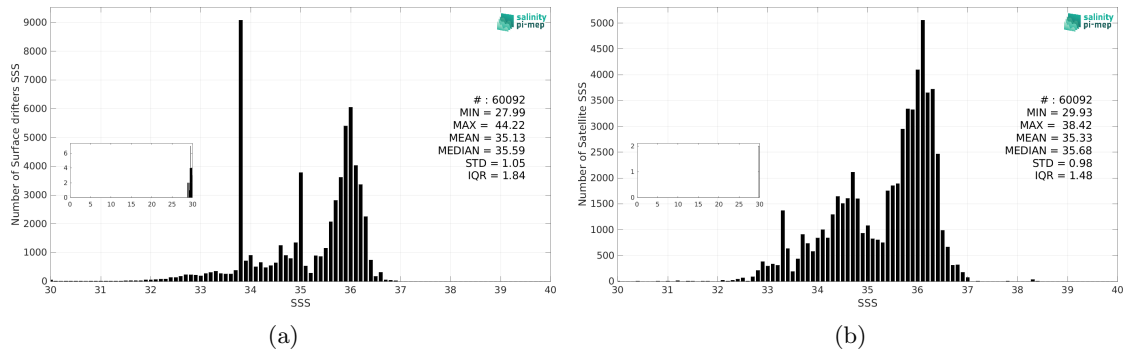
Figure 3: Histograms of SSS from Surface drifters (a) and SMAP SSS L3 v5.0 - 8-Day running (JPL) (b) considering all match-up pairs per bins of 0.1 over the Atlantic Ocean Pi-MEP region and for the full satellite product period.
