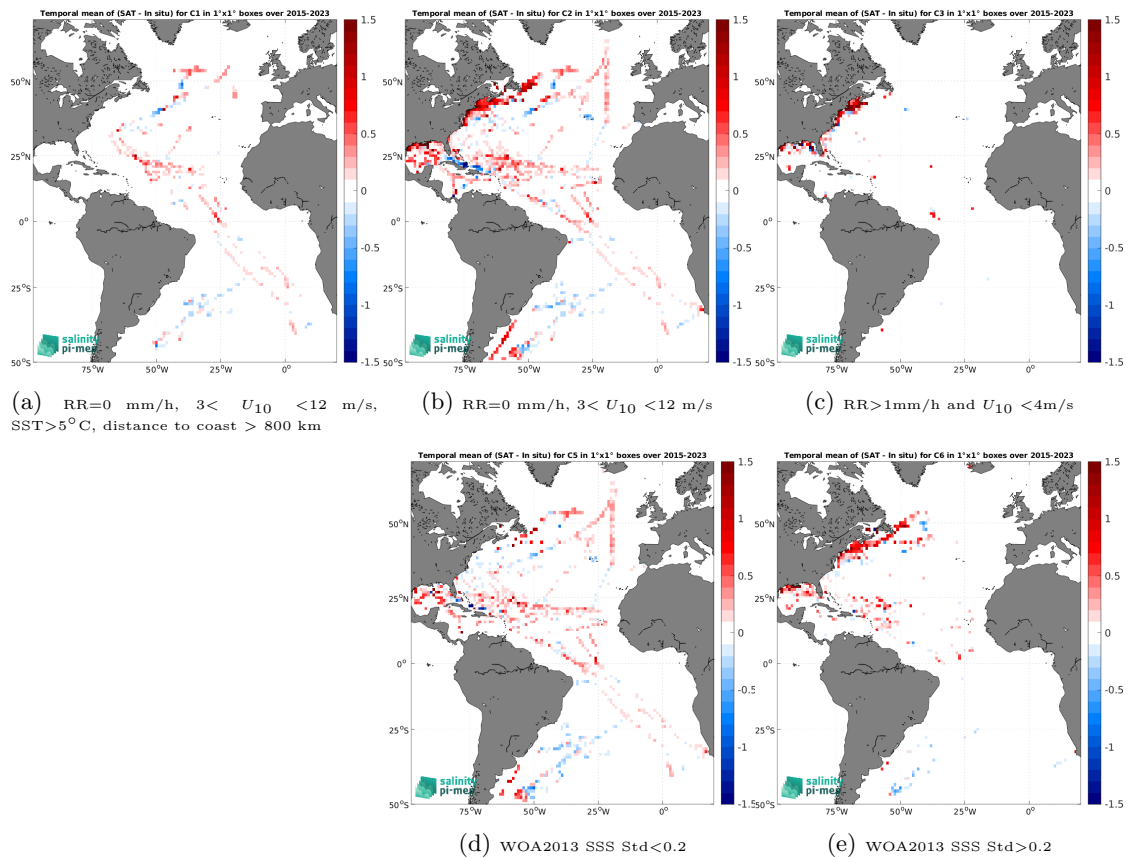
Figure 14: Temporal mean gridded over spatial boxes of size 1^\circ \times 1^\circ of \Delta\text{SSS} (SMAP SSS L3 v5.0 - Monthly (JPL) - TSG (SAMOS)) for 5 different subdatasets corresponding to:RR=0 mm/h, 3 < U_{10} < 12 m/s, SST >5^\circ\text{C} , distance to coast > 800 km (a), RR=0 mm/h, 3 < U_{10} < 12 m/s (b), RR >1 mm/h and U_{10} < 4 m/s (c), WOA2013 SSS Std <0.2 (d), WOA2013 SSS Std >0.2 (e).
