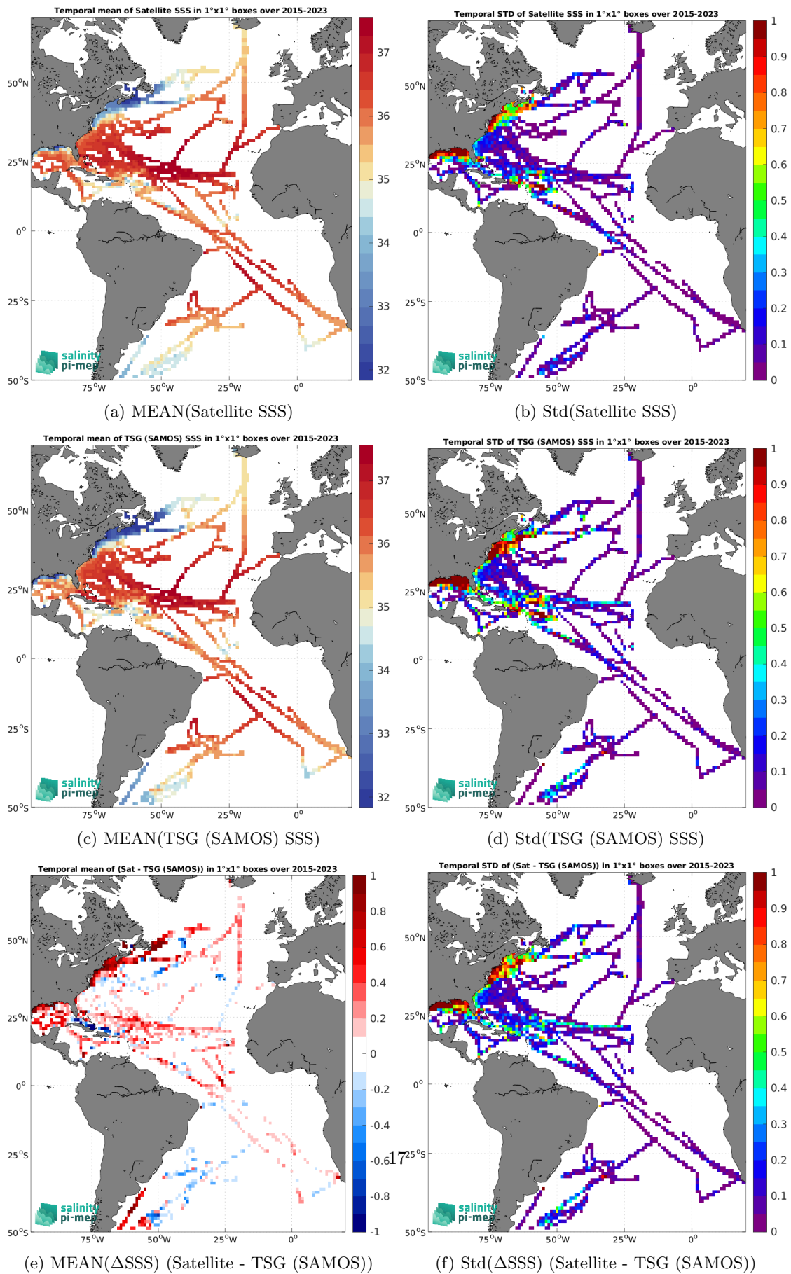
(e) MEAN( \Delta SSS) (Satellite - TSG (SAMOS)) (f) Std( \Delta SSS) (Satellite - TSG (SAMOS)) Figure 7: Temporal mean (left) and Std (right) of SSS from SMAP SSS L3 v5.0 - Monthly (JPL) (top), TSG (SAMOS) (middle), and of \Delta SSS (Satellite - TSG (SAMOS)). Only match-up pairs are used to generate these maps.
