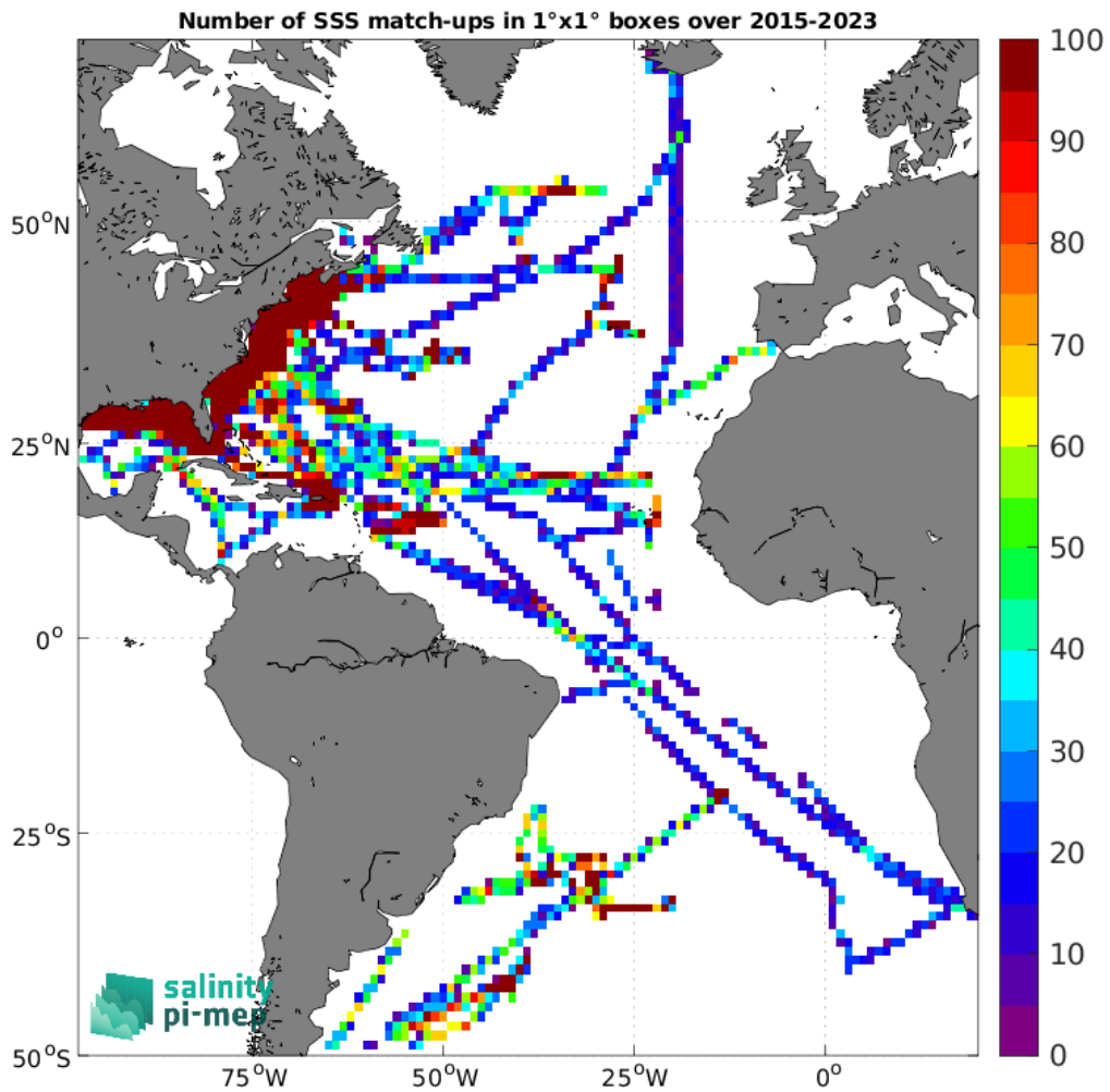
Figure 5: Number of SSS match-ups between TSG (SAMOS) SSS and the SMAP SSS L3 v5.0 - Monthly (JPL) SSS product for the Atlantic Ocean Pi-MEP region over 1^\circ \times 1^\circ boxes and for the full satellite product period.
