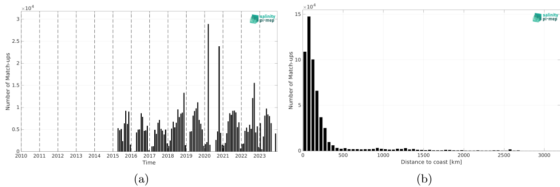
Figure 2: Number of match-ups between TSG (SAMOS) and SMAP SSS L3 v5.0 - Monthly (JPL) SSS as a function of time (a) and as function of the distance to coast (b) over the Atlantic Ocean Pi-MEP region and for the full satellite product period.
