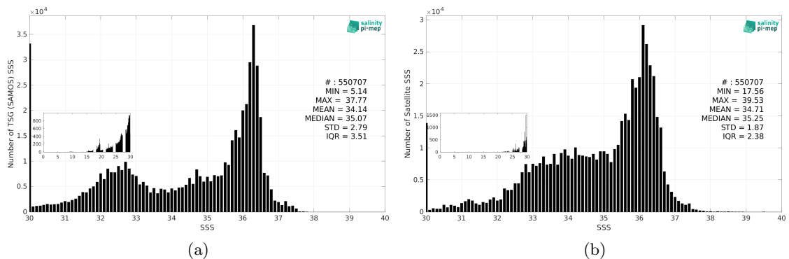
Figure 3: Histograms of SSS from TSG (SAMOS) (a) and SMAP SSS L3 v5.0 - Monthly (JPL) (b) considering all match-up pairs per bins of 0.1 over the Atlantic Ocean Pi-MEP region and for the full satellite product period.
