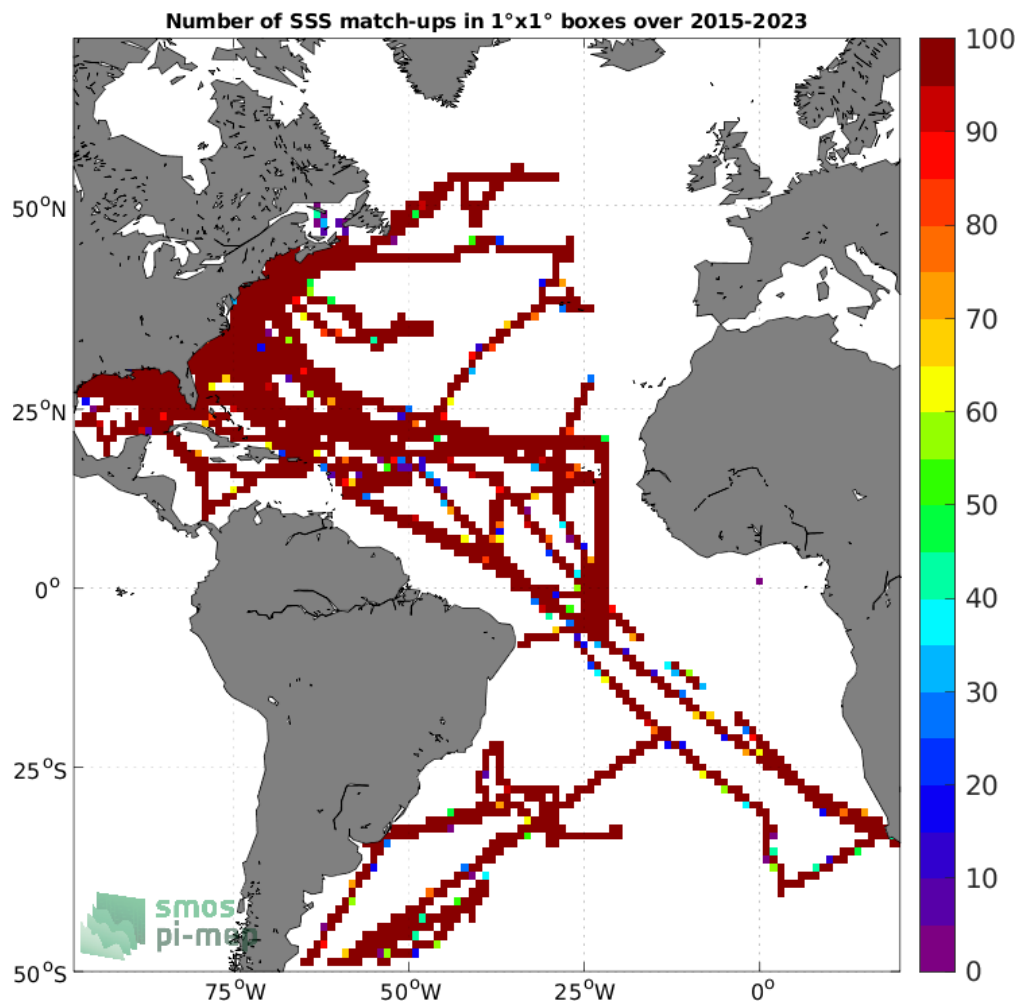
Figure 4: Number of SSS match-ups between TSG (SAMOS) SSS and the SMAP SSS L3 v5.0 - Monthly (JPL) SSS product for the Atlantic Ocean Pi-MEP region over 1°x1° boxes and for the full satellite product period.
