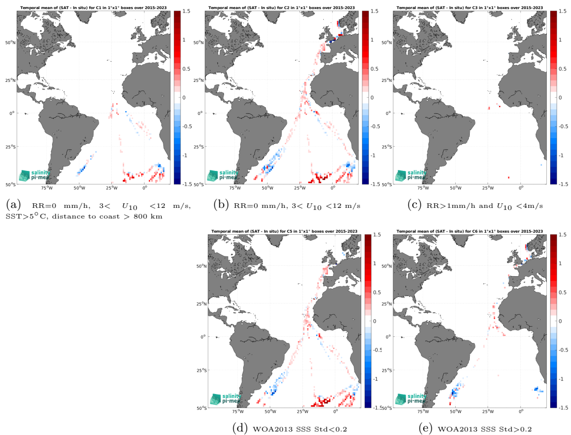
Figure 14: Temporal mean gridded over spatial boxes of size 1^\circ \times 1^\circ of \Delta SSS (SMAP SSS L3 v5.0 - Monthly (JPL) - TSG (Polarstern)) for 5 different subdatasets corresponding to:RR=0 mm/h, 3 < U_{10} < 12 m/s, SST >5^\circ\text{C} , distance to coast > 800 km (a), RR=0 mm/h, 3 < U_{10} < 12 m/s (b), RR >1 mm/h and U_{10} < 4 m/s (c), WOA2013 SSS Std <0.2 (d), WOA2013 SSS Std >0.2 (e).
