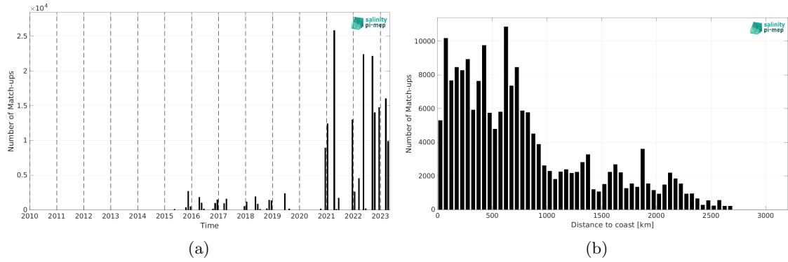
Figure 2: Number of match-ups between TSG (Polarstern) and SMAP SSS L3 v5.0 - Monthly (JPL) SSS as a function of time (a) and as function of the distance to coast (b) over the Atlantic Ocean Pi-MEP region and for the full satellite product period.
