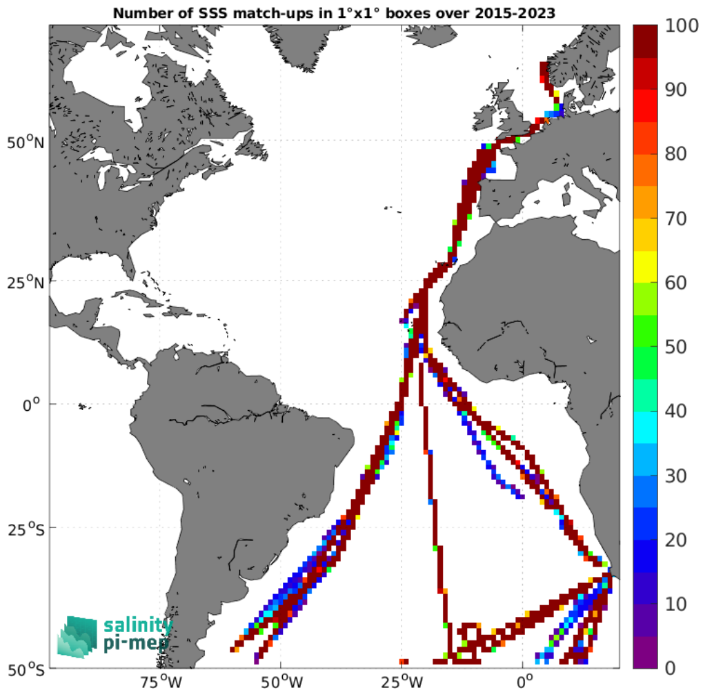
Figure 5: Number of SSS match-ups between TSG (Polarstern) SSS and the SMAP SSS L3 v5.0 - Monthly (JPL) SSS product for the Atlantic Ocean Pi-MEP region over 1^\circ \times 1^\circ boxes and for the full satellite product period.
