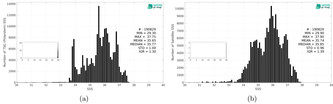
Figure 3: Histograms of SSS from TSG (Polarstern) (a) and SMAP SSS L3 v5.0 - Monthly (JPL) (b) considering all match-up pairs per bins of 0.1 over the Atlantic Ocean Pi-MEP region and for the full satellite product period.
