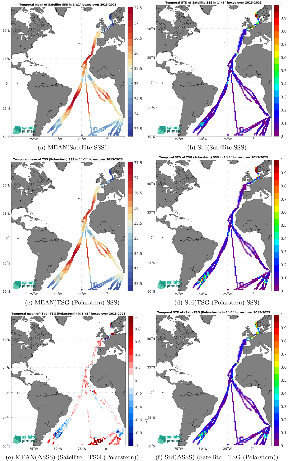
Figure 7: Temporal mean (left) and Std (right) of SSS from SMAP SSS L3 v5.0 - Monthly (JPL) (top), TSG (Polarstern) (middle), and of \Delta\text{SSS} (Satellite - TSG (Polarstern)). Only match-up pairs are used to generate these maps.
