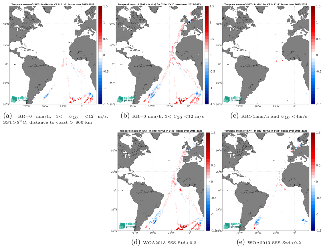
Figure 14: Temporal mean gridded over spatial boxes of size 1^\circ \times 1^\circ of \Delta\text{SSS} (SMAP SSS L3 v5.0 - Monthly (JPL) - TSG (Polarstern)) for 5 different subdatasets corresponding to:RR=0 mm/h, 3 < U_{10} < 12 m/s, SST >5^\circ\text{C} , distance to coast > 800 km (a), RR=0 mm/h, 3 < U_{10} < 12 m/s (b), RR >1 mm/h and U_{10} < 4 m/s (c), WOA2013 SSS Std <0.2 (d), WOA2013 SSS Std >0.2 (e).
