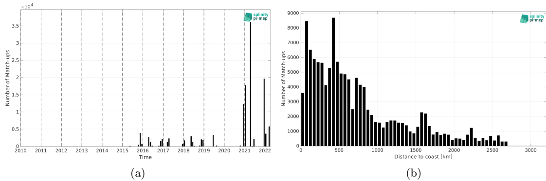
Figure 1: Number of match-ups between TSG (Polarstern) and SMAP SSS L3 v5.0 - Monthly (JPL) SSS as a function of time (a) and as function of the distance to coast (b) over the Atlantic Ocean Pi-MEP region and for the full satellite product period.
