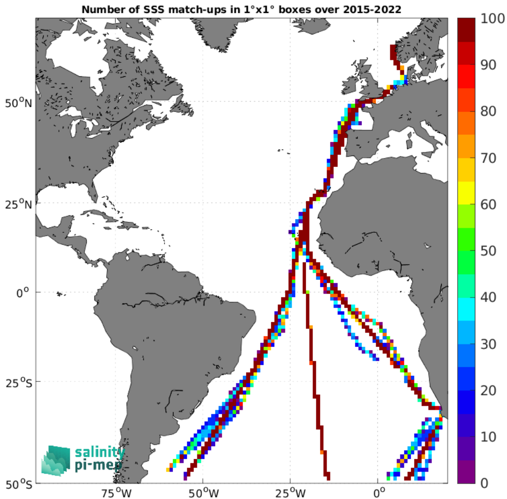
Figure 4: Number of SSS match-ups between TSG (Polarstern) SSS and the SMAP SSS L3 v5.0 - Monthly (JPL) SSS product for the Atlantic Ocean Pi-MEP region over 1°×1° boxes and for the full satellite product period.
