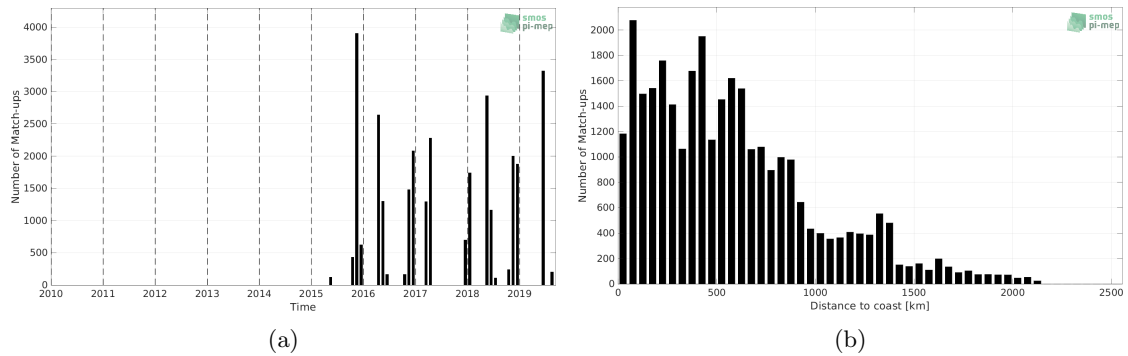
Figure 1: Number of match-ups between TSG (Polarstern) and SMAP SSS L3 v5.0 - Monthly (JPL) SSS as a function of time (a) and as function of the distance to coast (b) over the Atlantic Ocean Pi-MEP region and for the full satellite product period.
