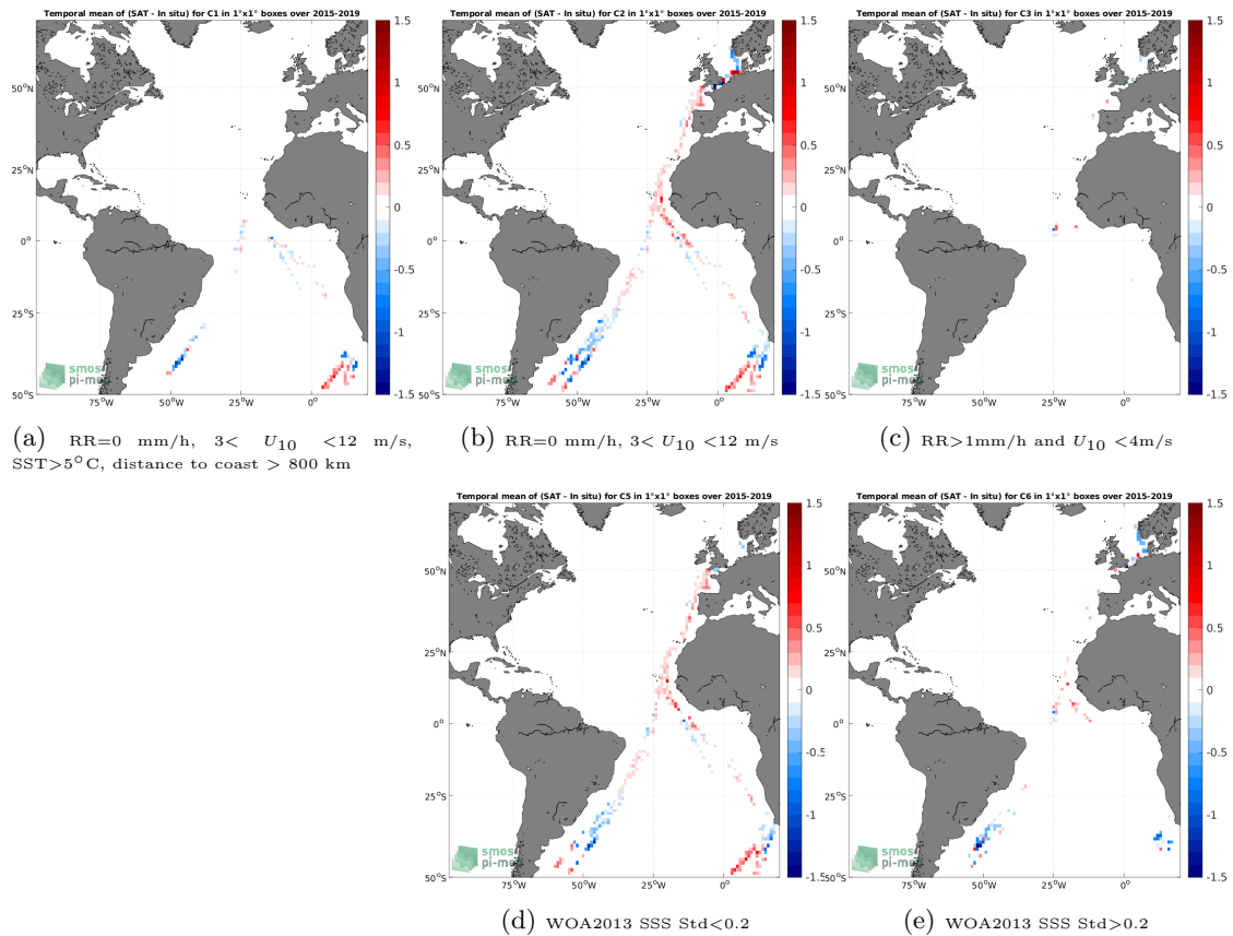
Figure 12: Temporal mean gridded over spatial boxes of size 1^\circ \times 1^\circ of \Delta SSS (SMAP SSS L3 v5.0 - Monthly (JPL) - TSG (Polarstern)) for 5 different subdatasets corresponding to:RR=0 mm/h, 3 < U_{10} < 12 m/s, SST >5^\circ\text{C} , distance to coast > 800 km (a), RR=0 mm/h, 3 < U_{10} < 12 m/s (b), RR >1 mm/h and U_{10} < 4 m/s (c), WOA2013 SSS Std <0.2 (d), WOA2013 SSS Std >0.2 (e).
