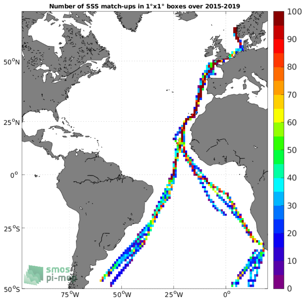
Figure 4: Number of SSS match-ups between TSG (Polarstern) SSS and the SMAP SSS L3 v5.0 - Monthly (JPL) SSS product for the Atlantic Ocean Pi-MEP region over 1°x1° boxes and for the full satellite product period.
