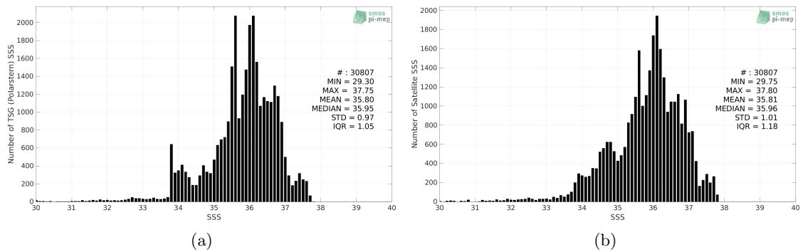
Figure 2: Histograms of SSS from TSG (Polarstern) (a) and SMAP SSS L3 v5.0 - Monthly (JPL) (b) considering all match-up pairs per bins of 0.1 over the Atlantic Ocean Pi-MEP region and for the full satellite product period.
