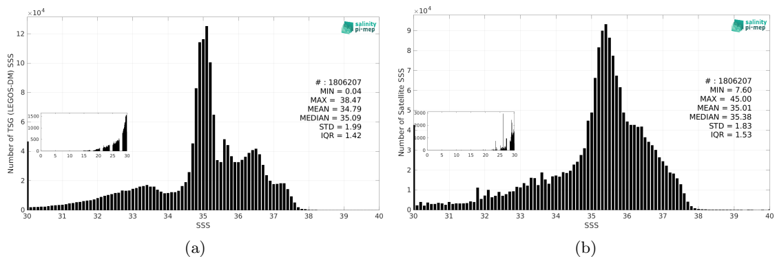
Figure 3: Histograms of SSS from TSG (LEGOS-DM) (a) and SMAP SSS L3 v5.0 - Monthly (JPL) (b) considering all match-up pairs per bins of 0.1 over the Atlantic Ocean Pi-MEP region and for the full satellite product period.
