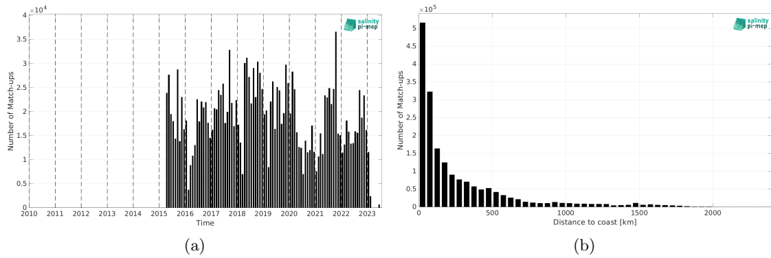
Figure 2: Number of match-ups between TSG (LEGOS-DM) and SMAP SSS L3 v5.0 - Monthly (JPL) SSS as a function of time (a) and as function of the distance to coast (b) over the Atlantic Ocean Pi-MEP region and for the full satellite product period.
