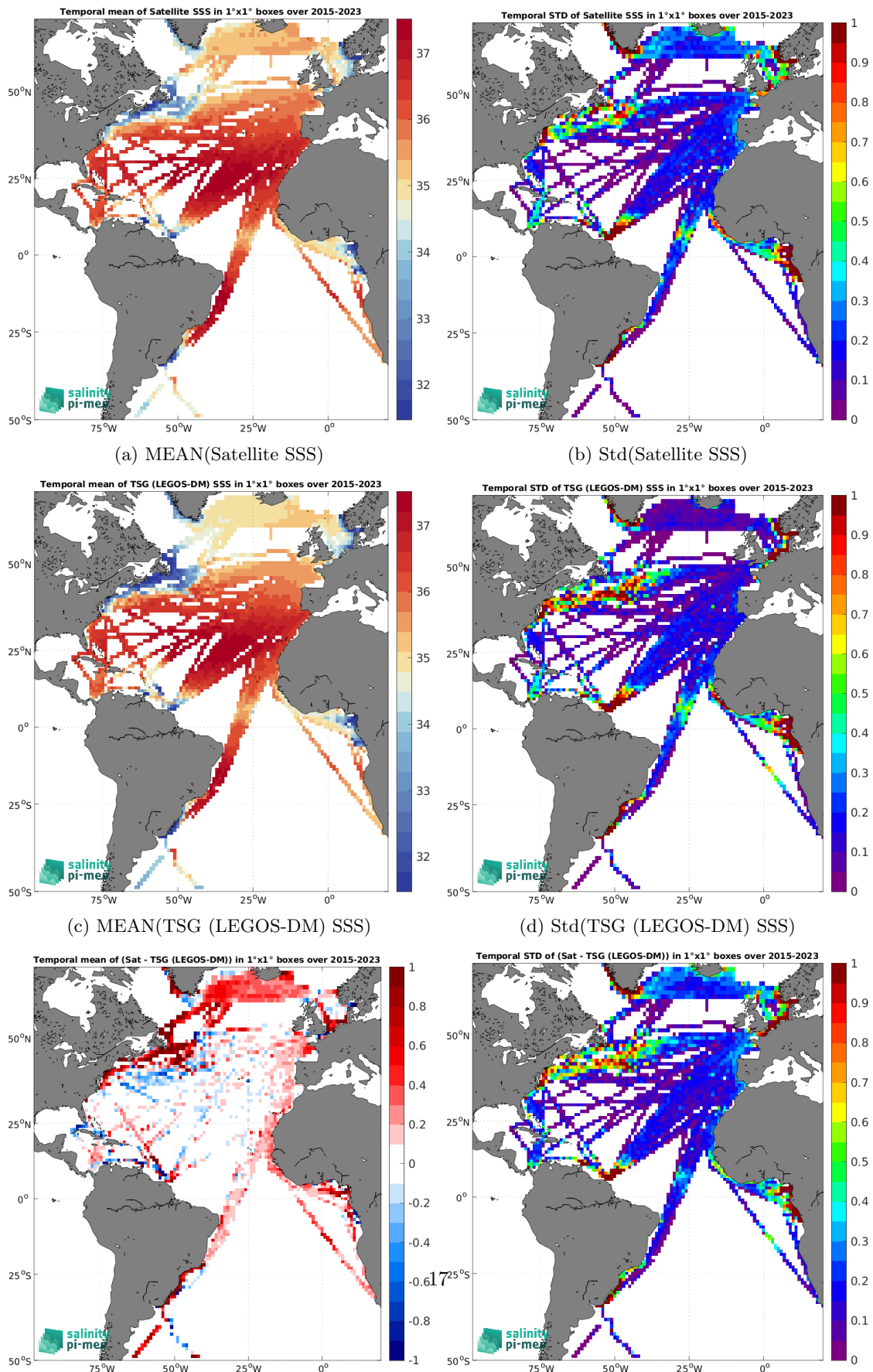
Figure 7: Temporal mean (left) and Std (right) of SSS from SMAP SSS L3 v5.0 - Monthly (JPL) (top), TSG (LEGOS-DM) (middle), and of \Delta SSS (Satellite - TSG (LEGOS-DM)). Only match-up pairs are used to generate these maps.
