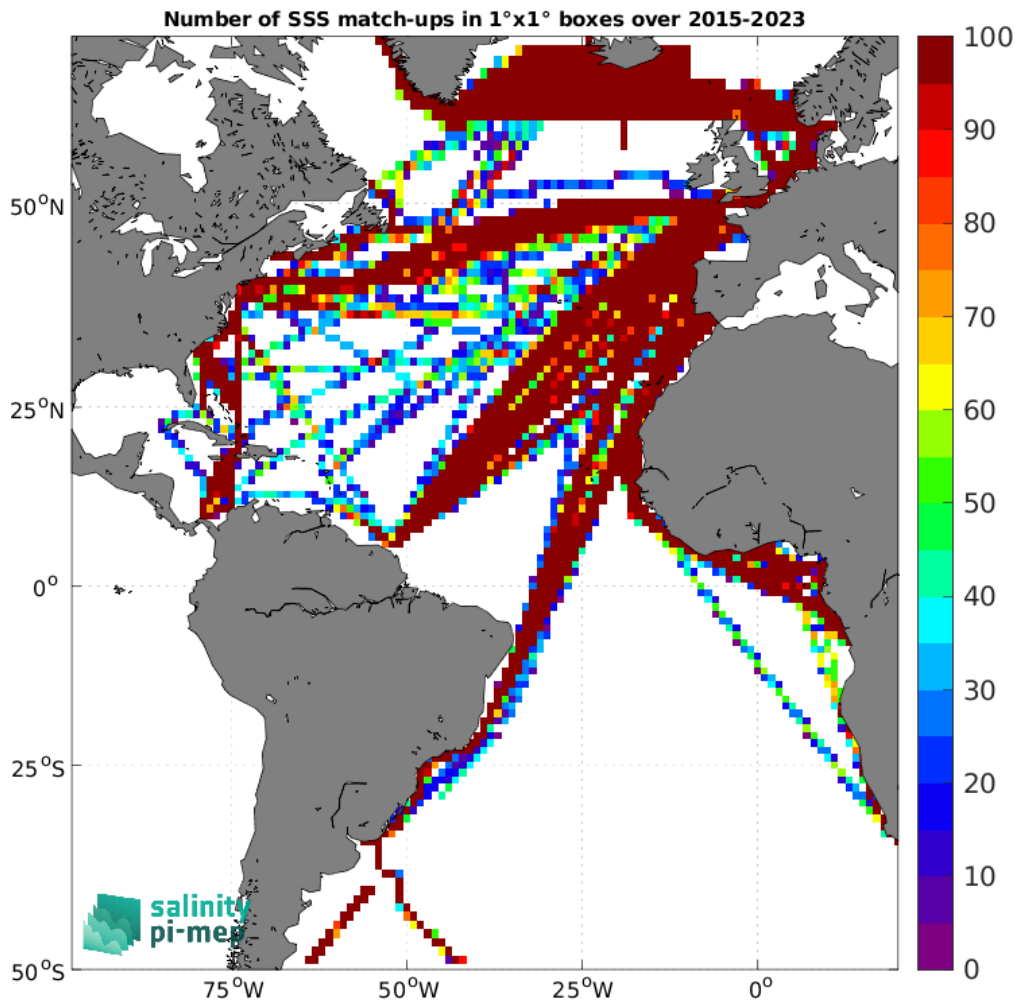
Figure 5: Number of SSS match-ups between TSG (LEGOS-DM) SSS and the SMAP SSS L3 v5.0 - Monthly (JPL) SSS product for the Atlantic Ocean Pi-MEP region over 1^\circ \times 1^\circ boxes and for the full satellite product period.
