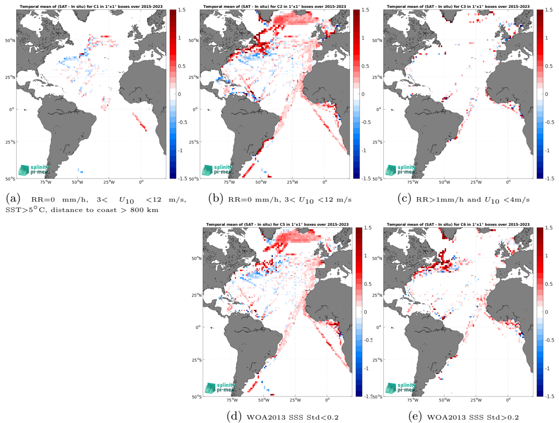
Figure 14: Temporal mean gridded over spatial boxes of size 1^\circ \times 1^\circ of \Delta\text{SSS} (SMAP SSS L3 v5.0 - Monthly (JPL) - TSG (LEGOS-DM)) for 5 different subdatasets corresponding to:RR=0 mm/h, 3 < U_{10} < 12 m/s, SST>5°C, distance to coast > 800 km (a), RR=0 mm/h, 3 < U_{10} < 12 m/s (b), RR>1mm/h and U_{10} < 4 m/s (c), WOA2013 SSS Std<0.2 (d), WOA2013 SSS Std>0.2 (e).
