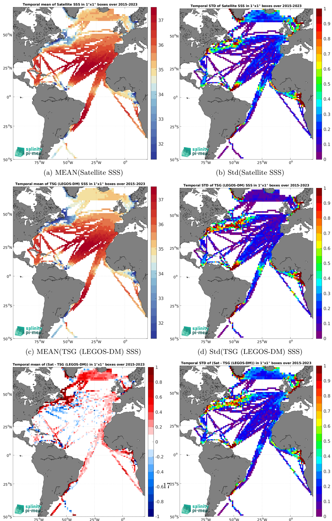
(e) MEAN( \Delta SSS) (Satellite - TSG (LEGOS-DM)) (f) Std( \Delta SSS) (Satellite - TSG (LEGOS-DM)) Figure 6: Temporal mean (left) and Std (right) of SSS from SMAP SSS L3 v5.0 - Monthly (JPL) (top), TSG (LEGOS-DM) (middle), and of \Delta SSS (Satellite - TSG (LEGOS-DM)). Only match-up pairs are used to generate these maps.
