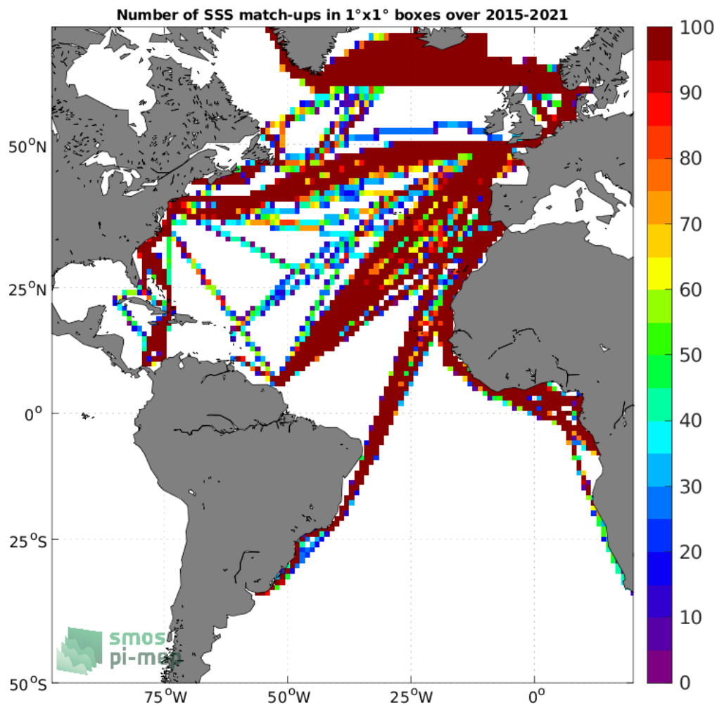
Figure 4: Number of SSS match-ups between TSG (LEGOS-DM) SSS and the SMAP SSS L3 v5.0 - Monthly (JPL) SSS product for the Atlantic Ocean Pi-MEP region over 1°x1° boxes and for the full satellite product period.
