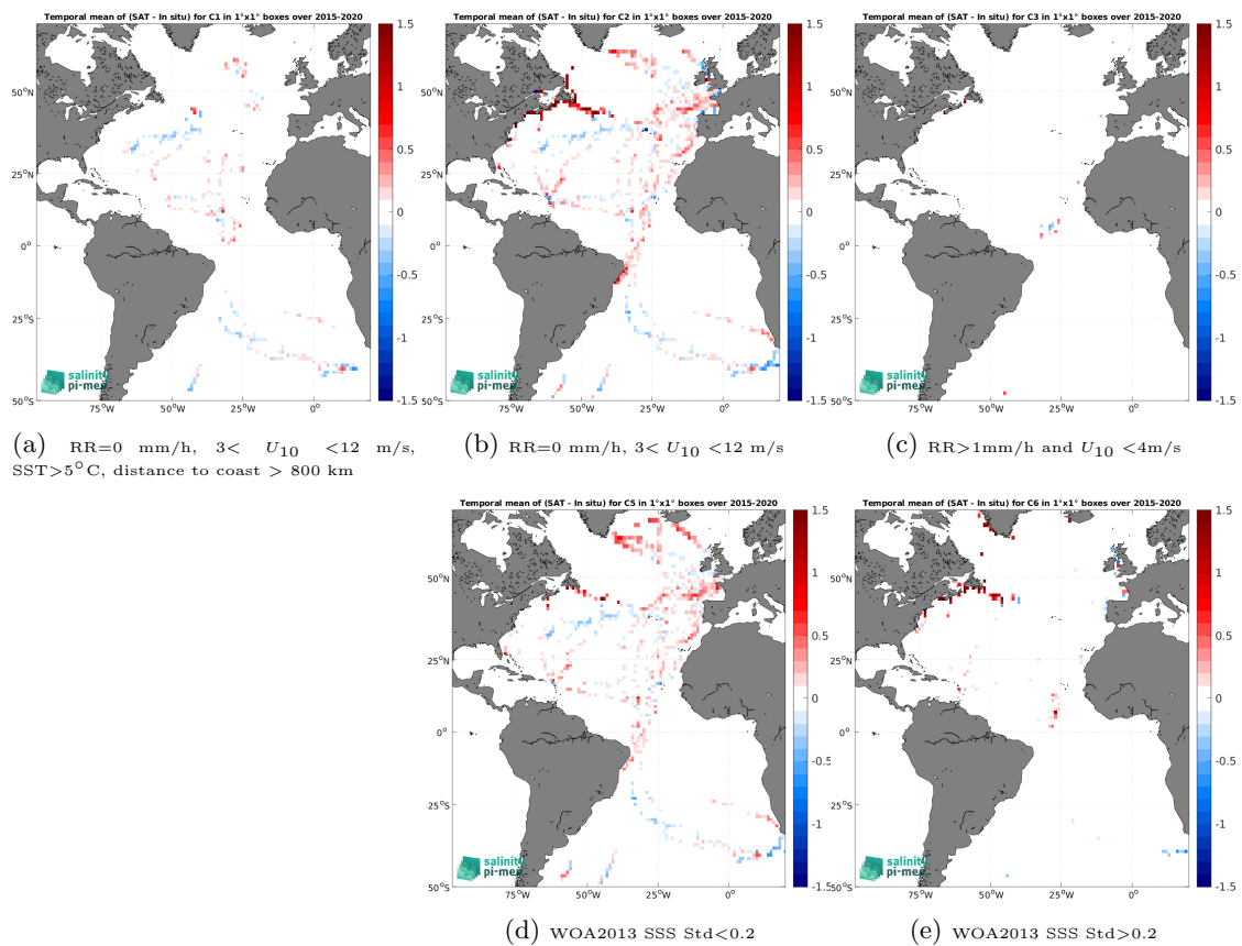
Figure 12: Temporal mean gridded over spatial boxes of size 1^\circ \times 1^\circ of \Delta SSS (SMAP SSS L3 v5.0 - Monthly (JPL) - TSG (GOSUD-Sailing-ship)) for 5 different subdatasets corresponding to:RR=0 mm/h, 3 < U_{10} < 12 m/s, SST >5^\circ\text{C} , distance to coast > 800 km (a), RR=0 mm/h, 3 < U_{10} < 12 m/s (b), RR >1 mm/h and U_{10} < 4 m/s (c), WOA2013 SSS Std <0.2 (d), WOA2013 SSS Std >0.2 (e).
