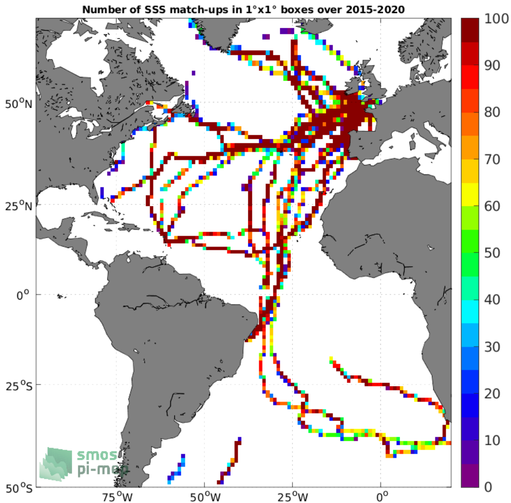
Figure 4: Number of SSS match-ups between TSG (GOSUD-Sailing-ship) SSS and the SMAP SSS L3 v5.0 - Monthly (JPL) SSS product for the Atlantic Ocean Pi-MEP region over 1°x1° boxes and for the full satellite product period.
