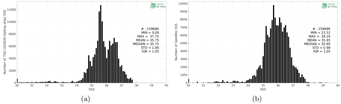
Figure 2: Histograms of SSS from TSG (GOSUD-Sailing-ship) (a) and SMAP SSS L3 v5.0 - Monthly (JPL) (b) considering all match-up pairs per bins of 0.1 over the Atlantic Ocean Pi-MEP region and for the full satellite product period.
