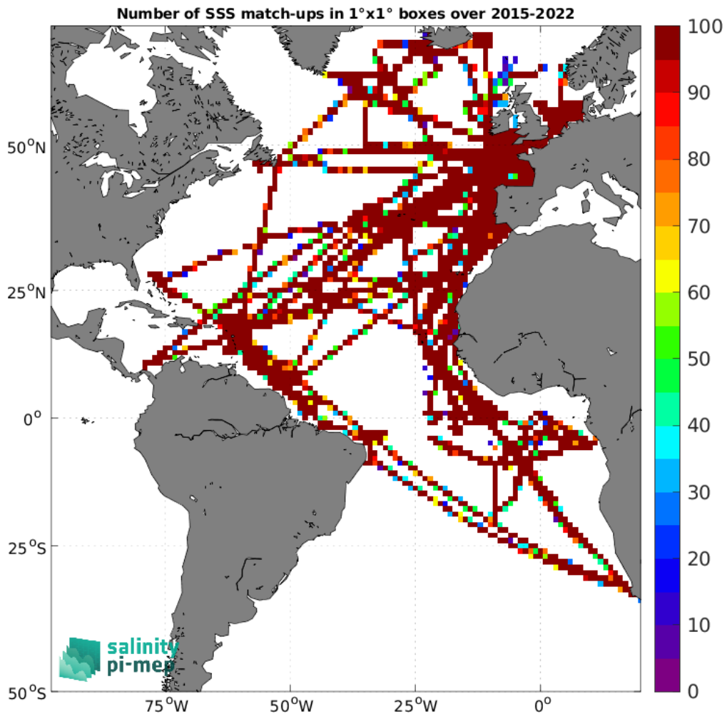
Figure 5: Number of SSS match-ups between TSG (GOSUD-Research-vessel) SSS and the SMAP SSS L3 v5.0 - Monthly (JPL) SSS product for the Atlantic Ocean Pi-MEP region over 1°x1° boxes and for the full satellite product period.
