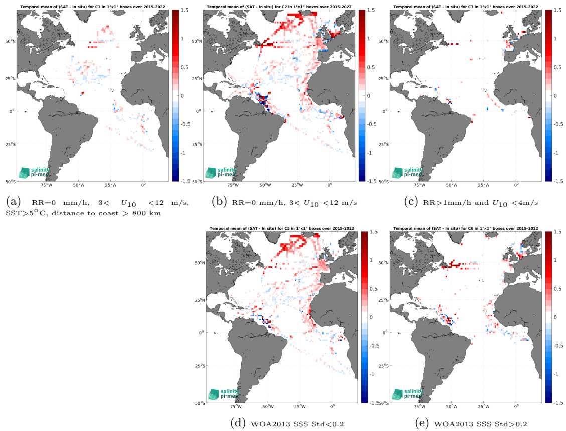
Figure 14: Temporal mean gridded over spatial boxes of size 1^\circ \times 1^\circ of \Delta\text{SSS} (SMAP SSS L3 v5.0 - Monthly (JPL) - TSG (GOSUD-Research-vessel)) for 5 different subdatasets corresponding to:RR=0 mm/h, 3 < U_{10} < 12 m/s, SST>5°C, distance to coast > 800 km (a), RR=0 mm/h, 3 < U_{10} < 12 m/s (b), RR>1mm/h and U_{10} < 4 m/s (c), WOA2013 SSS Std<0.2 (d), WOA2013 SSS Std>0.2 (e).
