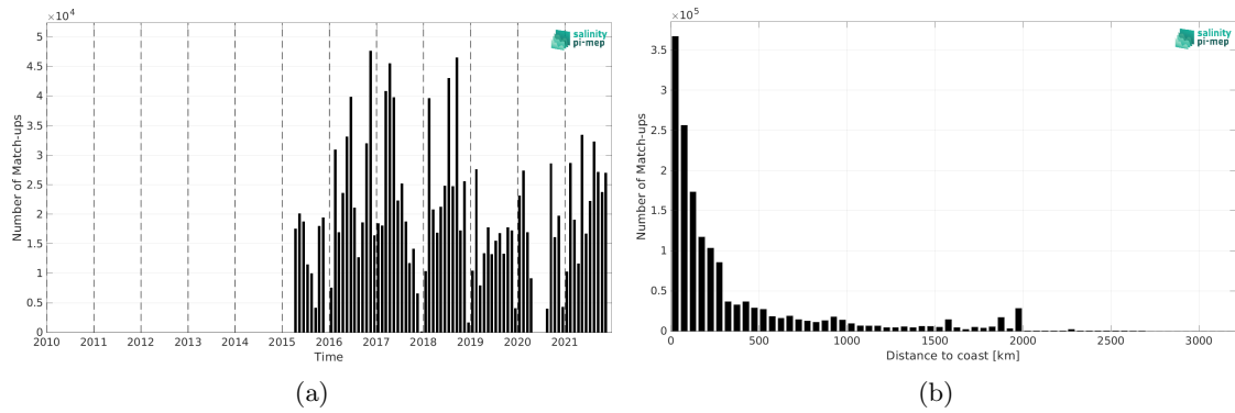
Figure 2: Number of match-ups between TSG (GOSUD-Research-vessel) and SMAP SSS L3 v5.0 - Monthly (JPL) SSS as a function of time (a) and as function of the distance to coast (b) over the Atlantic Ocean Pi-MEP region and for the full satellite product period.
