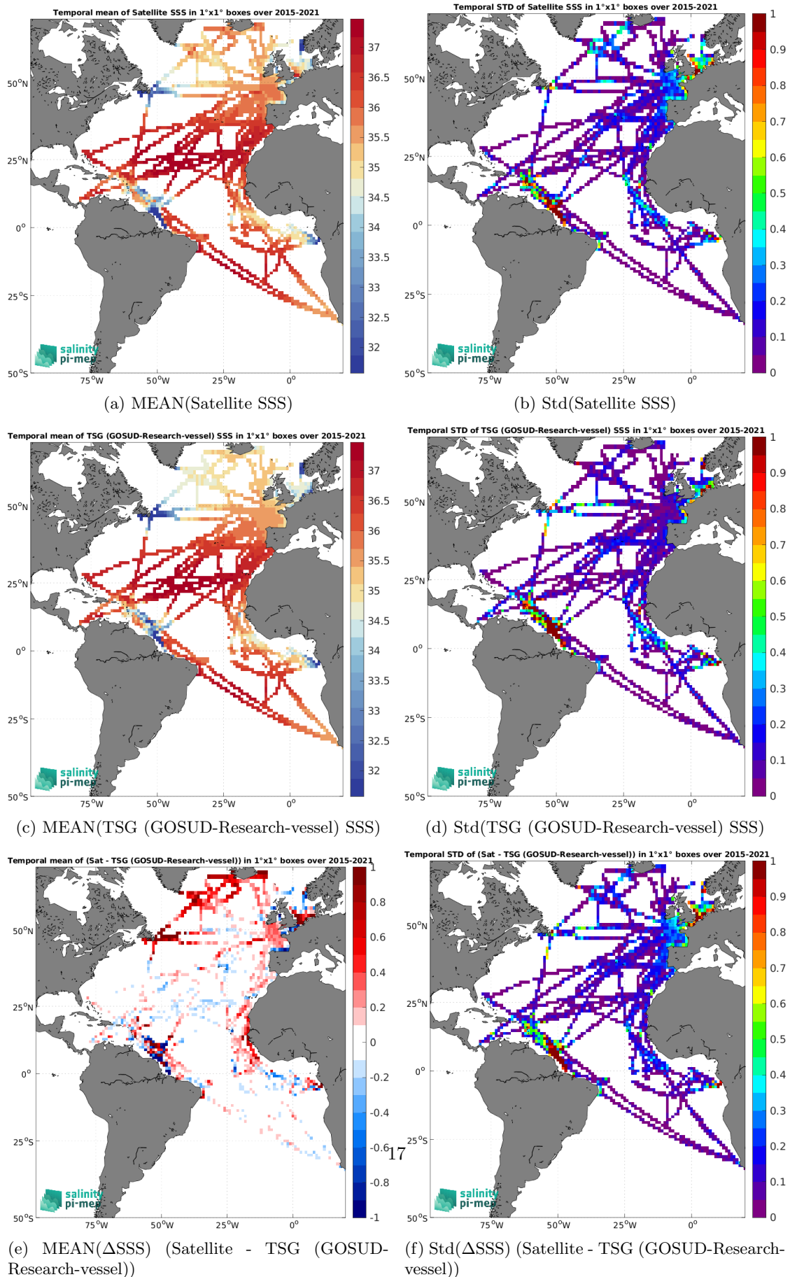
Figure 7: Temporal mean (left) and Std (right) of SSS from SMAP SSS L3 v5.0 - Monthly (JPL) (top), TSG (GOSUD-Research-vessel) (middle), and of \Delta SSS (Satellite - TSG (GOSUD-Research-vessel)). Only match-up pairs are used to generate these maps.
