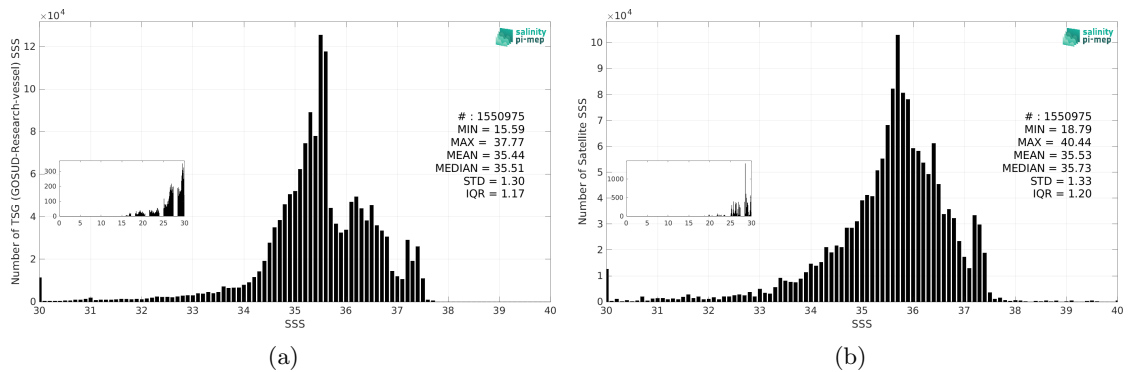
Figure 3: Histograms of SSS from TSG (GOSUD-Research-vessel) (a) and SMAP SSS L3 v5.0 - Monthly (JPL) (b) considering all match-up pairs per bins of 0.1 over the Atlantic Ocean Pi-MEP region and for the full satellite product period.
