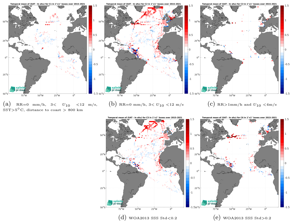
Figure 14: Temporal mean gridded over spatial boxes of size 1^\circ \times 1^\circ of \Delta SSS (SMAP SSS L3 v5.0 - Monthly (JPL) - TSG (GOSUD-Research-vessel)) for 5 different subdatasets corresponding to:RR=0 mm/h, 3 < U_{10} < 12 m/s, SST >5^\circ\text{C} , distance to coast > 800 km (a), RR=0 mm/h, 3 < U_{10} < 12 m/s (b), RR >1 mm/h and U_{10} < 4 m/s (c), WOA2013 SSS Std <0.2 (d), WOA2013 SSS Std >0.2 (e).
