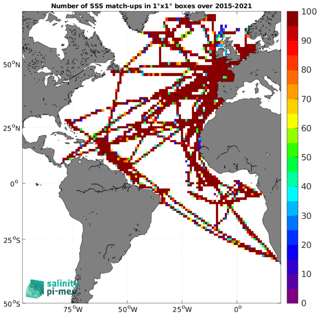
Figure 5: Number of SSS match-ups between TSG (GOSUD-Research-vessel) SSS and the SMAP SSS L3 v5.0 - Monthly (JPL) SSS product for the Atlantic Ocean Pi-MEP region over 1^\circ \times 1^\circ boxes and for the full satellite product period.
