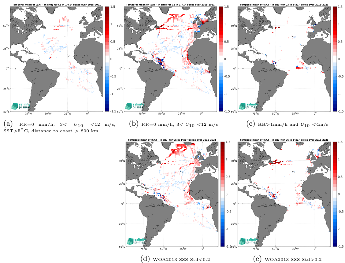
Figure 12: Temporal mean gridded over spatial boxes of size 1^\circ \times 1^\circ of \Delta\text{SSS} (SMAP SSS L3 v5.0 - Monthly (JPL) - TSG (GOSUD-Research-vessel)) for 5 different subdatasets corresponding to:RR=0 mm/h, 3 < U_{10} < 12 m/s, SST >5^\circ\text{C} , distance to coast > 800 km (a), RR=0 mm/h, 3 < U_{10} < 12 m/s (b), RR >1 mm/h and U_{10} < 4 m/s (c), WOA2013 SSS Std <0.2 (d), WOA2013 SSS Std >0.2 (e).
