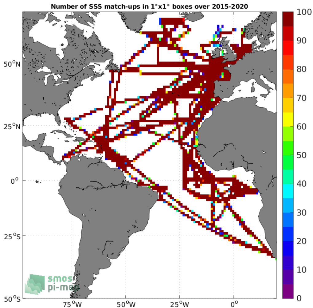
Figure 4: Number of SSS match-ups between TSG (GOSUD-Research-vessel) SSS and the SMAP SSS L3 v5.0 - Monthly (JPL) SSS product for the Atlantic Ocean Pi-MEP region over 1^\circ \times 1^\circ boxes and for the full satellite product period.
