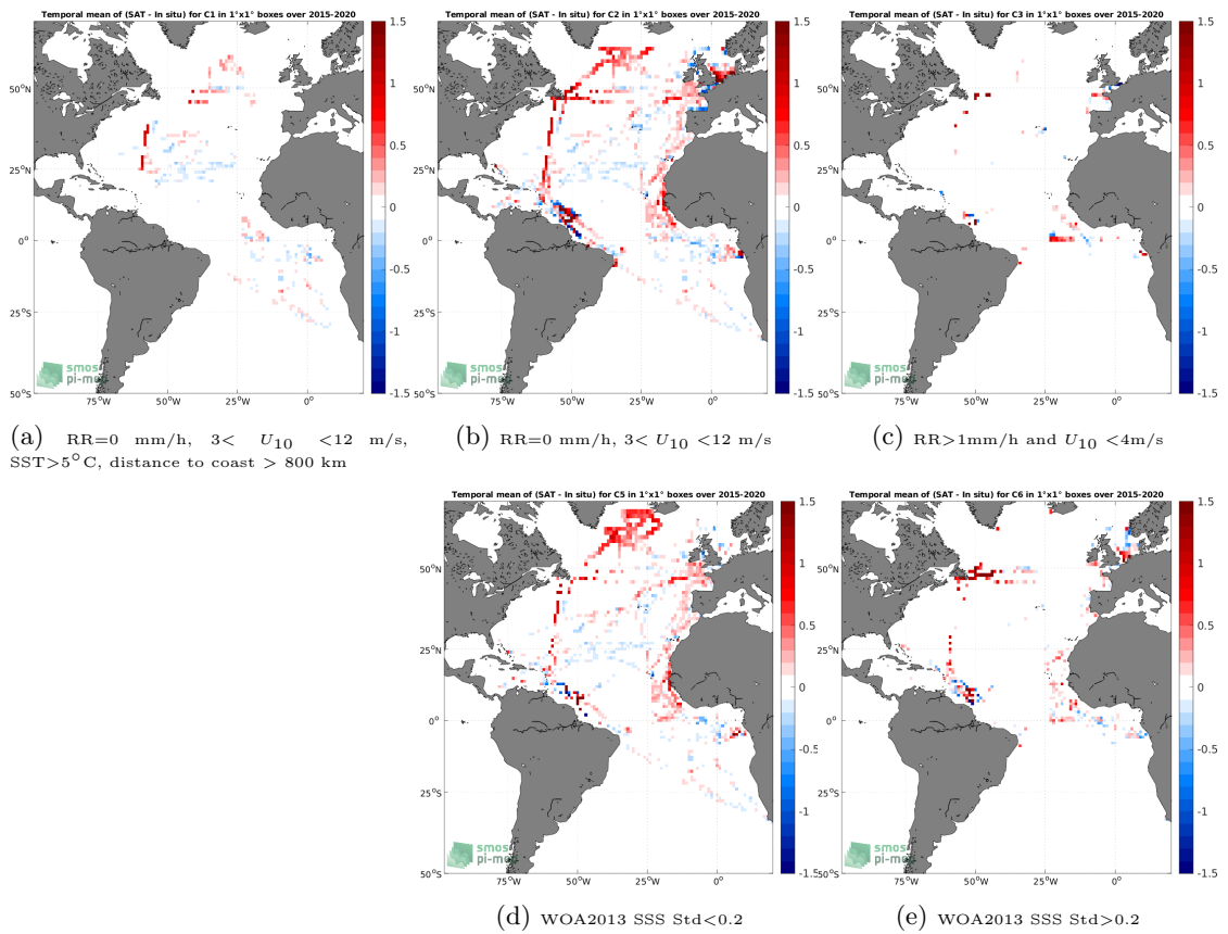
Figure 12: Temporal mean gridded over spatial boxes of size 1^\circ \times 1^\circ of \Delta SSS (SMAP SSS L3 v5.0 - Monthly (JPL) - TSG (GOSUD-Research-vessel)) for 5 different subdatasets corresponding to:RR=0 mm/h, 3 < U_{10} < 12 m/s, SST>5°C, distance to coast > 800 km (a), RR=0 mm/h, 3 < U_{10} < 12 m/s (b), RR>1mm/h and U_{10} < 4 m/s (c), WOA2013 SSS Std<0.2 (d), WOA2013 SSS Std>0.2 (e).
