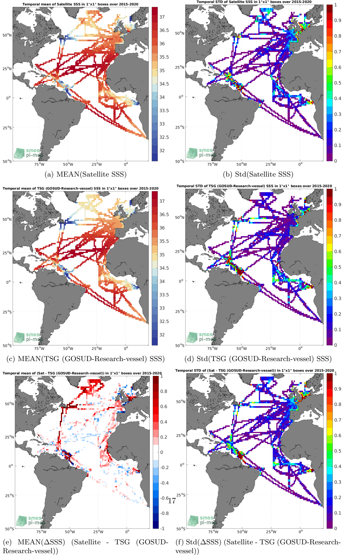
Figure 6: Temporal mean (left) and Std (right) of SSS from SMAP SSS L3 v5.0 - Monthly (JPL) (top), TSG (GOSUD-Research-vessel) (middle), and of \Delta SSS (Satellite - TSG (GOSUD-Research-vessel)). Only match-up pairs are used to generate these maps.
