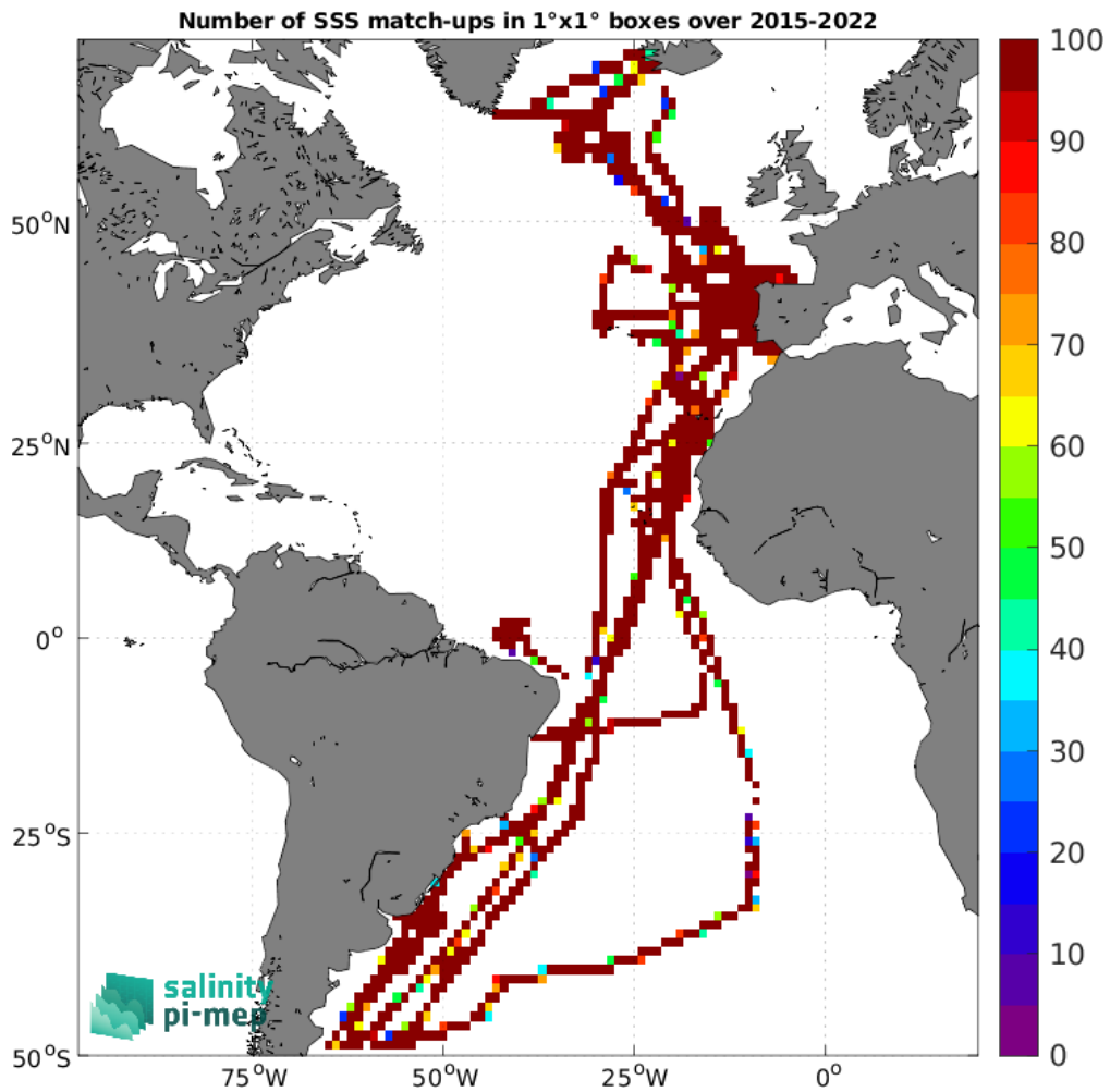
Figure 5: Number of SSS match-ups between TSG (CSIC-UTM) SSS and the SMAP SSS L3 v5.0 - Monthly (JPL) SSS product for the Atlantic Ocean Pi-MEP region over 1°×1° boxes and for the full satellite product period.
