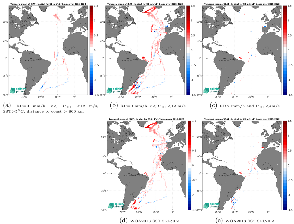
Figure 14: Temporal mean gridded over spatial boxes of size 1^\circ \times 1^\circ of \Delta\text{SSS} (SMAP SSS L3 v5.0 - Monthly (JPL) - TSG (CSIC-UTM)) for 5 different subdatasets corresponding to:RR=0 mm/h, 3 < U_{10} < 12 m/s, SST>5°C, distance to coast > 800 km (a), RR=0 mm/h, 3 < U_{10} < 12 m/s (b), RR>1mm/h and U_{10} < 4 m/s (c), WOA2013 SSS Std<0.2 (d), WOA2013 SSS Std>0.2 (e).
