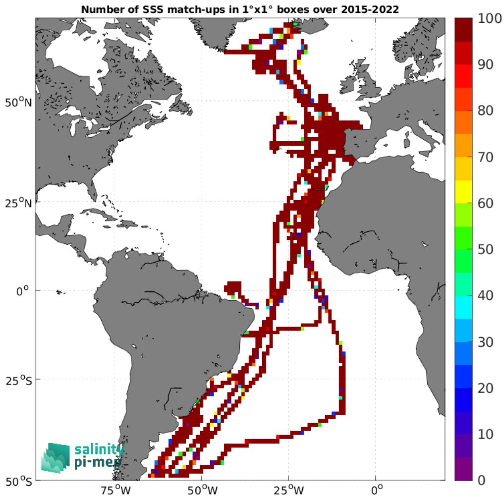
Figure 4: Number of SSS match-ups between TSG (CSIC-UTM) SSS and the SMAP SSS L3 v5.0 - Monthly (JPL) SSS product for the Atlantic Ocean Pi-MEP region over 1^{\circ} \times 1^{\circ} boxes and for the full satellite product period.
