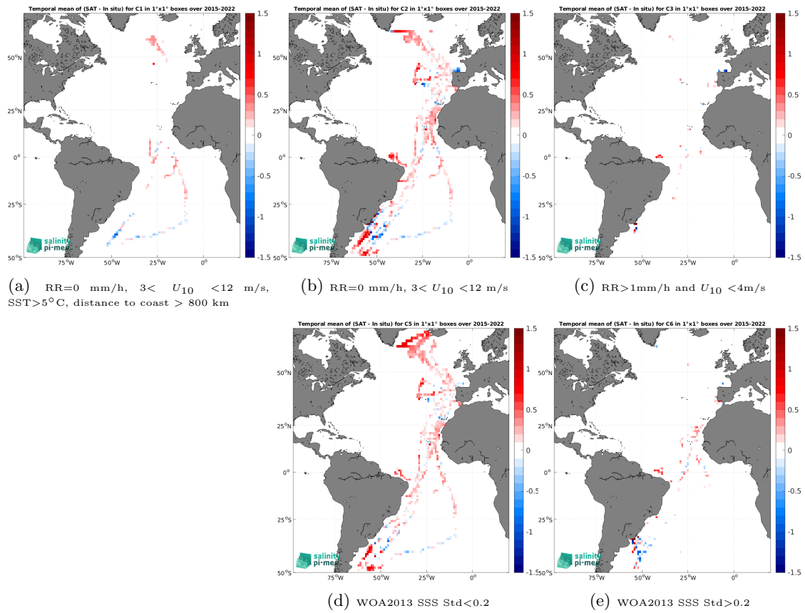
Figure 12: Temporal mean gridded over spatial boxes of size 1^\circ \times 1^\circ of \Delta\text{SSS} (SMAP SSS L3 v5.0 - Monthly (JPL) - TSG (CSIC-UTM)) for 5 different subdatasets corresponding to:RR=0 mm/h, 3 < U_{10} < 12 m/s, SST >5^\circ\text{C} , distance to coast > 800 km (a), RR=0 mm/h, 3 < U_{10} < 12 m/s (b), RR >1 mm/h and U_{10} < 4 m/s (c), WOA2013 SSS Std <0.2 (d), WOA2013 SSS Std >0.2 (e).
