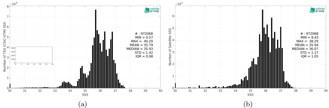
Figure 2: Histograms of SSS from TSG (CSIC-UTM) (a) and SMAP SSS L3 v5.0 - Monthly (JPL) (b) considering all match-up pairs per bins of 0.1 over the Atlantic Ocean Pi-MEP region and for the full satellite product period.
