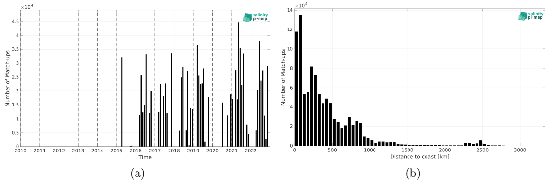
Figure 1: Number of match-ups between TSG (CSIC-UTM) and SMAP SSS L3 v5.0 - Monthly (JPL) SSS as a function of time (a) and as function of the distance to coast (b) over the Atlantic Ocean Pi-MEP region and for the full satellite product period.
