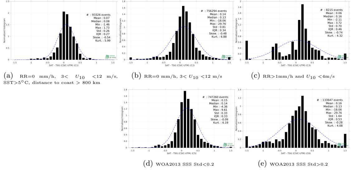
Figure 13: Normalized histogram of \Delta SSS (SMAP SSS L3 v5.0 - Monthly (JPL) - TSG (CSIC-UTM)) for 5 different subdatasets corresponding to: RR=0 mm/h, 3 < U_{10} < 12 m/s, SST>5°C, distance to coast > 800 km (a), RR=0 mm/h, 3 < U_{10} < 12 m/s (b), RR>1mm/h and U_{10} < 4 m/s (c), WOA2013 SSS Std<0.2 (d), WOA2013 SSS Std>0.2 (e).
