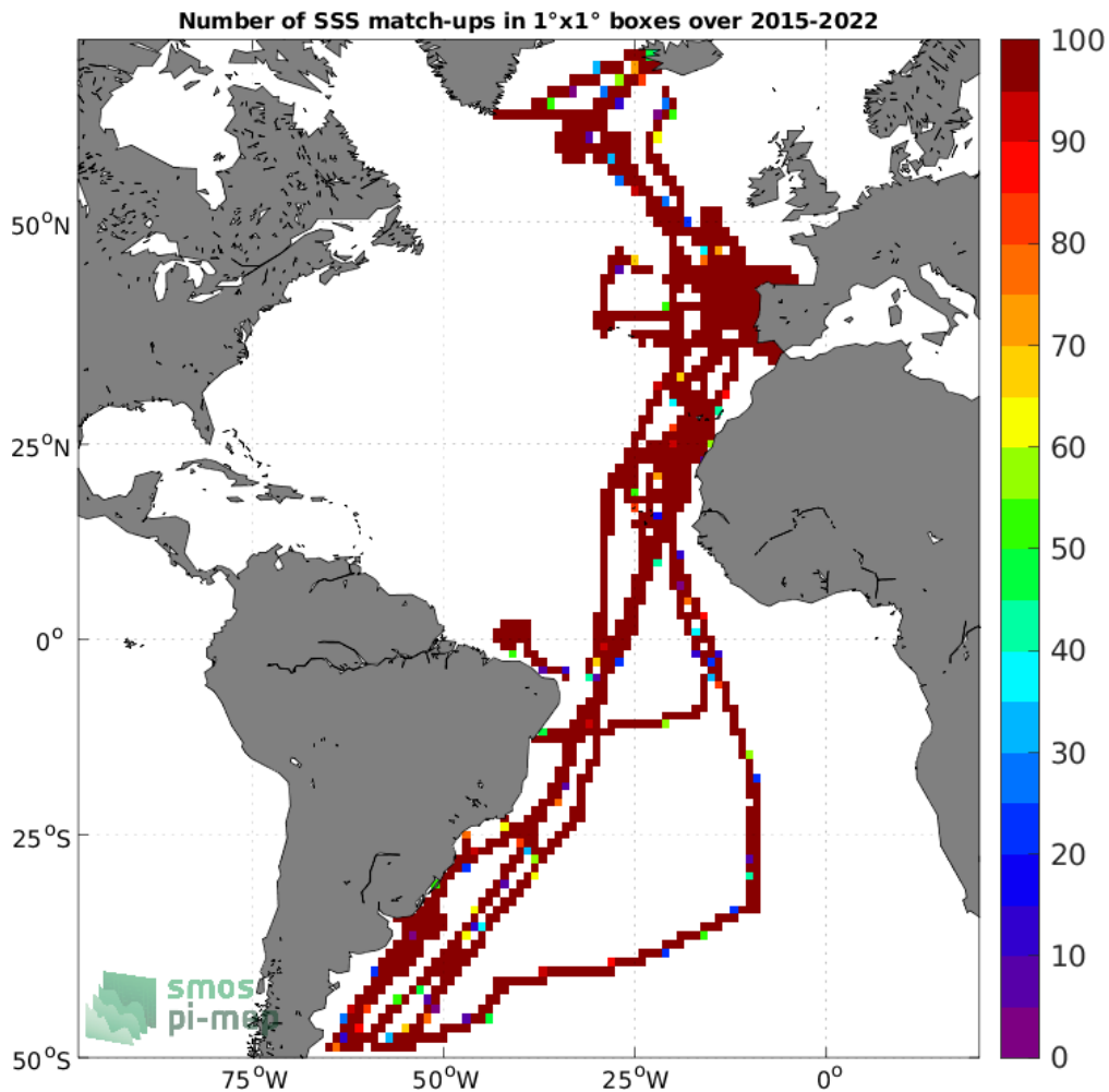
Figure 4: Number of SSS match-ups between TSG (CSIC-UTM) SSS and the SMAP SSS L3 v5.0 - Monthly (JPL) SSS product for the Atlantic Ocean Pi-MEP region over 1°x1° boxes and for the full satellite product period.
