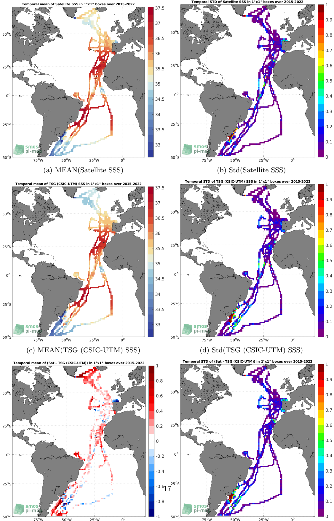
(e) MEAN( \Delta SSS) (Satellite - TSG (CSIC-UTM)) (f) Std( \Delta SSS) (Satellite - TSG (CSIC-UTM)) Figure 6: Temporal mean (left) and Std (right) of SSS from SMAP SSS L3 v5.0 - Monthly (JPL) (top), TSG (CSIC-UTM) (middle), and of \Delta SSS (Satellite - TSG (CSIC-UTM)). Only match-up pairs are used to generate these maps.
