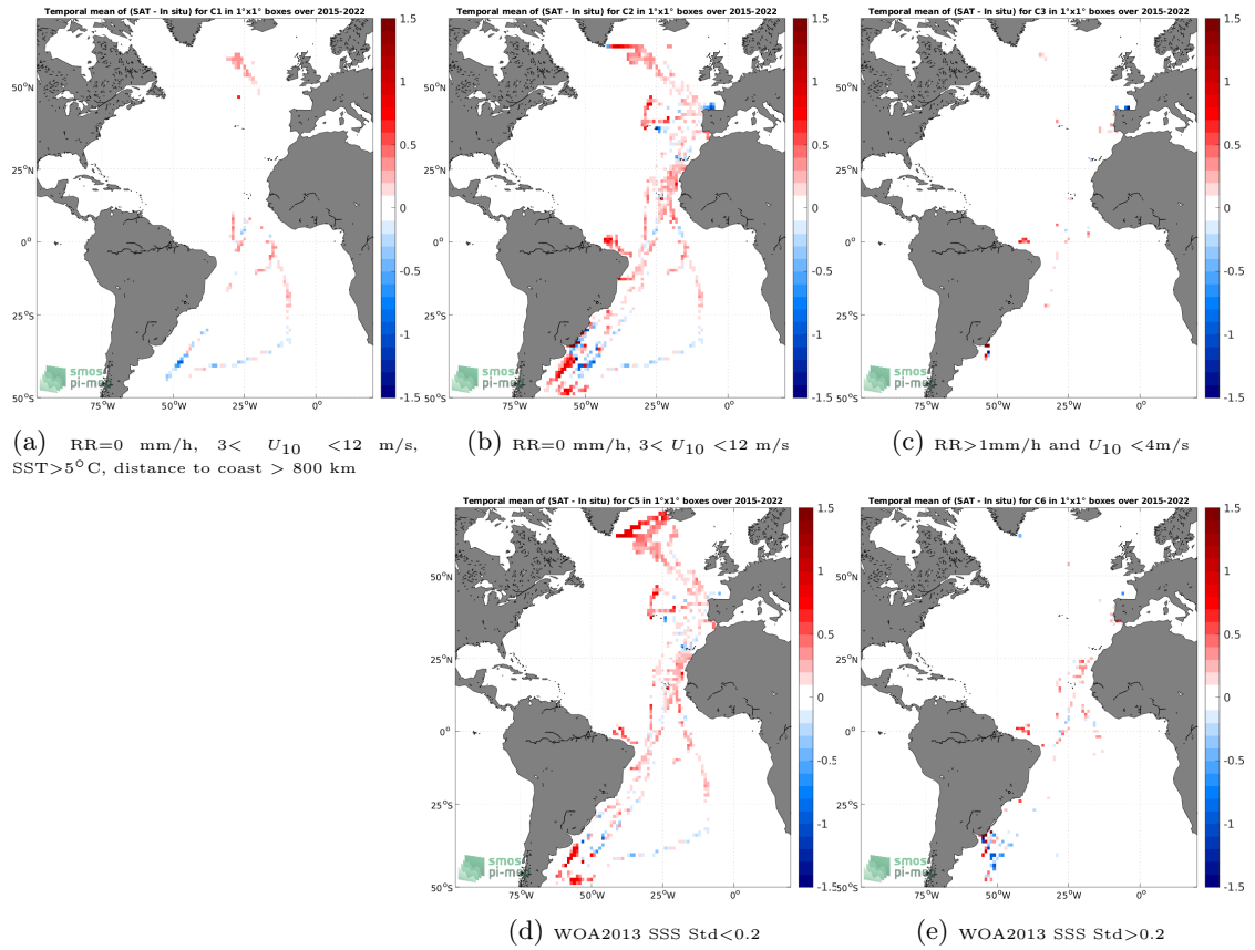
Figure 12: Temporal mean gridded over spatial boxes of size 1^\circ \times 1^\circ of \Delta SSS (SMAP SSS L3 v5.0 - Monthly (JPL) - TSG (CSIC-UTM)) for 5 different subdatasets corresponding to:RR=0 mm/h, 3 < U_{10} < 12 m/s, SST >5^\circ\text{C} , distance to coast > 800 km (a), RR=0 mm/h, 3 < U_{10} < 12 m/s (b), RR >1 mm/h and U_{10} < 4 m/s (c), WOA2013 SSS Std <0.2 (d), WOA2013 SSS Std >0.2 (e).
