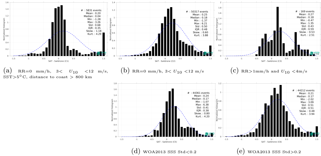
Figure 15: Normalized histogram of \Delta SSS (SMAP SSS L3 v5.0 - Monthly (JPL) - SSS (Saildrone)) for 5 different subdatasets corresponding to: RR=0 mm/h, 3 < U_{10} < 12 m/s, SST > 5°C, distance to coast > 800 km (a), RR=0 mm/h, 3 < U_{10} < 12 m/s (b), RR > 1mm/h and U_{10} < 4 m/s (c), WOA2013 SSS Std < 0.2 (d), WOA2013 SSS Std > 0.2 (e).
