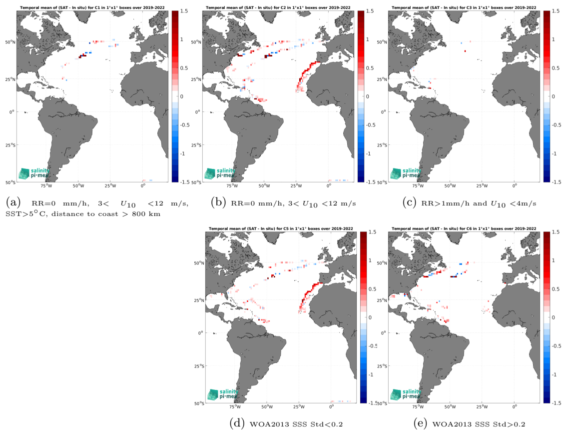
Figure 14: Temporal mean gridded over spatial boxes of size 1^\circ \times 1^\circ of \Delta\text{SSS} (SMAP SSS L3 v5.0 - Monthly (JPL) - Sairdrone) for 5 different subdatasets corresponding to:RR=0 mm/h, 3 < U_{10} < 12 m/s, SST >5^\circ\text{C} , distance to coast > 800 km (a), RR=0 mm/h, 3 < U_{10} < 12 m/s (b), RR >1 mm/h and U_{10} < 4 m/s (c), WOA2013 SSS Std <0.2 (d), WOA2013 SSS Std >0.2 (e).
