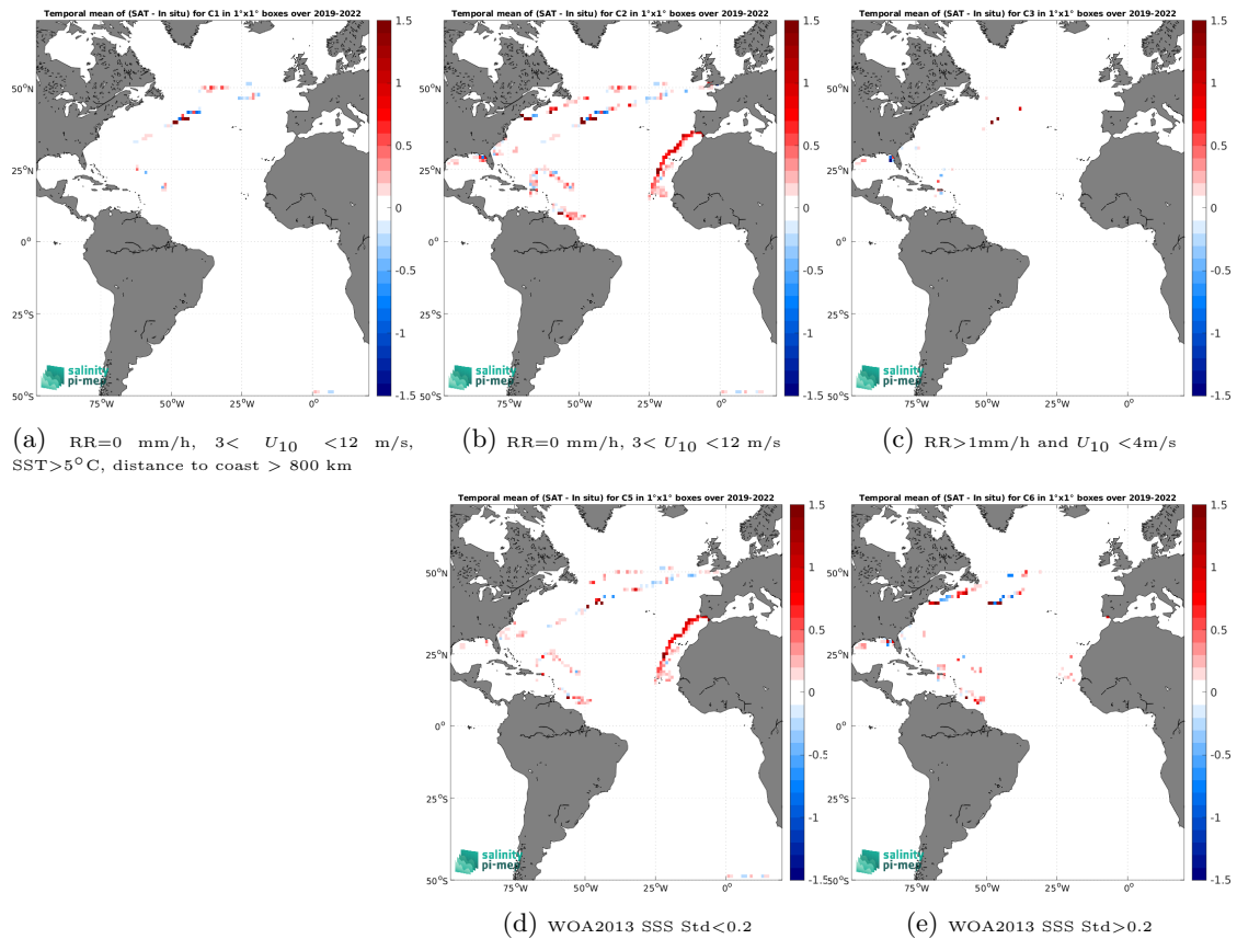
Figure 12: Temporal mean gridded over spatial boxes of size 1^\circ \times 1^\circ of \Delta\text{SSS} (SMAP SSS L3 v5.0 - Monthly (JPL) - Saildrone) for 5 different subdatasets corresponding to:RR=0 mm/h, 3 < U_{10} < 12 m/s, SST >5^\circ\text{C} , distance to coast > 800 km (a), RR=0 mm/h, 3 < U_{10} < 12 m/s (b), RR >1 mm/h and U_{10} < 4 m/s (c), WOA2013 SSS Std <0.2 (d), WOA2013 SSS Std >0.2 (e).
