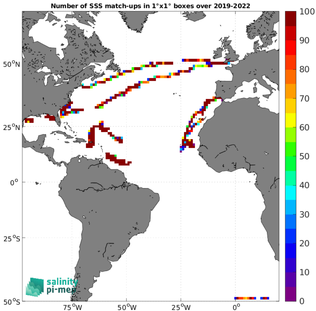
Figure 4: Number of SSS match-ups between Saildrone SSS and the SMAP SSS L3 v5.0 - Monthly (JPL) SSS product for the Atlantic Ocean Pi-MEP region over 1^\circ \times 1^\circ boxes and for the full satellite product period.
