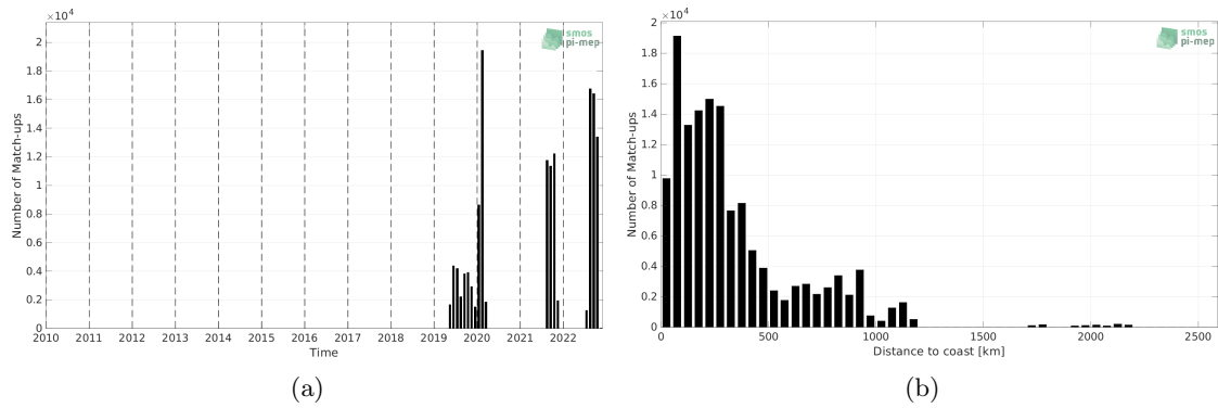
Figure 1: Number of match-ups between Saildrone and SMAP SSS L3 v5.0 - Monthly (JPL) SSS as a function of time (a) and as function of the distance to coast (b) over the Atlantic Ocean Pi-MEP region and for the full satellite product period.
