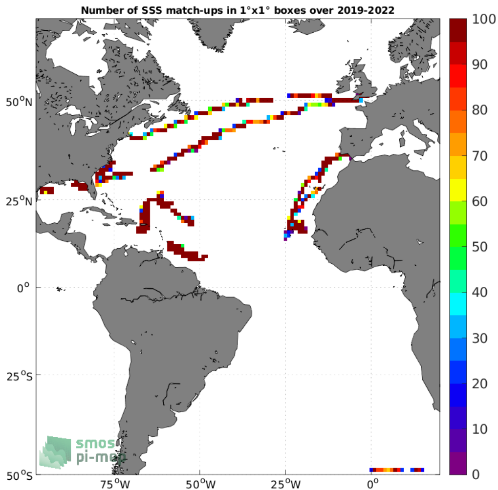
Figure 4: Number of SSS match-ups between Saildrone SSS and the SMAP SSS L3 v5.0 - Monthly (JPL) SSS product for the Atlantic Ocean Pi-MEP region over 1°x1° boxes and for the full satellite product period.
