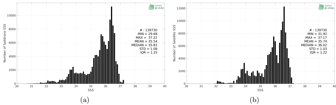
Figure 2: Histograms of SSS from Saildrone (a) and SMAP SSS L3 v5.0 - Monthly (JPL) (b) considering all match-up pairs per bins of 0.1 over the Atlantic Ocean Pi-MEP region and for the full satellite product period.
