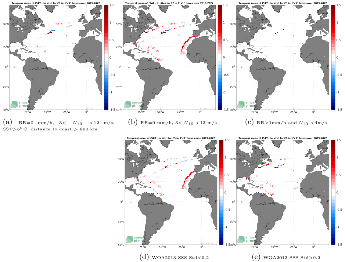
Figure 12: Temporal mean gridded over spatial boxes of size 1^\circ \times 1^\circ of \Delta SSS (SMAP SSS L3 v5.0 - Monthly (JPL) - Sairdrone) for 5 different subdatasets corresponding to:RR=0 mm/h, 3 < U_{10} < 12 m/s, SST >5^\circ\text{C} , distance to coast > 800 km (a), RR=0 mm/h, 3 < U_{10} < 12 m/s (b), RR >1 mm/h and U_{10} < 4 m/s (c), WOA2013 SSS Std <0.2 (d), WOA2013 SSS Std >0.2 (e).
