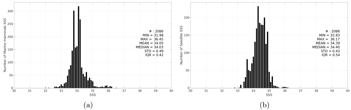
Figure 3: Histograms of SSS from Marine mammals (a) and SMAP SSS L3 v5.0 - Monthly (JPL) (b) considering all match-up pairs per bins of 0.1 over the Atlantic Ocean Pi-MEP region and for the full satellite product period.
