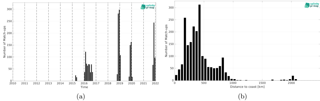
Figure 2: Number of match-ups between Marine mammals and SMAP SSS L3 v5.0 - Monthly (JPL) SSS as a function of time (a) and as function of the distance to coast (b) over the Atlantic Ocean Pi-MEP region and for the full satellite product period.
