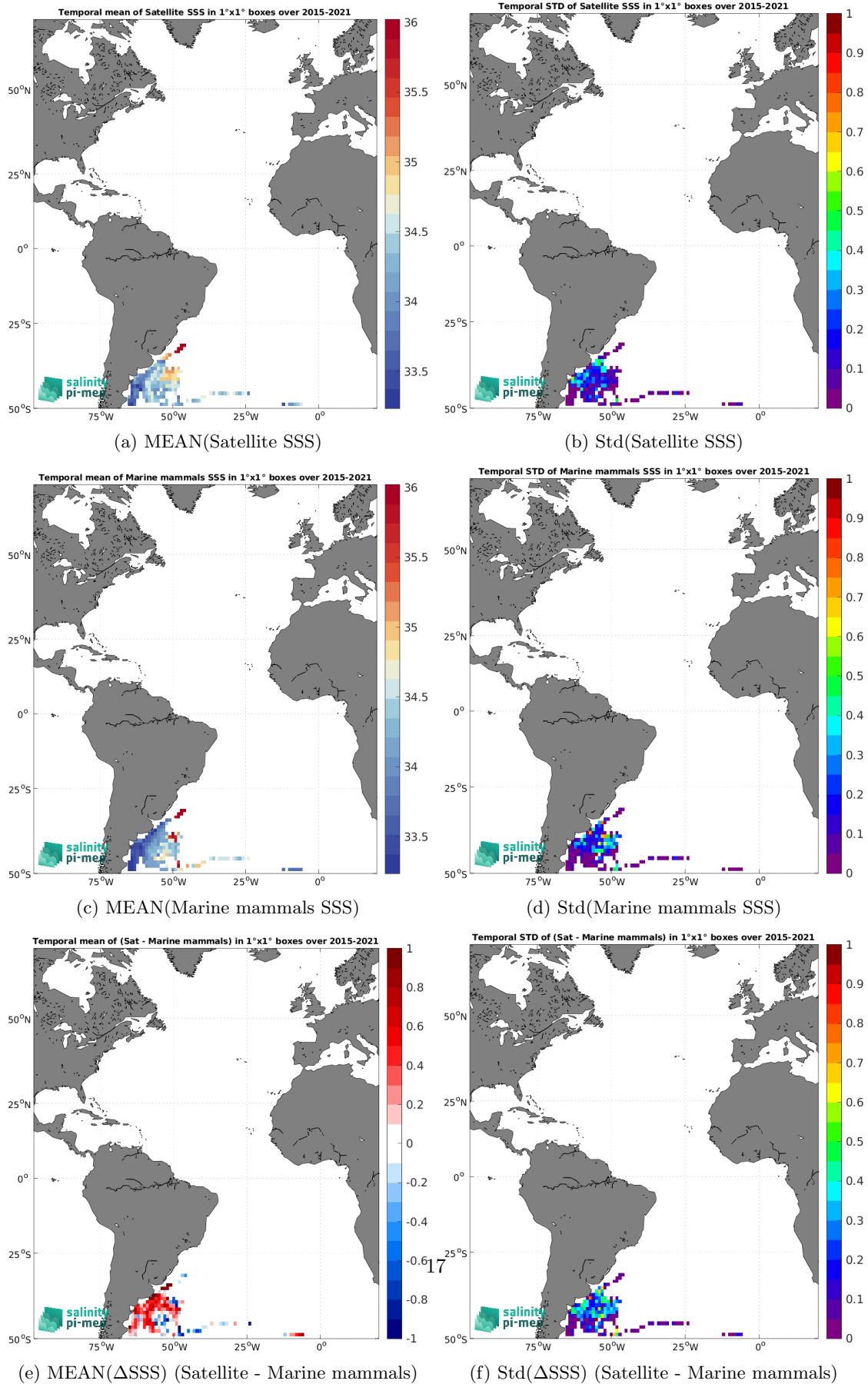
Figure 7: Temporal mean (left) and Std (right) of SSS from SMAP SSS L3 v5.0 - Monthly (JPL) (top), Marine mammals (middle), and of \Delta SSS (Satellite - Marine mammals). Only match-up pairs are used to generate these maps.
