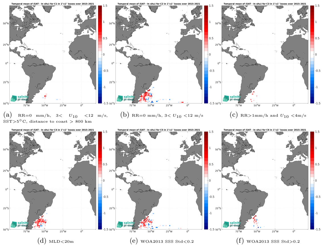
Figure 14: Temporal mean gridded over spatial boxes of size 1^\circ \times 1^\circ of \Delta SSS (SMAP SSS L3 v5.0 - Monthly (JPL) - Marine mammals) for 6 different subdatasets corresponding to: RR=0 mm/h, 3 < U_{10} < 12 m/s, SST > 5^\circ\text{C} , distance to coast > 800 km (a), RR=0 mm/h, 3 < U_{10} < 12 m/s (b), RR > 1 mm/h and U_{10} < 4 m/s (c), MLD < 20 m (d), WOA2013 SSS Std < 0.2 (e), WOA2013 SSS Std > 0.2 (f).
