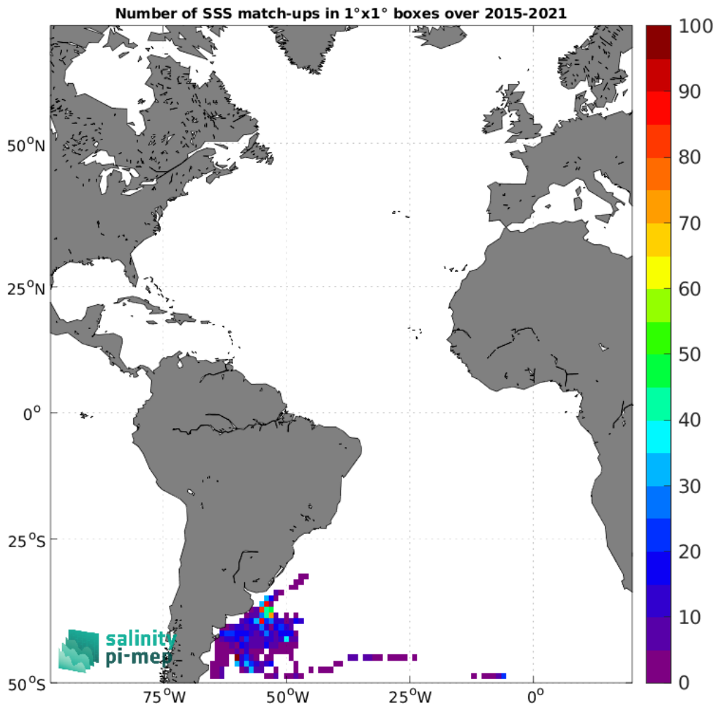
Figure 5: Number of SSS match-ups between Marine mammals SSS and the SMAP SSS L3 v5.0 - Monthly (JPL) SSS product for the Atlantic Ocean Pi-MEP region over 1^\circ \times 1^\circ boxes and for the full satellite product period.
