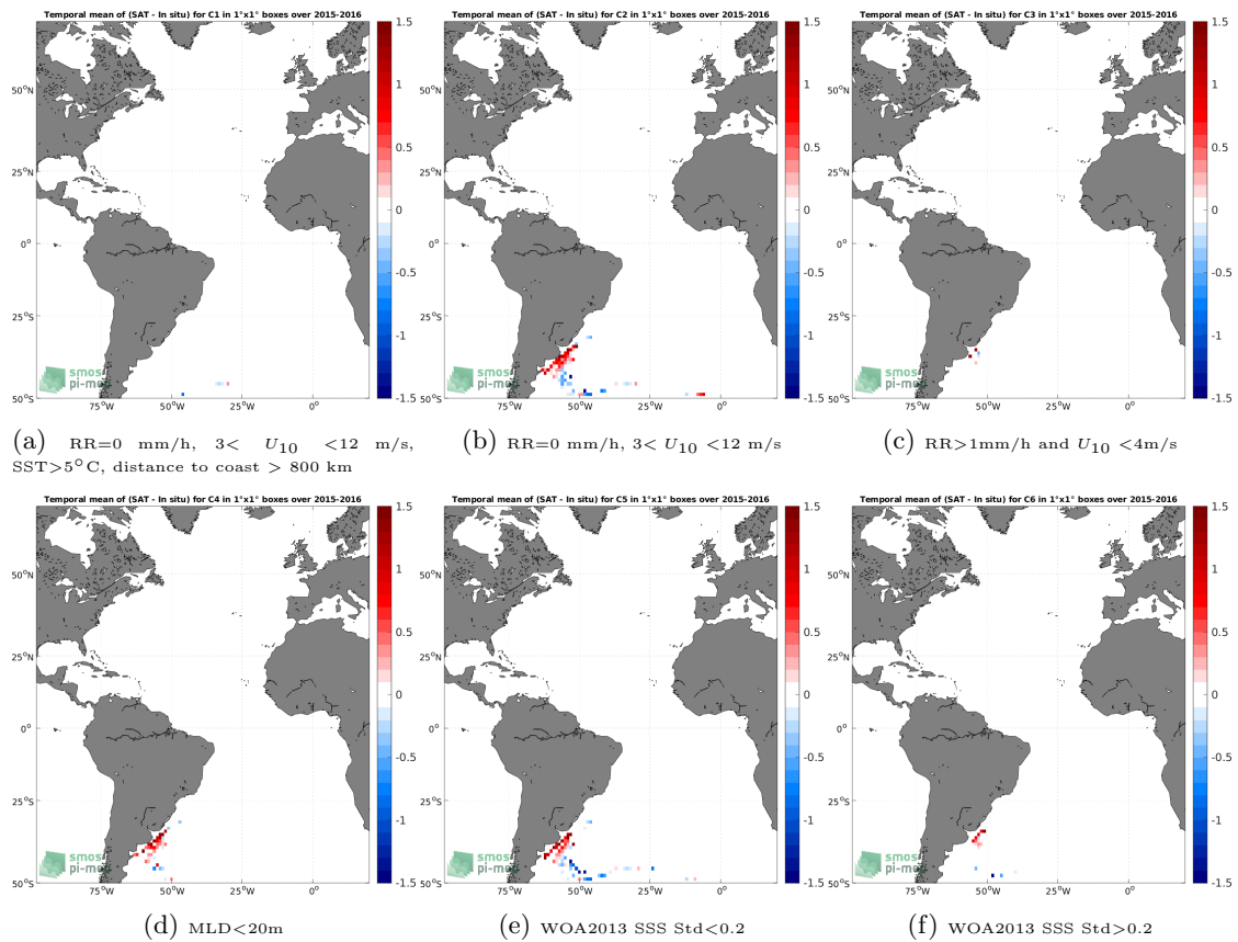
Figure 12: Temporal mean gridded over spatial boxes of size 1^\circ \times 1^\circ of \Delta SSS (SMAP SSS L3 v5.0 - Monthly (JPL) - Marine mammals) for 6 different subdatasets corresponding to: RR=0 mm/h, 3 < U_{10} < 12 m/s, SST > 5^\circ\text{C} , distance to coast > 800 km (a), RR=0 mm/h, 3 < U_{10} < 12 m/s (b), RR > 1 mm/h and U_{10} < 4 m/s (c),MLD < 20 m (d),WOA2013 SSS Std < 0.2 (e),WOA2013 SSS Std > 0.2 (f).
