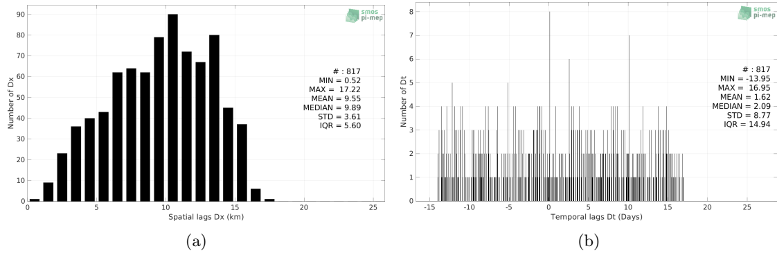
Figure 5: Histograms of the spatial (a) and temporal (b) lags between the location/time of the Marine mammals measurement and the date of the corresponding SMAP SSS L3 v5.0 - Monthly (JPL) SSS pixel.
