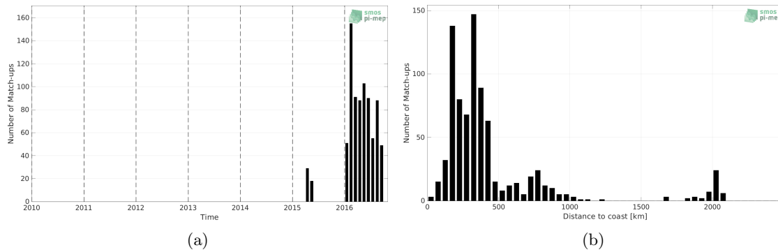
Figure 1: Number of match-ups between Marine mammals and SMAP SSS L3 v5.0 - Monthly (JPL) SSS as a function of time (a) and as function of the distance to coast (b) over the Atlantic Ocean Pi-MEP region and for the full satellite product period.
