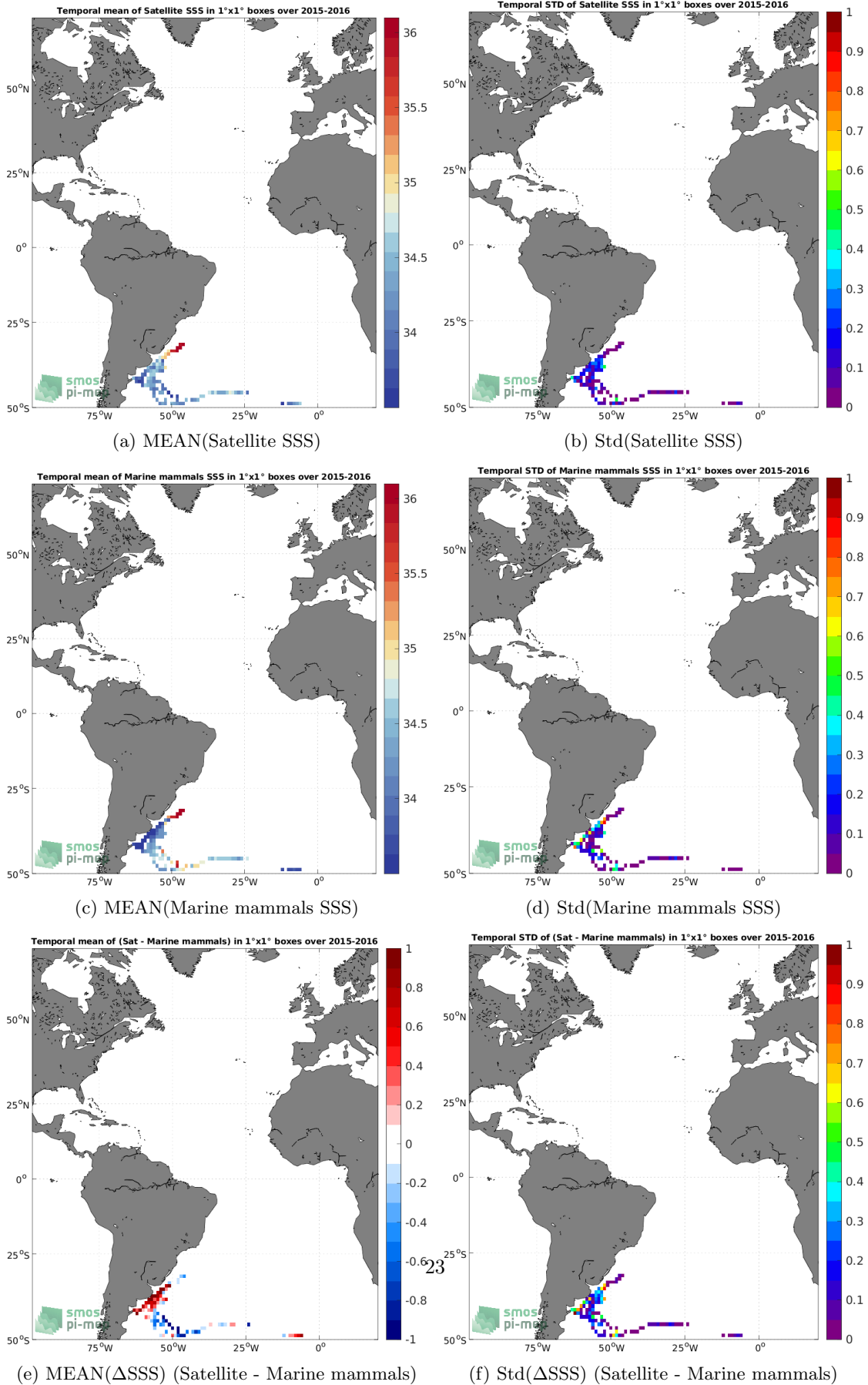
Figure 6: Temporal mean (left) and Std (right) of SSS from SMAP SSS L3 v5.0 - Monthly (JPL) (top), Marine mammals (middle), and of \Delta SSS (Satellite - Marine mammals). Only match-up pairs are used to generate these maps.
