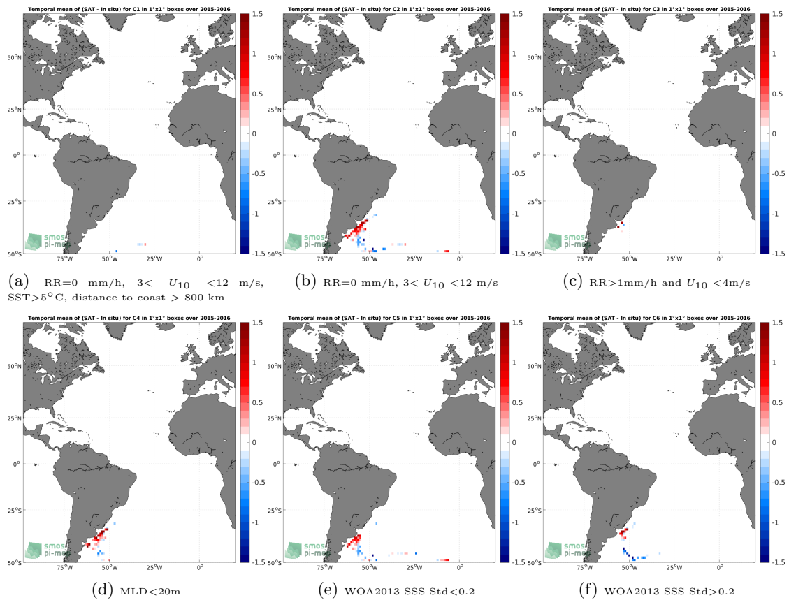
Figure 12: Temporal mean gridded over spatial boxes of size 1^\circ \times 1^\circ of \Delta SSS (SMAP SSS L3 v5.0 - Monthly (JPL) - Marine mammals) for 6 different subdatasets corresponding to:RR=0 mm/h, 3 < U_{10} < 12 m/s, SST >5^\circ C, distance to coast > 800 km (a), RR=0 mm/h, 3 < U_{10} < 12 m/s (b), RR >1 mm/h and U_{10} < 4 m/s (c),MLD <20 m (d),WOA2013 SSS Std <0.2 (e),WOA2013 SSS Std >0.2 (f).
