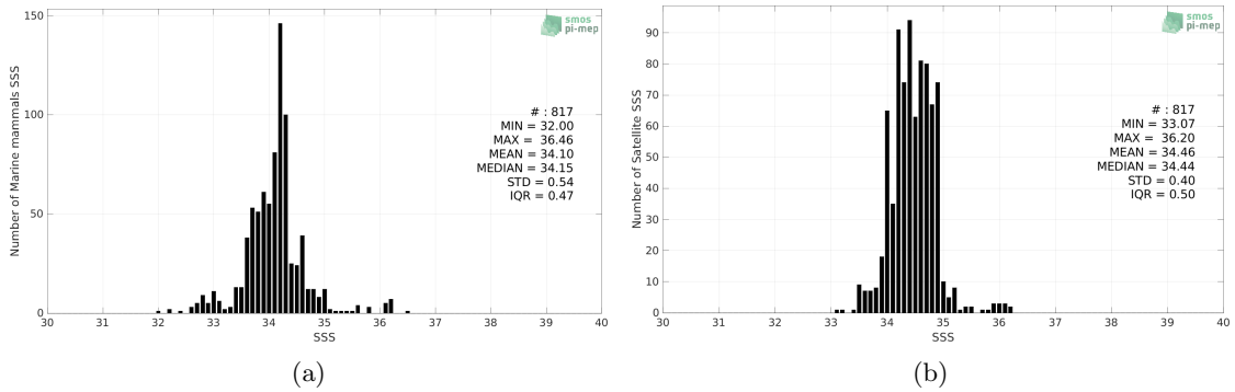
Figure 2: Histograms of SSS from Marine mammals (a) and SMAP SSS L3 v5.0 - Monthly (JPL) (b) considering all match-up pairs per bins of 0.1 over the Atlantic Ocean Pi-MEP region and for the full satellite product period.
