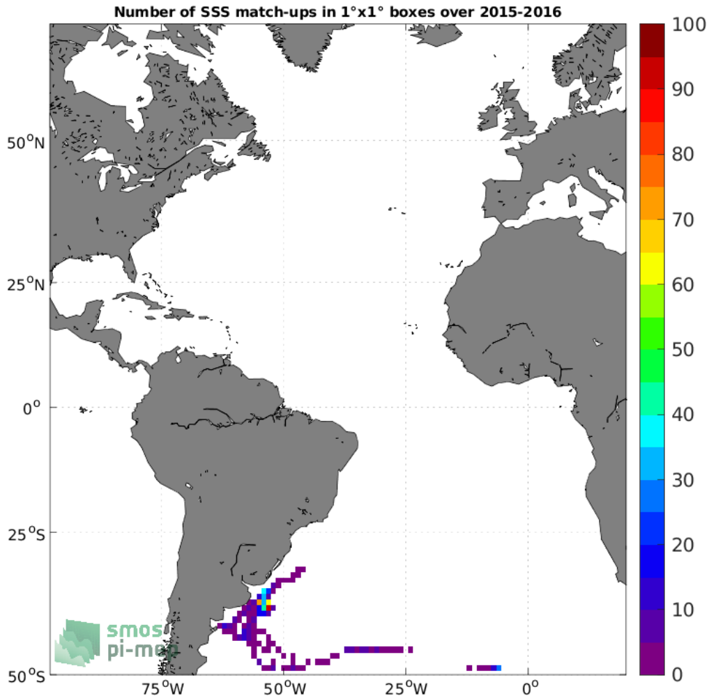
Figure 4: Number of SSS match-ups between Marine mammals SSS and the SMAP SSS L3 v5.0 - Monthly (JPL) SSS product for the Atlantic Ocean Pi-MEP region over 1^\circ \times 1^\circ boxes and for the full satellite product period.
