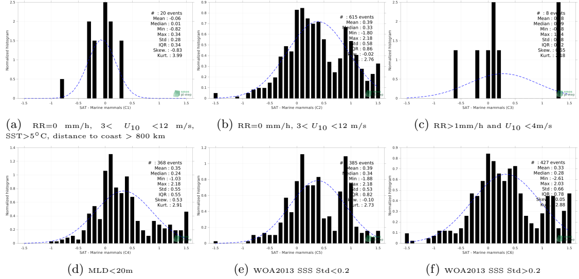
Figure 13: Normalized histogram of \Delta SSS (SMAP SSS L3 v5.0 - Monthly (JPL) - Marine mammals) for 6 different subdatasets corresponding to: RR=0 mm/h, 3 < U_{10} < 12 m/s, SST>5°C, distance to coast > 800 km (a), RR=0 mm/h, 3 < U_{10} < 12 m/s (b), RR>1mm/h and U_{10} < 4 m/s (c), MLD<20m (d), WOA2013 SSS Std<0.2 (e), WOA2013 SSS Std>0.2 (f).
