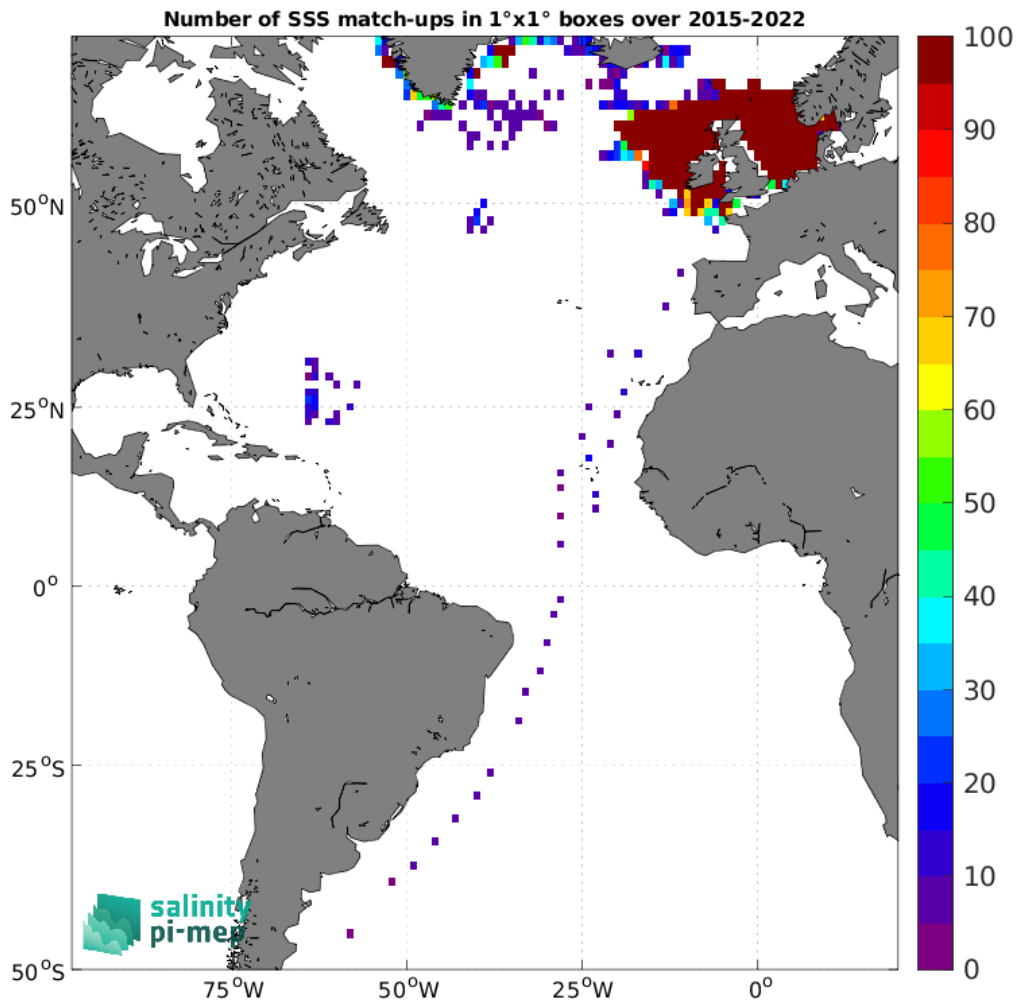
Figure 4: Number of SSS match-ups between ICES SSS and the SMAP SSS L3 v5.0 - Monthly (JPL) SSS product for the Atlantic Ocean Pi-MEP region over 1^{\circ} \times 1^{\circ} boxes and for the full satellite product period.
