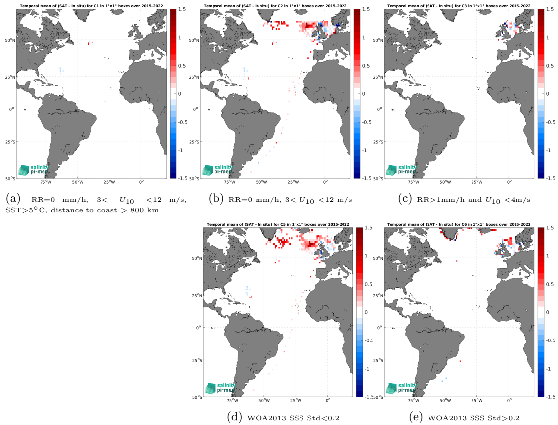
Figure 12: Temporal mean gridded over spatial boxes of size 1^\circ \times 1^\circ of \Delta SSS (SMAP SSS L3 v5.0 - Monthly (JPL) - ICES) for 5 different subdatasets corresponding to:RR=0 mm/h, 3 < U_{10} < 12 m/s, SST >5^\circ\text{C} , distance to coast > 800 km (a), RR=0 mm/h, 3 < U_{10} < 12 m/s (b), RR >1 mm/h and U_{10} < 4 m/s (c), WOA2013 SSS Std <0.2 (d), WOA2013 SSS Std >0.2 (e).
