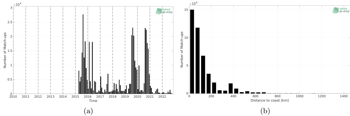
Figure 1: Number of match-ups between ICES and SMAP SSS L3 v5.0 - Monthly (JPL) SSS as a function of time (a) and as function of the distance to coast (b) over the Atlantic Ocean Pi-MEP region and for the full satellite product period.
