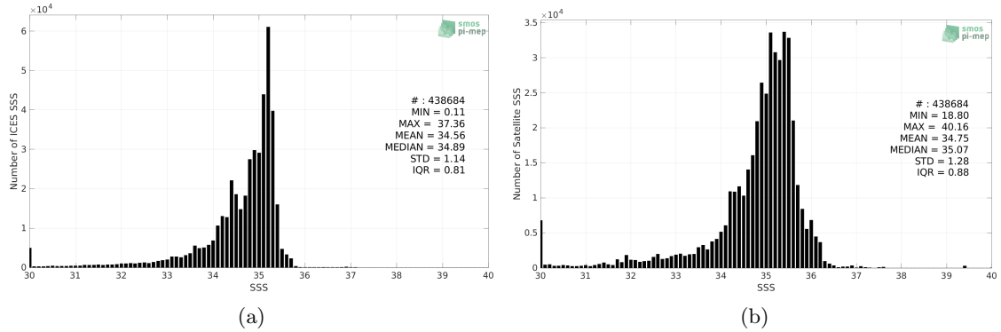
Figure 2: Histograms of SSS from ICES (a) and SMAP SSS L3 v5.0 - Monthly (JPL) (b) considering all match-up pairs per bins of 0.1 over the Atlantic Ocean Pi-MEP region and for the full satellite product period.
