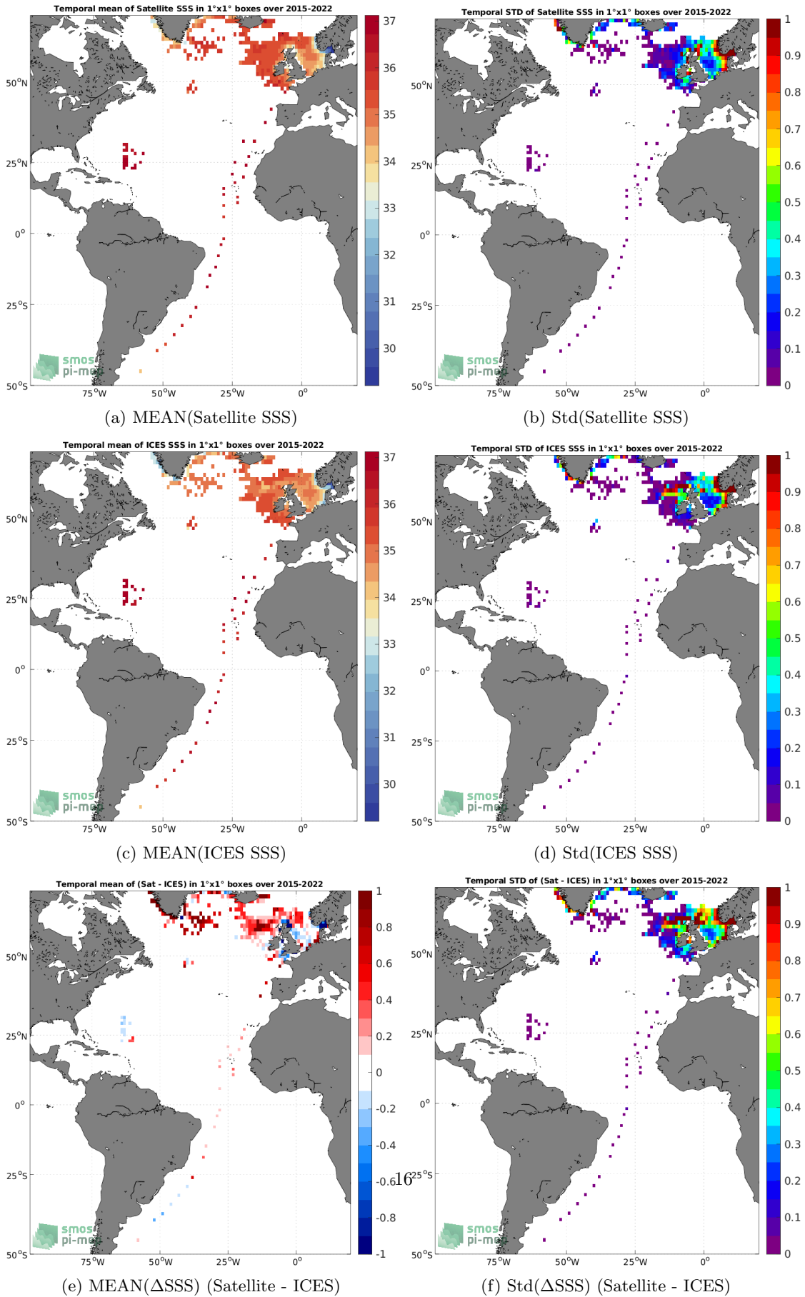
Figure 6: Temporal mean (left) and Std (right) of SSS from SMAP SSS L3 v5.0 - Monthly (JPL) (top), ICES (middle), and of \Delta SSS (Satellite - ICES). Only match-up pairs are used to generate these maps.
