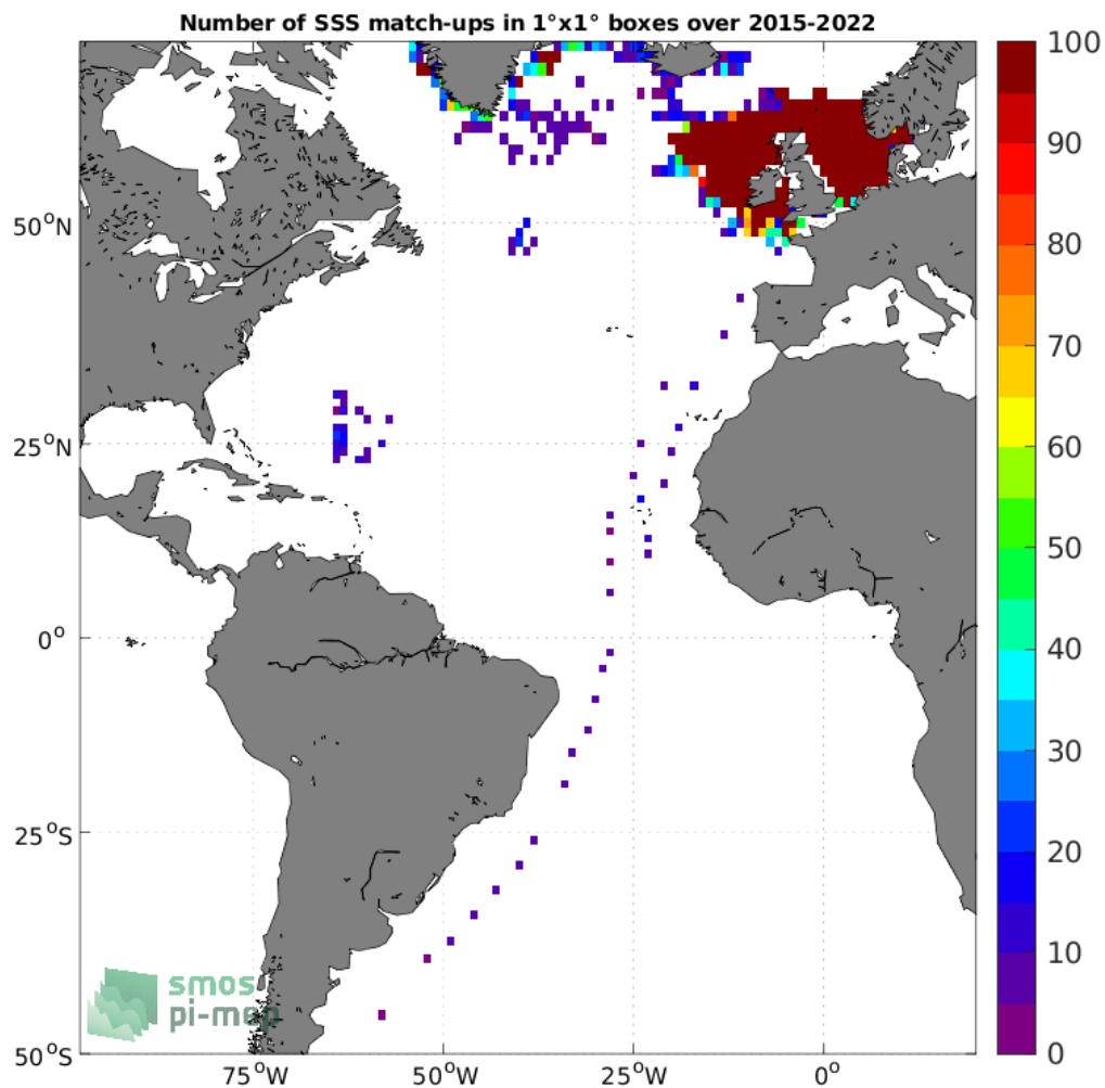
Figure 4: Number of SSS match-ups between ICES SSS and the SMAP SSS L3 v5.0 - Monthly (JPL) SSS product for the Atlantic Ocean Pi-MEP region over 1°x1° boxes and for the full satellite product period.
