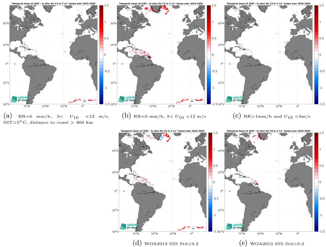
Figure 13: Temporal mean gridded over spatial boxes of size 1^\circ \times 1^\circ of \Delta SSS (SMAP SSS L3 v5.0 - Monthly (JPL) - Surface drifters) for 5 different subdatasets corresponding to:RR=0 mm/h, 3 < U_{10} < 12 m/s, SST >5^\circ\text{C} , distance to coast > 800 km (a), RR=0 mm/h, 3 < U_{10} < 12 m/s (b), RR >1 mm/h and U_{10} < 4 m/s (c), WOA2013 SSS Std <0.2 (d), WOA2013 SSS Std >0.2 (e).
