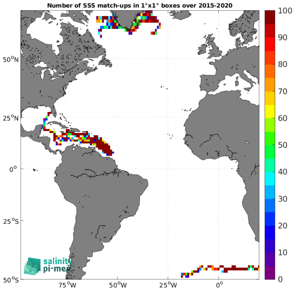
Figure 4: Number of SSS match-ups between Surface drifters SSS and the SMAP SSS L3 v5.0 - Monthly (JPL) SSS product for the Atlantic Ocean Pi-MEP region over 1°×1° boxes and for the full satellite product period.
