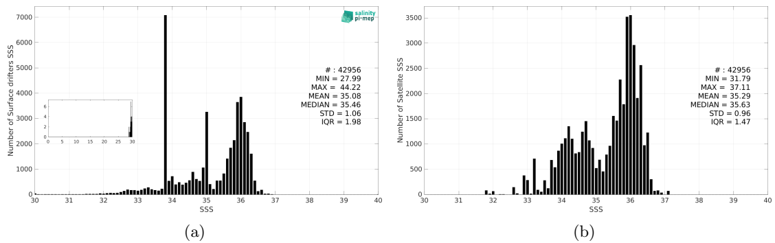
Figure 3: Histograms of SSS from Surface drifters (a) and SMAP SSS L3 v5.0 - Monthly (JPL) (b) considering all match-up pairs per bins of 0.1 over the Atlantic Ocean Pi-MEP region and for the full satellite product period.
