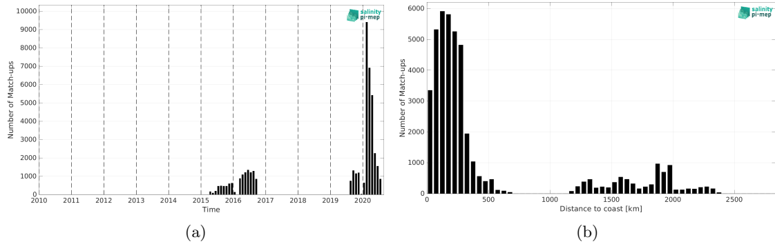
Figure 2: Number of match-ups between Surface drifters and SMAP SSS L3 v5.0 - Monthly (JPL) SSS as a function of time (a) and as function of the distance to coast (b) over the Atlantic Ocean Pi-MEP region and for the full satellite product period.
