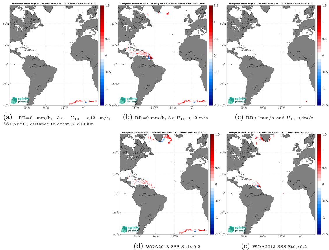
Figure 11: Temporal mean gridded over spatial boxes of size 1^\circ \times 1^\circ of \Delta SSS (SMAP SSS L3 v5.0 - Monthly (JPL) - Surface drifters) for 5 different subdatasets corresponding to:RR=0 mm/h, 3 < U_{10} < 12 m/s, SST >5^\circ\text{C} , distance to coast > 800 km (a), RR=0 mm/h, 3 < U_{10} < 12 m/s (b), RR >1 mm/h and U_{10} < 4 m/s (c), WOA2013 SSS Std <0.2 (d), WOA2013 SSS Std >0.2 (e).
