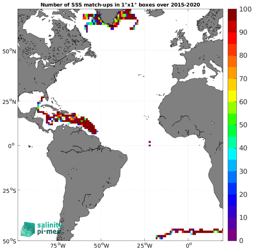
Figure 3: Number of SSS match-ups between Surface drifters SSS and the SMAP SSS L3 v5.0 - Monthly (JPL) SSS product for the Atlantic Ocean Pi-MEP region over 1°×1° boxes and for the full satellite product period.
