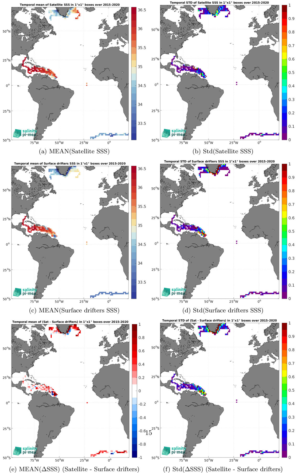
Figure 5: Temporal mean (left) and Std (right) of SSS from SMAP SSS L3 v5.0 - Monthly (JPL) (top), Surface drifters (middle), and of \Delta SSS (Satellite - Surface drifters). Only match-up pairs are used to generate these maps.
