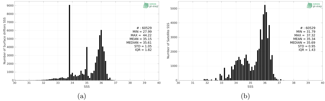
Figure 2: Histograms of SSS from Surface drifters (a) and SMAP SSS L3 v5.0 - Monthly (JPL) (b) considering all match-up pairs per bins of 0.1 over the Atlantic Ocean Pi-MEP region and for the full satellite product period.
