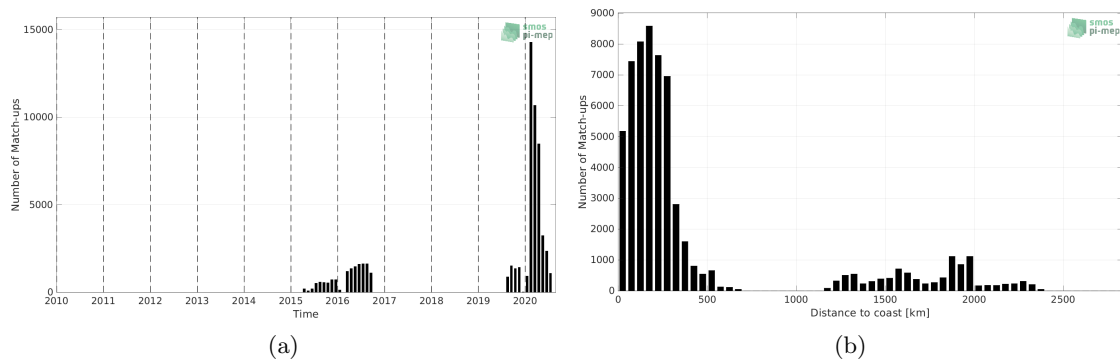
Figure 1: Number of match-ups between Surface drifters and SMAP SSS L3 v5.0 - Monthly (JPL) SSS as a function of time (a) and as function of the distance to coast (b) over the Atlantic Ocean Pi-MEP region and for the full satellite product period.
