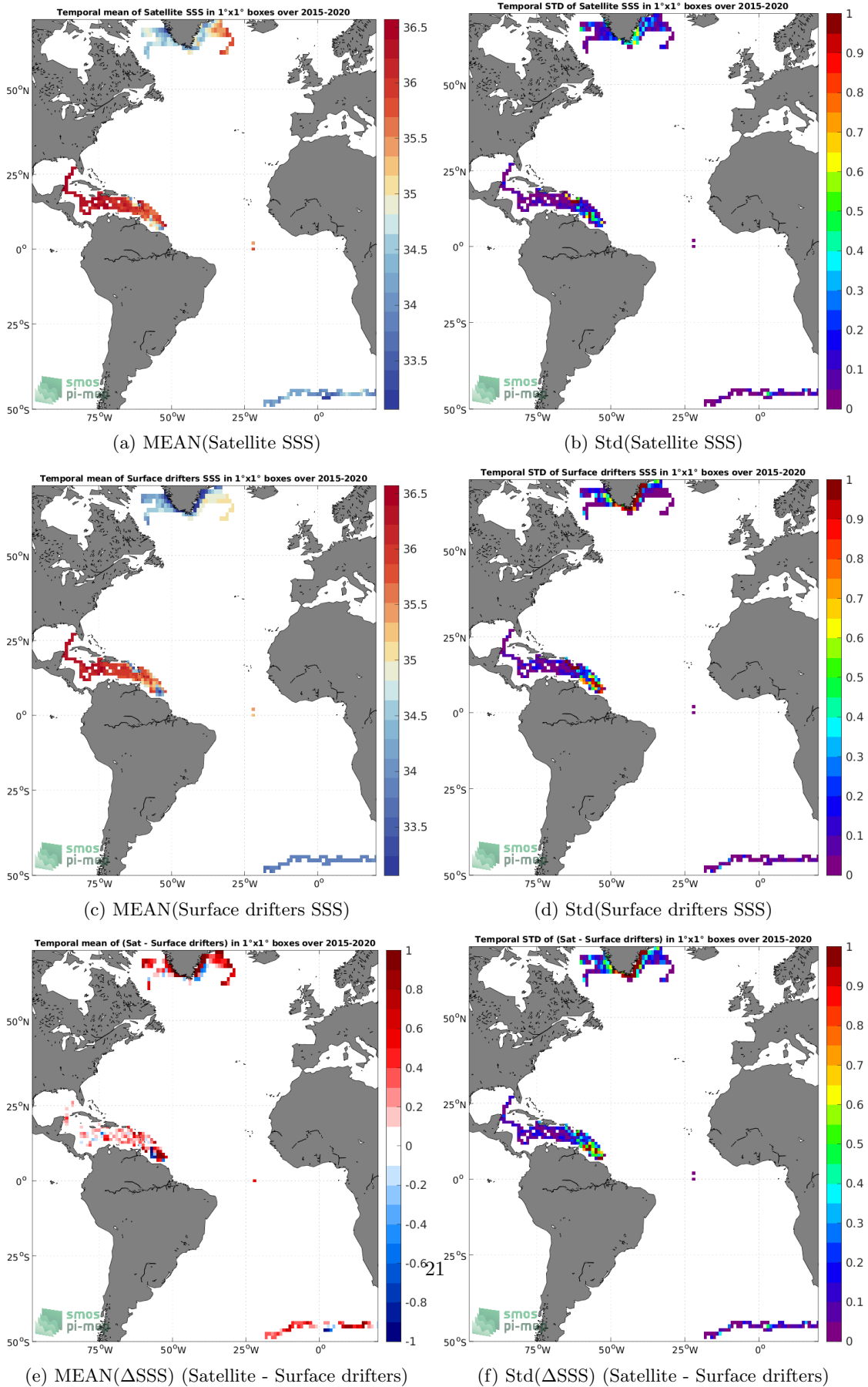
(e) MEAN( \Delta SSS) (Satellite - Surface drifters) (f) Std( \Delta SSS) (Satellite - Surface drifters) Figure 5: Temporal mean (left) and Std (right) of SSS from SMAP SSS L3 v5.0 - Monthly (JPL) (top), Surface drifters (middle), and of \Delta SSS (Satellite - Surface drifters). Only match-up pairs are used to generate these maps.
