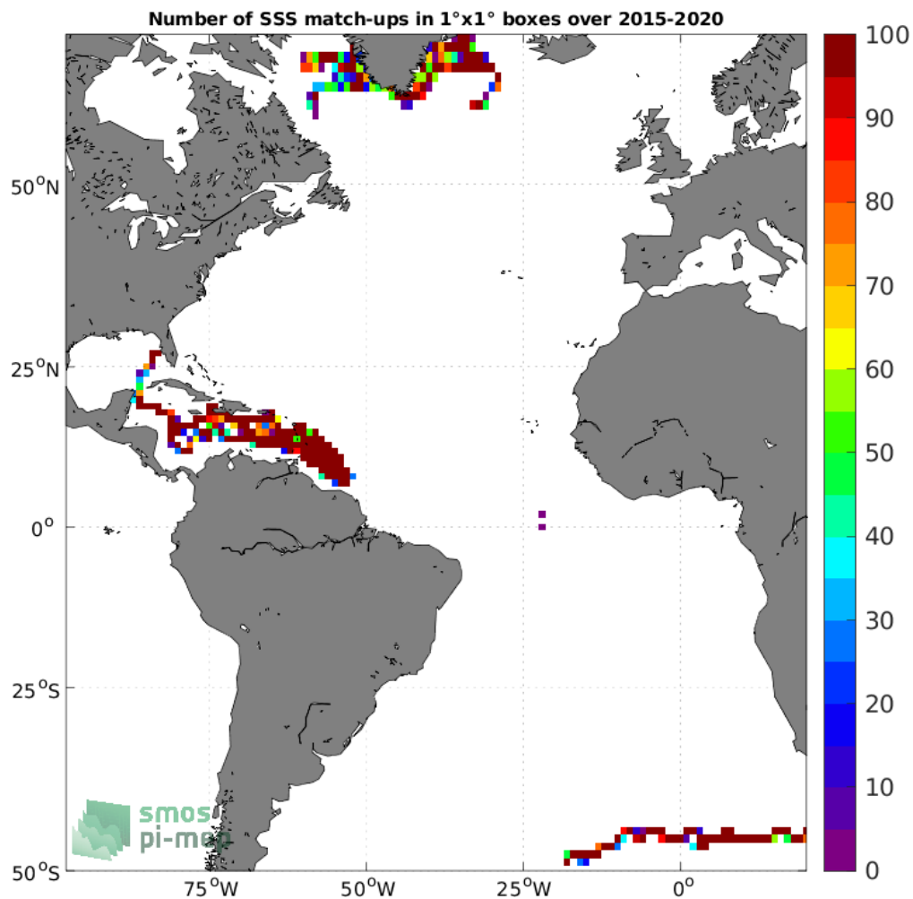
Figure 3: Number of SSS match-ups between Surface drifters SSS and the SMAP SSS L3 v5.0 - Monthly (JPL) SSS product for the Atlantic Ocean Pi-MEP region over 1°x1° boxes and for the full satellite product period.
