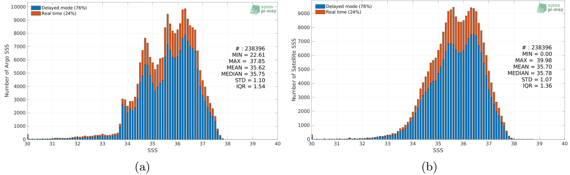
Figure 2: Histograms of SSS from Argo (a) and SMAP SSS L3 v5.0 - Monthly (JPL) (b) considering all match-up pairs per bins of 0.1 over the Atlantic Ocean Pi-MEP region and for the full satellite product period.
