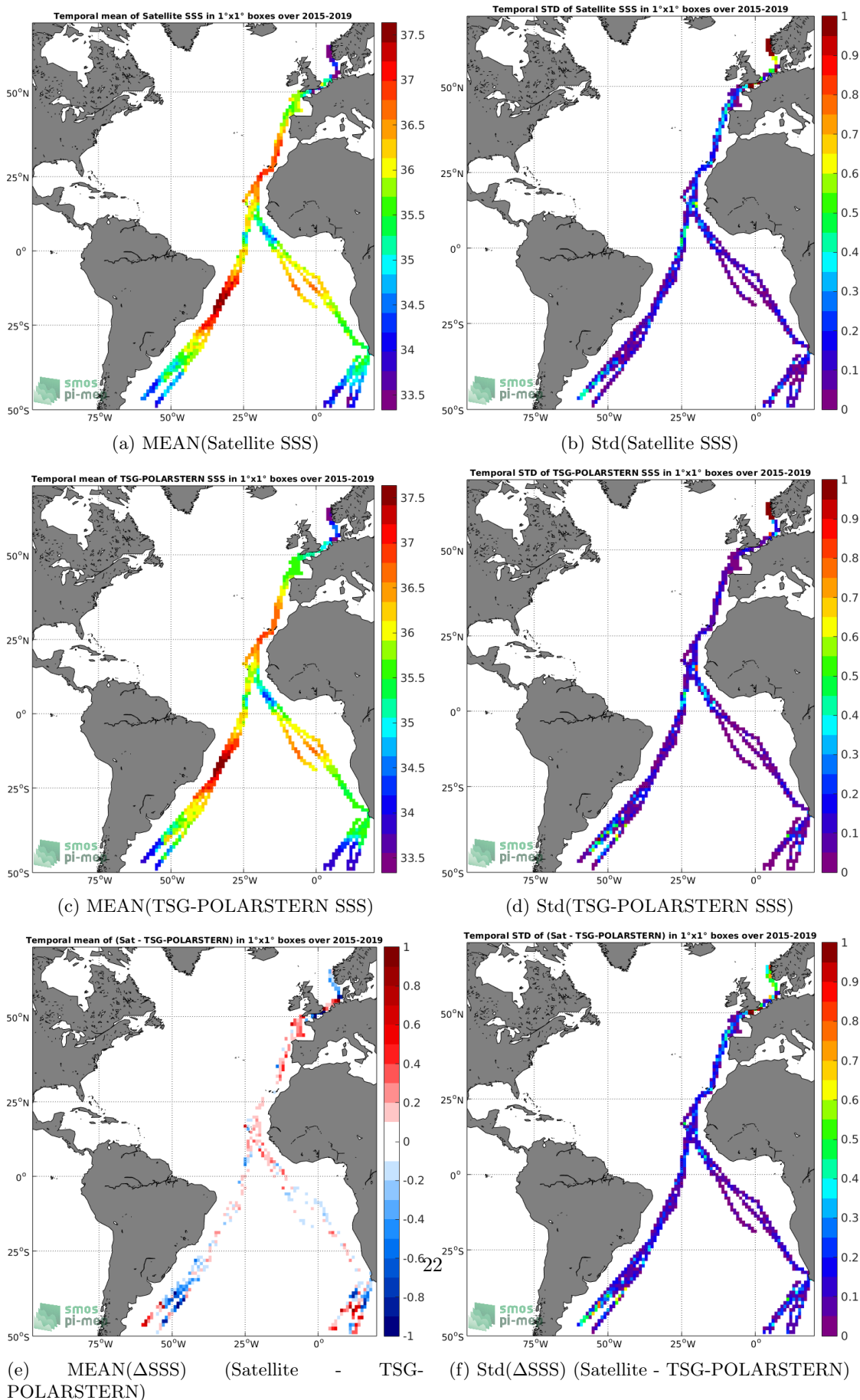
Figure 6: Temporal mean (left) and Std (right) of SSS from SMAP-L3-JPL-V4.3-8DAY-RUNNING-60KM (top), TSG-POLARSTERN (middle), and of \Delta SSS (Satellite - TSG-POLARSTERN). Only match-up pairs are used to generate these maps.
