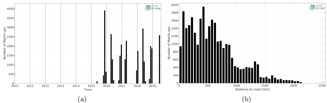
Figure 1: Number of match-ups between TSG-POLARSTERN and SMAP-L3-JPL-V4.3-8DAY-RUNNING-60KM SSS as a function of time (a) and as function of the distance to coast (b) over the Atlantic Ocean Pi-MEP region and for the full satellite product period.
