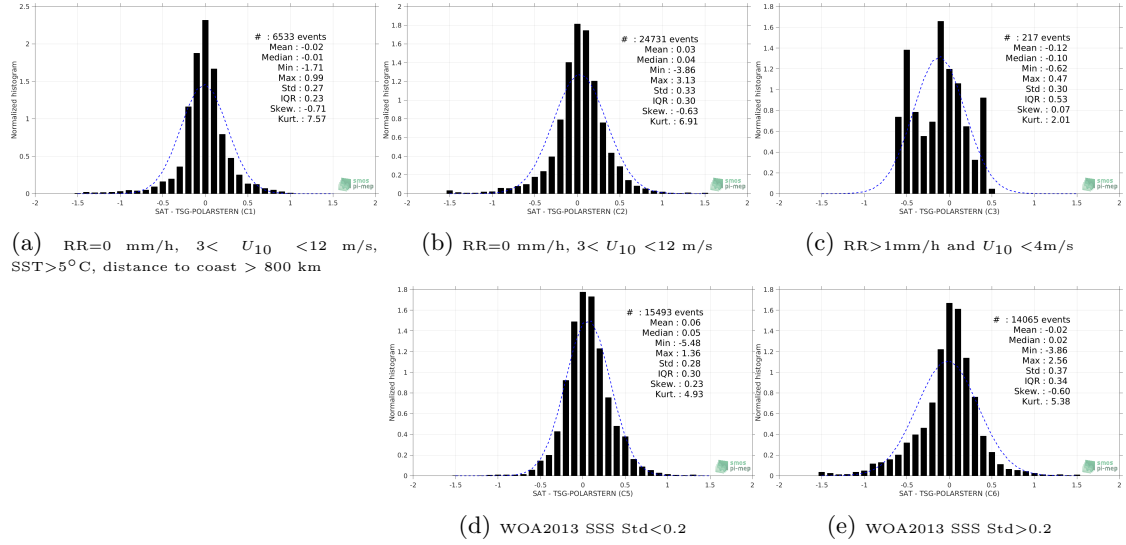
Figure 13: Normalized histogram of \Delta SSS (SMAP-L3-JPL-V4.3-8DAY-RUNNING-60KM - TSG-POLARSTERN) for 5 different subdatasets corresponding to: RR=0 mm/h, 3 < U_{10} < 12 m/s, SST > 5°C, distance to coast > 800 km (a), RR=0 mm/h, 3 < U_{10} < 12 m/s (b), RR > 1mm/h and U_{10} < 4 m/s (c), WOA2013 SSS Std < 0.2 (d), WOA2013 SSS Std > 0.2 (e).
