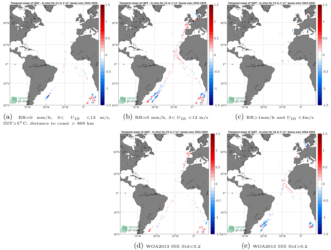
Figure 12: Temporal mean gridded over spatial boxes of size 1^\circ \times 1^\circ of \Delta SSS (SMAP-L3-JPL-V4.3-8DAY-RUNNING-60KM - TSG-POLARSTERN) for 5 different subdatasets corresponding to:RR=0 mm/h, 3 < U_{10} < 12 m/s, SST >5^\circ\text{C} , distance to coast > 800 km (a), RR=0 mm/h, 3 < U_{10} < 12 m/s (b), RR >1 mm/h and U_{10} < 4 m/s (c), WOA2013 SSS Std <0.2 (d), WOA2013 SSS Std >0.2 (e).
