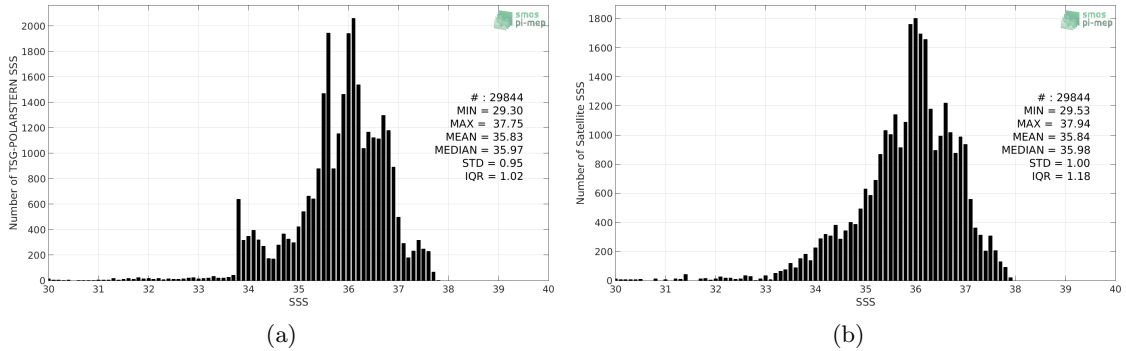
Figure 2: Histograms of SSS from TSG-POLARSTERN (a) and SMAP-L3-JPL-V4.3-8DAY-RUNNING-60KM (b) considering all match-up pairs per bins of 0.1 over the Atlantic Ocean Pi-MEP region and for the full satellite product period.
