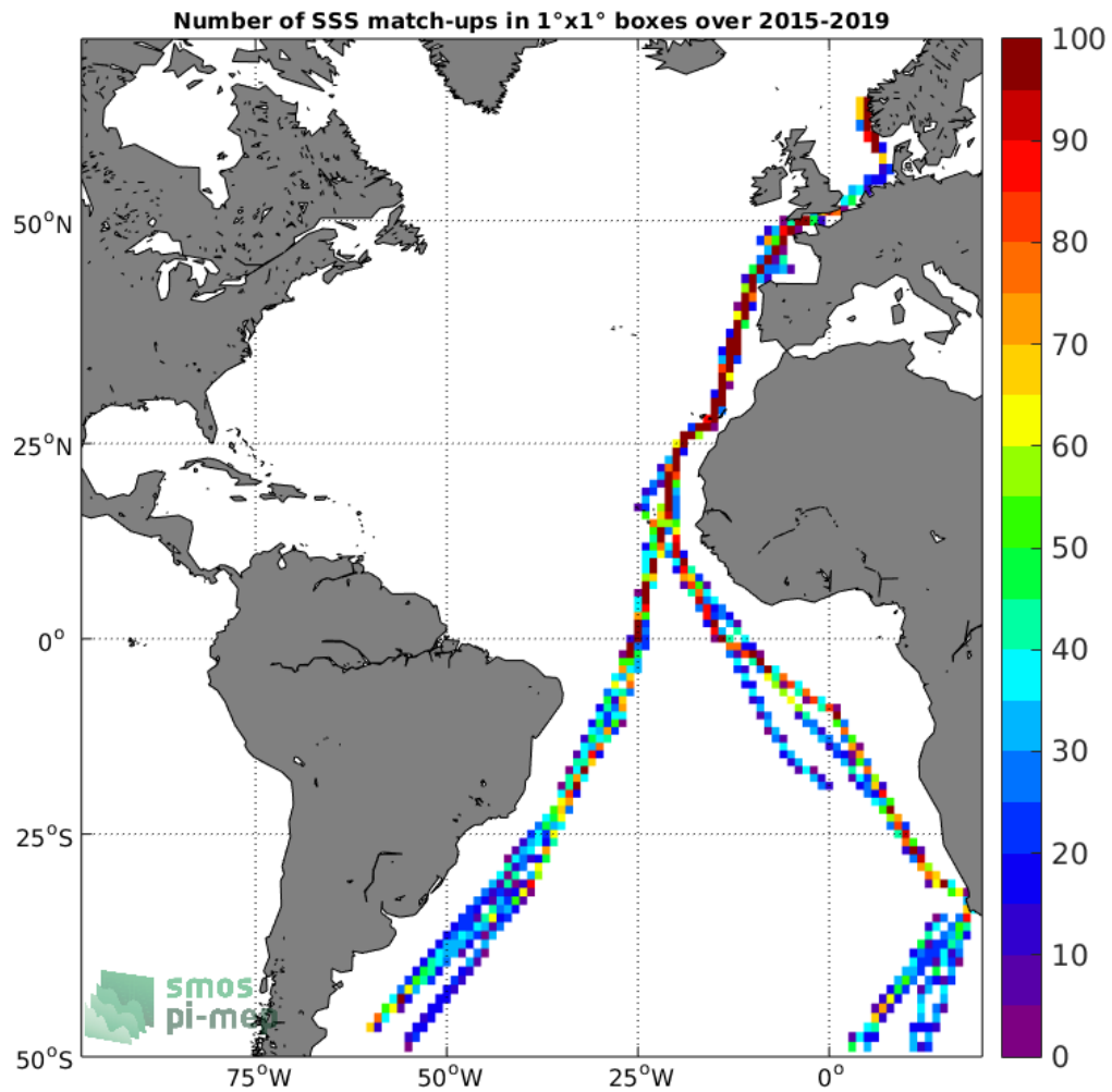
Figure 4: Number of SSS match-ups between TSG-POLARSTERN SSS and the SMAP-L3-JPL-V4.3-8DAY-RUNNING-60KM SSS product for the Atlantic Ocean Pi-MEP region over 1°x1° boxes and for the full satellite product period.
