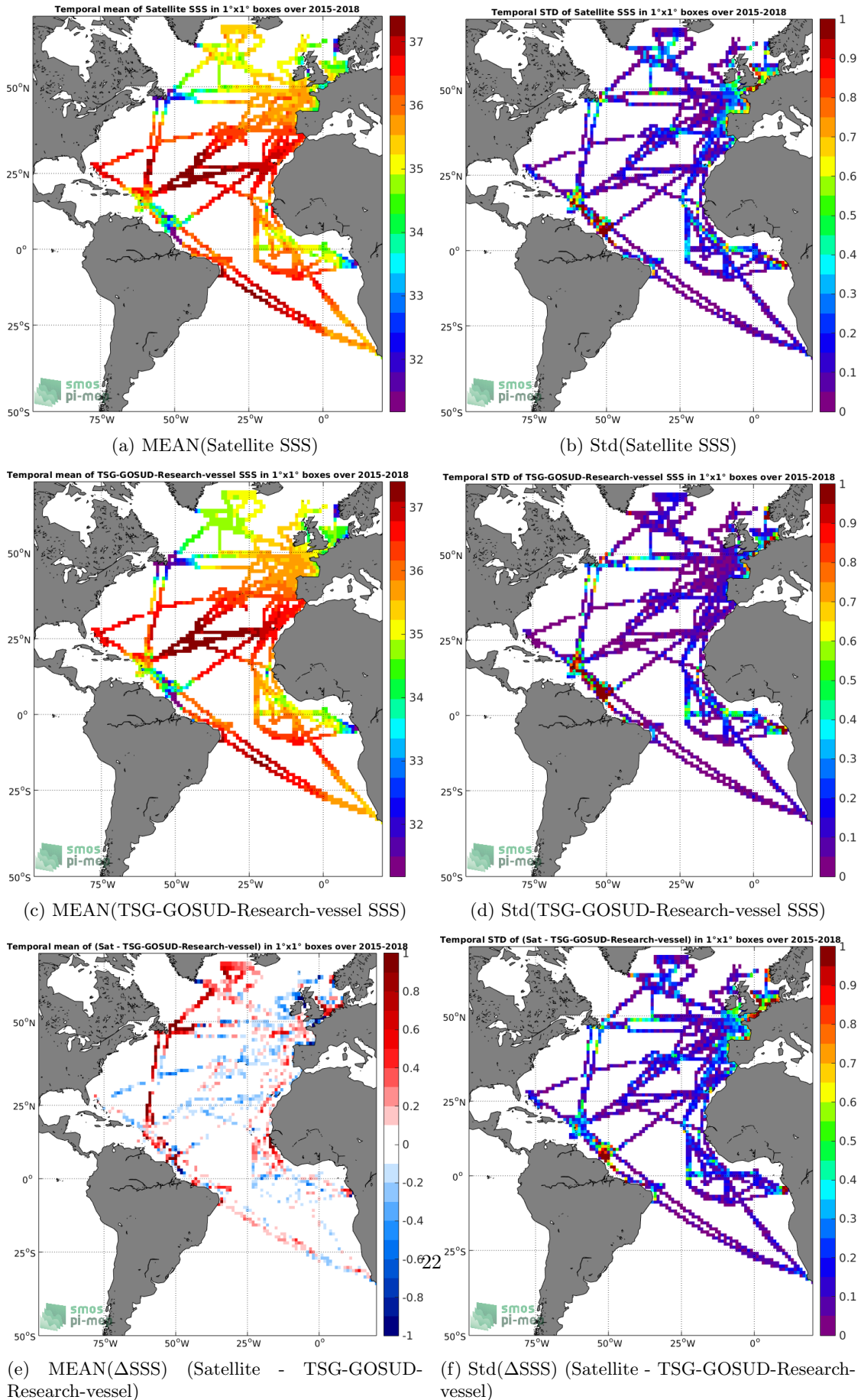
Figure 6: Temporal mean (left) and Std (right) of SSS from SMAP-L3-JPL-V4.3-8DAY-RUNNING-60KM (top), TSG-GOSUD-Research-vessel (middle), and of \Delta SSS (Satellite - TSG-GOSUD-Research-vessel). Only match-up pairs are used to generate these maps.
