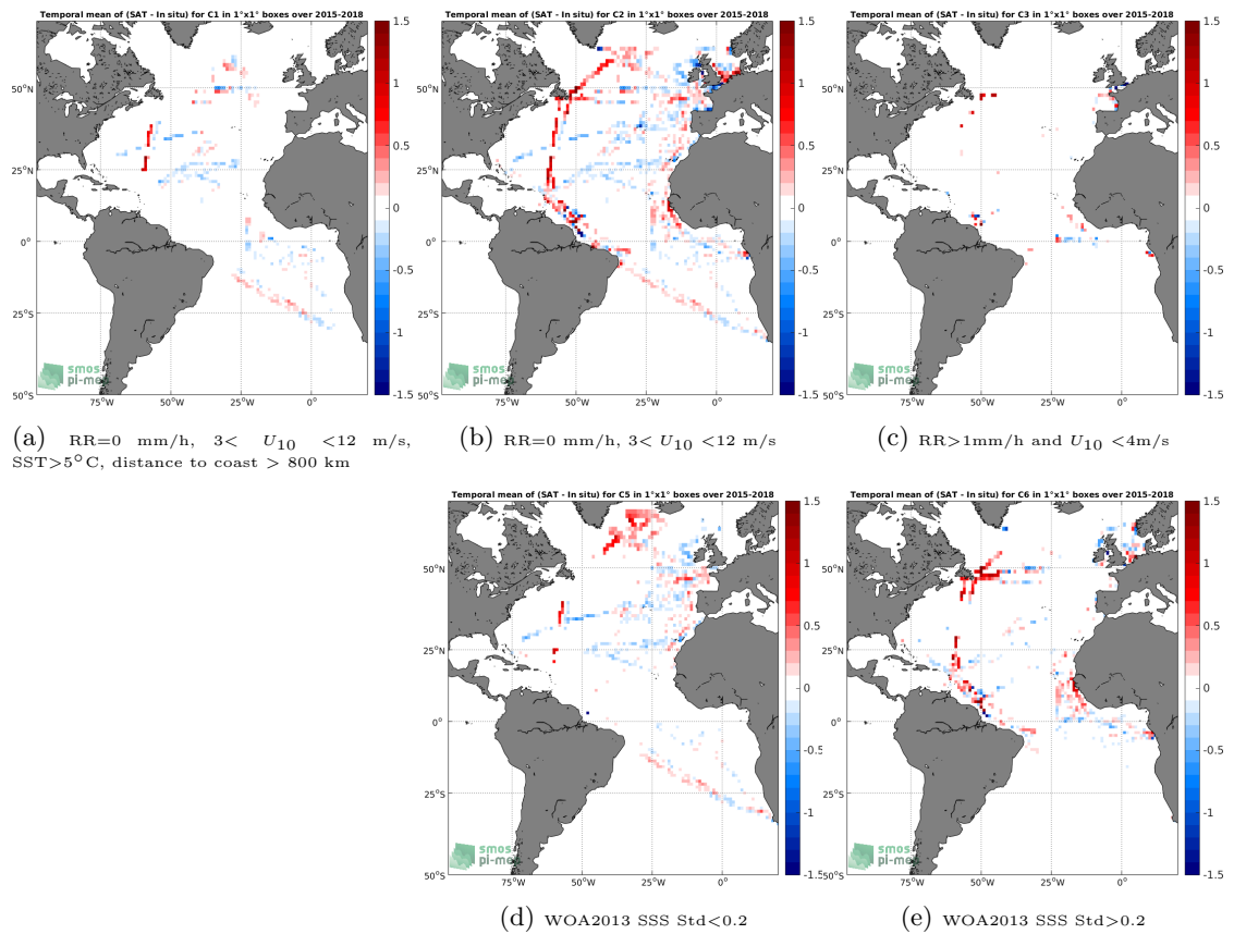
Figure 12: Temporal mean gridded over spatial boxes of size 1^\circ \times 1^\circ of \Delta SSS (SMAP-L3-JPL-V4.3-8DAY-RUNNING-60KM - TSG-GOSUD-Research-vessel) for 5 different subdatasets corresponding to:RR=0 mm/h, 3 < U_{10} < 12 m/s, SST >5^\circ\text{C} , distance to coast > 800 km (a), RR=0 mm/h, 3 < U_{10} < 12 m/s (b), RR >1 mm/h and U_{10} < 4 m/s (c), WOA2013 SSS Std <0.2 (d), WOA2013 SSS Std >0.2 (e).
