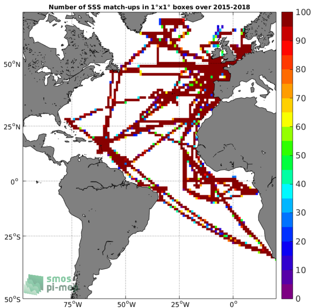
Figure 4: Number of SSS match-ups between TSG-GOSUD-Research-vessel SSS and the SMAP-L3-JPL-V4.3-8DAY-RUNNING-60KM SSS product for the Atlantic Ocean Pi-MEP region over 1°x1° boxes and for the full satellite product period.
