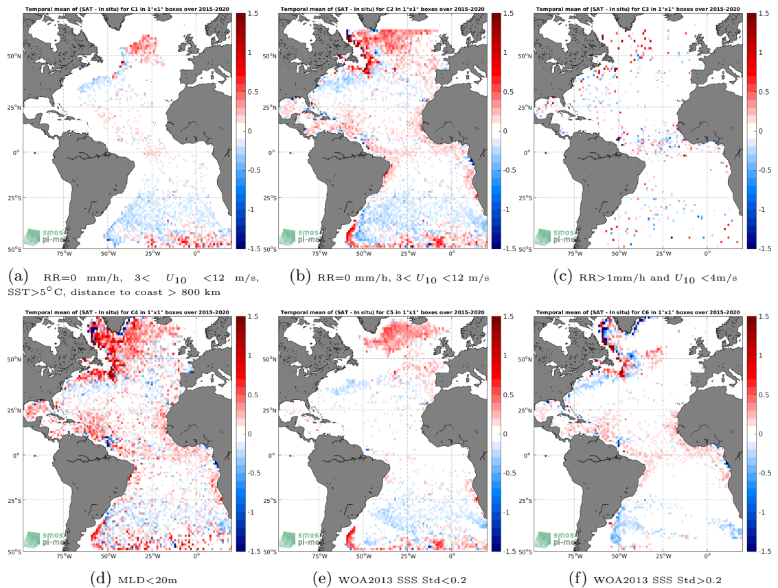
Figure 12: Temporal mean gridded over spatial boxes of size 1^\circ \times 1^\circ of \Delta SSS (SMAP-L3-JPL-V4.3-8DAY-RUNNING-60KM - Argo) for 6 different subdatasets corresponding to:RR=0 mm/h, 3 < U_{10} < 12 m/s, SST >5^\circ C, distance to coast > 800 km (a), RR=0 mm/h, 3 < U_{10} < 12 m/s (b), RR >1 mm/h and U_{10} < 4 m/s (c),MLD <20 m (d),WOA2013 SSS Std <0.2 (e),WOA2013 SSS Std >0.2 (f).
