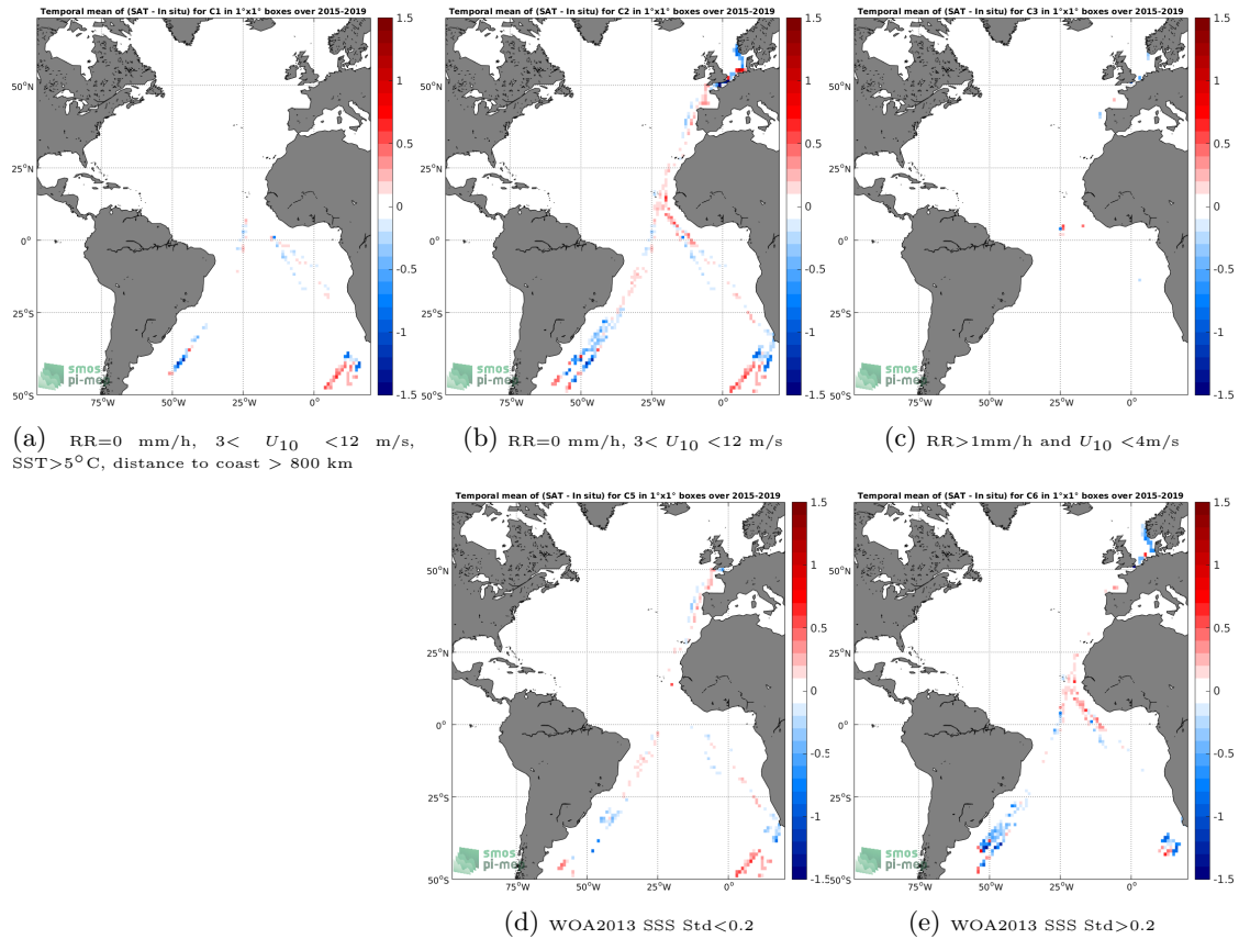
Figure 12: Temporal mean gridded over spatial boxes of size 1^\circ \times 1^\circ of \Delta SSS (SMAP-L3-JPL-V4.3-MONTHLY-60KM - TSG-POLARSTERN) for 5 different subdatasets corresponding to:RR=0 mm/h, 3 < U_{10} < 12 m/s, SST >5^\circ\text{C} , distance to coast > 800 km (a), RR=0 mm/h, 3 < U_{10} < 12 m/s (b), RR >1 mm/h and U_{10} < 4 m/s (c), WOA2013 SSS Std <0.2 (d), WOA2013 SSS Std >0.2 (e).
