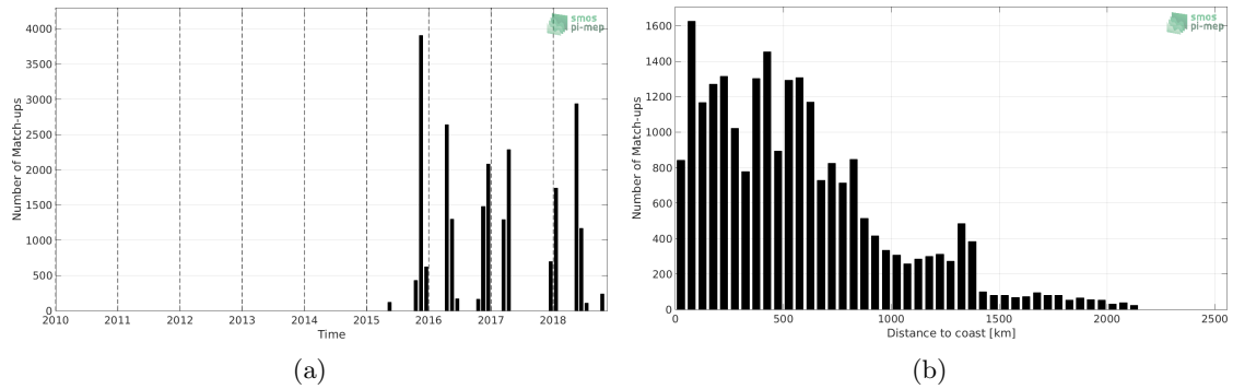
Figure 1: Number of match-ups between TSG-POLARSTERN and SMAP-L3-JPL-V4.3-MONTHLY-60KM SSS as a function of time (a) and as function of the distance to coast (b) over the Atlantic Ocean Pi-MEP region and for the full satellite product period.
