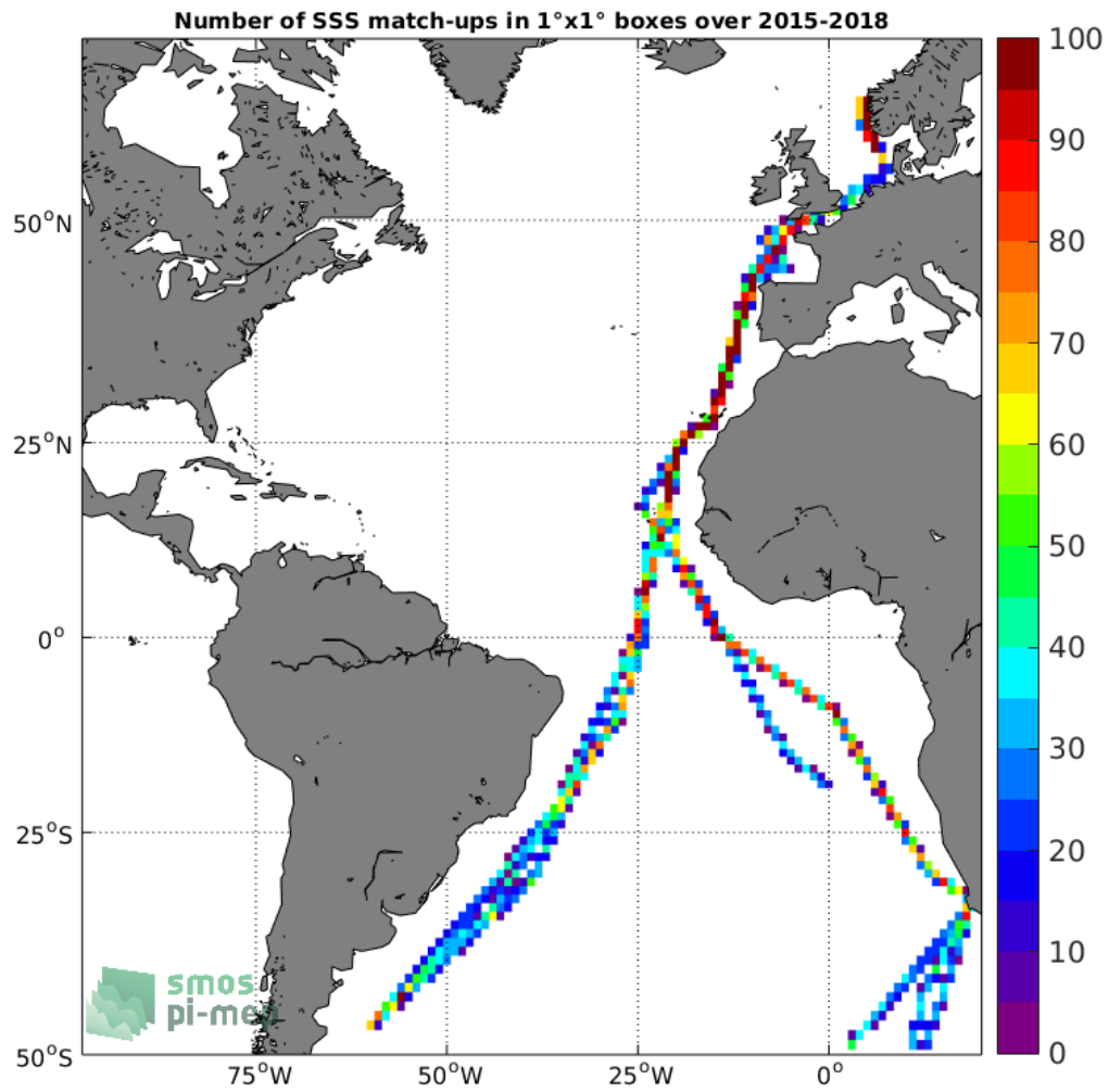
Figure 4: Number of SSS match-ups between TSG-POLARSTERN SSS and the SMAP-L3-JPL-V4.3-MONTHLY-60KM SSS product for the Atlantic Ocean Pi-MEP region over 1°x1° boxes and for the full satellite product period.
