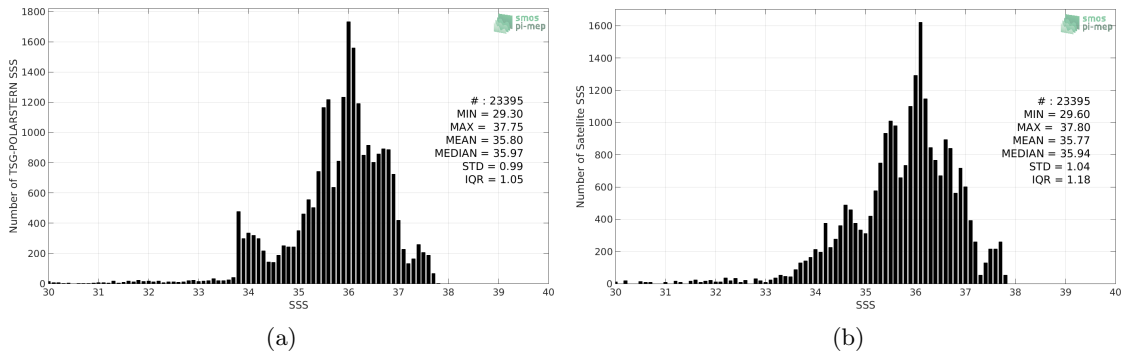
Figure 2: Histograms of SSS from TSG-POLARSTERN (a) and SMAP-L3-JPL-V4.3-MONTHLY-60KM (b) considering all match-up pairs per bins of 0.1 over the Atlantic Ocean Pi-MEP region and for the full satellite product period.
