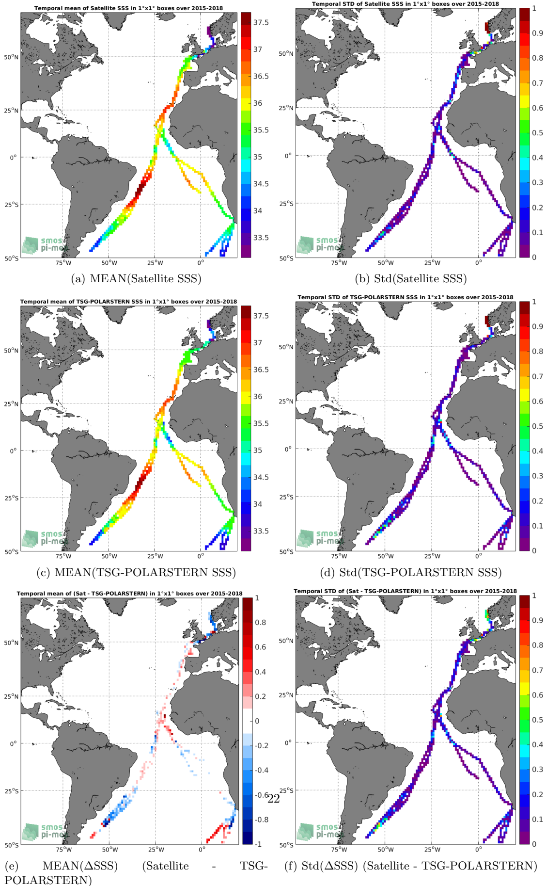
Figure 6: Temporal mean (left) and Std (right) of SSS from SMAP-L3-JPL-V4.3-MONTHLY-60KM (top), TSG-POLARSTERN (middle), and of \Delta SSS (Satellite - TSG-POLARSTERN). Only match-up pairs are used to generate these maps.
