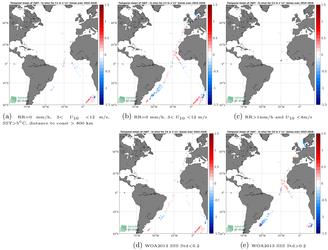
Figure 12: Temporal mean gridded over spatial boxes of size 1^\circ \times 1^\circ of \Delta SSS (SMAP-L3-JPL-V4.3-MONTHLY-60KM - TSG-POLARSTERN) for 5 different subdatasets corresponding to:RR=0 mm/h, 3 < U_{10} < 12 m/s, SST >5^\circ\text{C} , distance to coast > 800 km (a), RR=0 mm/h, 3 < U_{10} < 12 m/s (b), RR >1 mm/h and U_{10} < 4 m/s (c), WOA2013 SSS Std <0.2 (d), WOA2013 SSS Std >0.2 (e).
