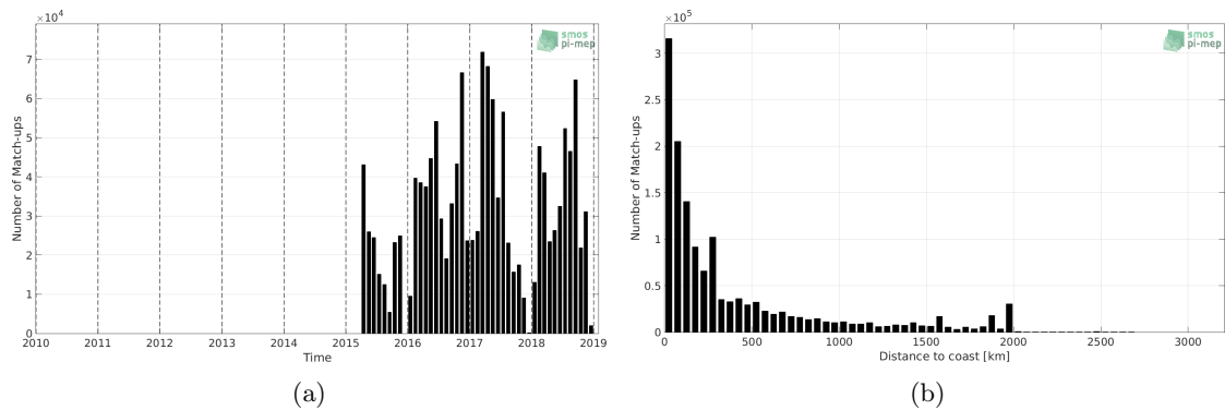
Figure 1: Number of match-ups between TSG-GOSUD-Research-vessel and SMAP-L3-JPL-V4.3-MONTHLY-60KM SSS as a function of time (a) and as function of the distance to coast (b) over the Atlantic Ocean Pi-MEP region and for the full satellite product period.
