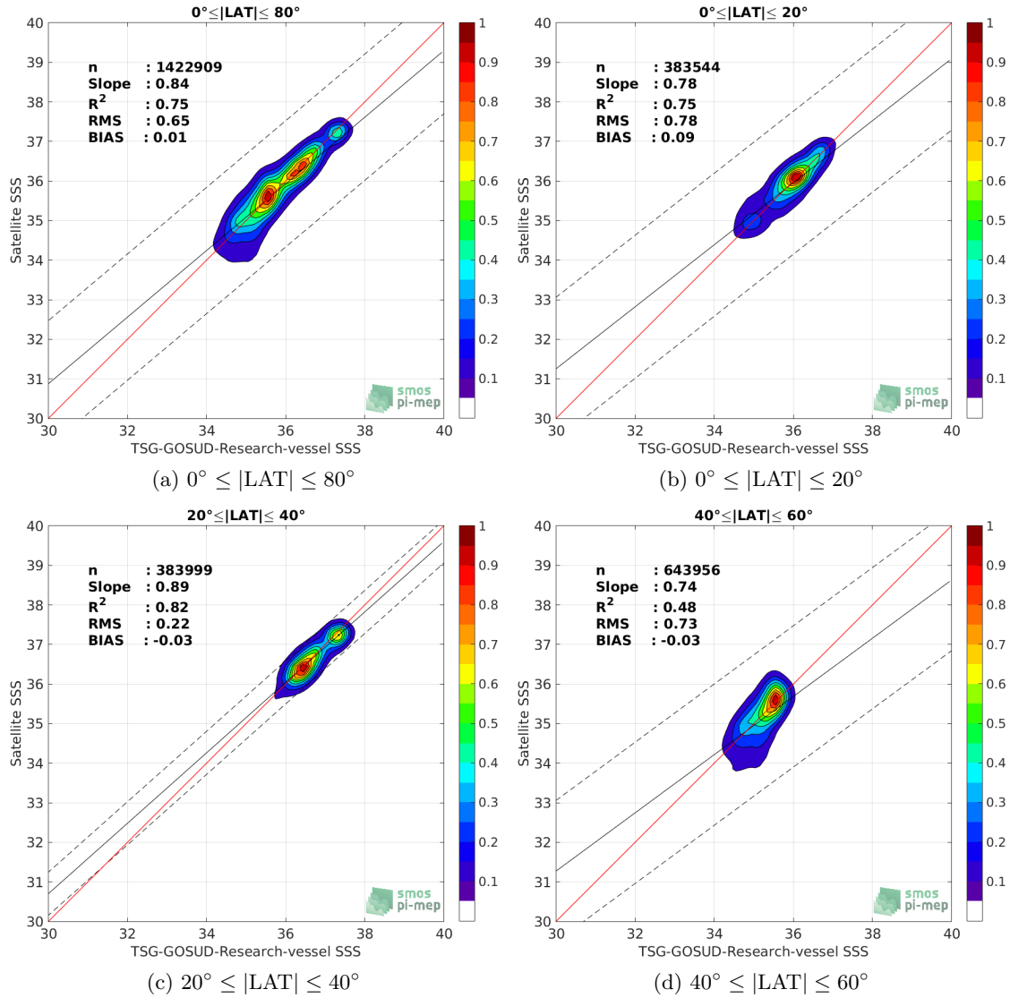
Figure 9: Contour maps of the concentration of SMAP-L3-JPL-V4.3-MONTHLY-60KM SSS (y-axis) versus TSG-GOSUD-Research-vessel SSS (x-axis) at match-up pairs for different latitude bands. For each plot, the red line shows x=y . The black thin and dashed lines indicate a linear fit through the data cloud and the \pm 95\% confidence levels, respectively. The number match-up pairs n , the slope and R^2 coefficient of the linear fit, the root mean square (RMS) and the mean bias between satellite and in situ data are indicated for each latitude band in each plots.
