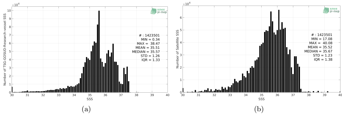
Figure 2: Histograms of SSS from TSG-GOSUD-Research-vessel (a) and SMAP-L3-JPL-V4.3-MONTHLY-60KM (b) considering all match-up pairs per bins of 0.1 over the Atlantic Ocean Pi-MEP region and for the full satellite product period.
