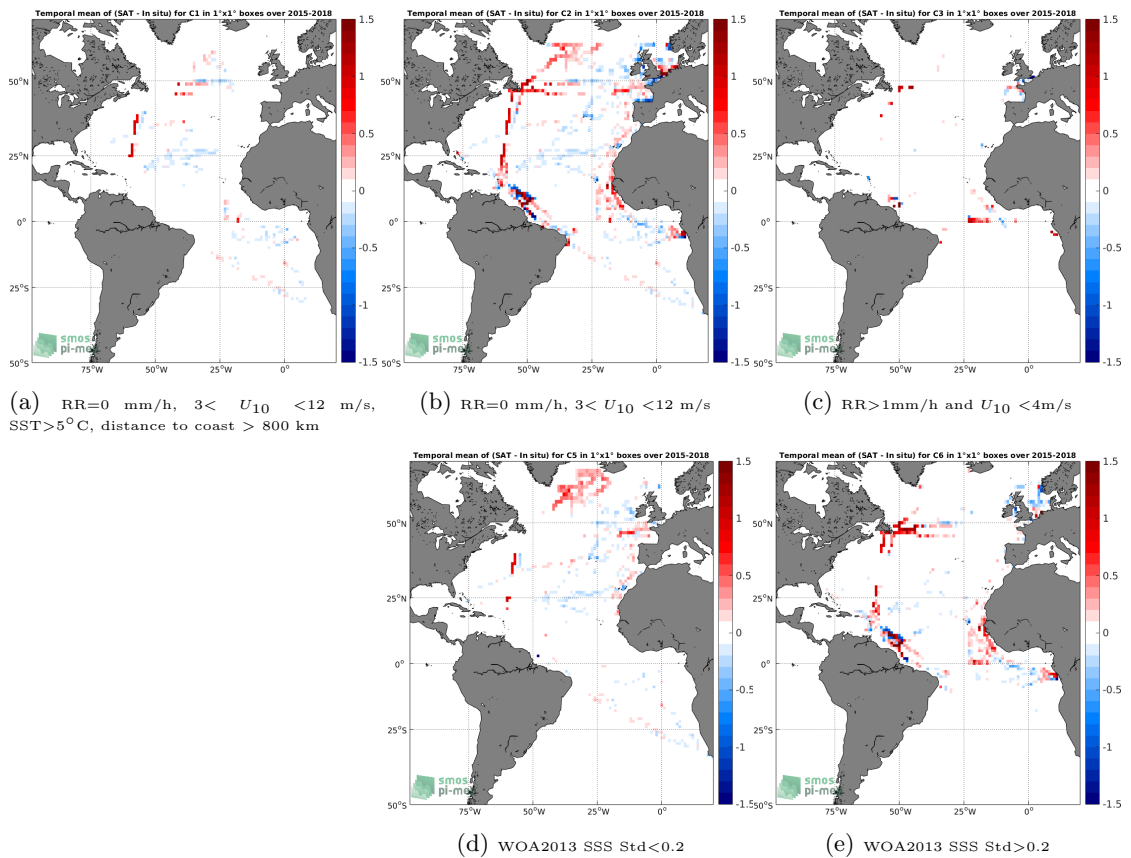
Figure 12: Temporal mean gridded over spatial boxes of size 1^\circ \times 1^\circ of \Delta SSS (SMAP-L3-JPL-V4.3-MONTHLY-60KM - TSG-GOSUD-Research-vessel) for 5 different subdatasets corresponding to:RR=0 mm/h, 3 < U_{10} < 12 m/s, SST>5°C, distance to coast > 800 km (a), RR=0 mm/h, 3 < U_{10} < 12 m/s (b), RR>1mm/h and U_{10} < 4 m/s (c), WOA2013 SSS Std<0.2 (d), WOA2013 SSS Std>0.2 (e).
