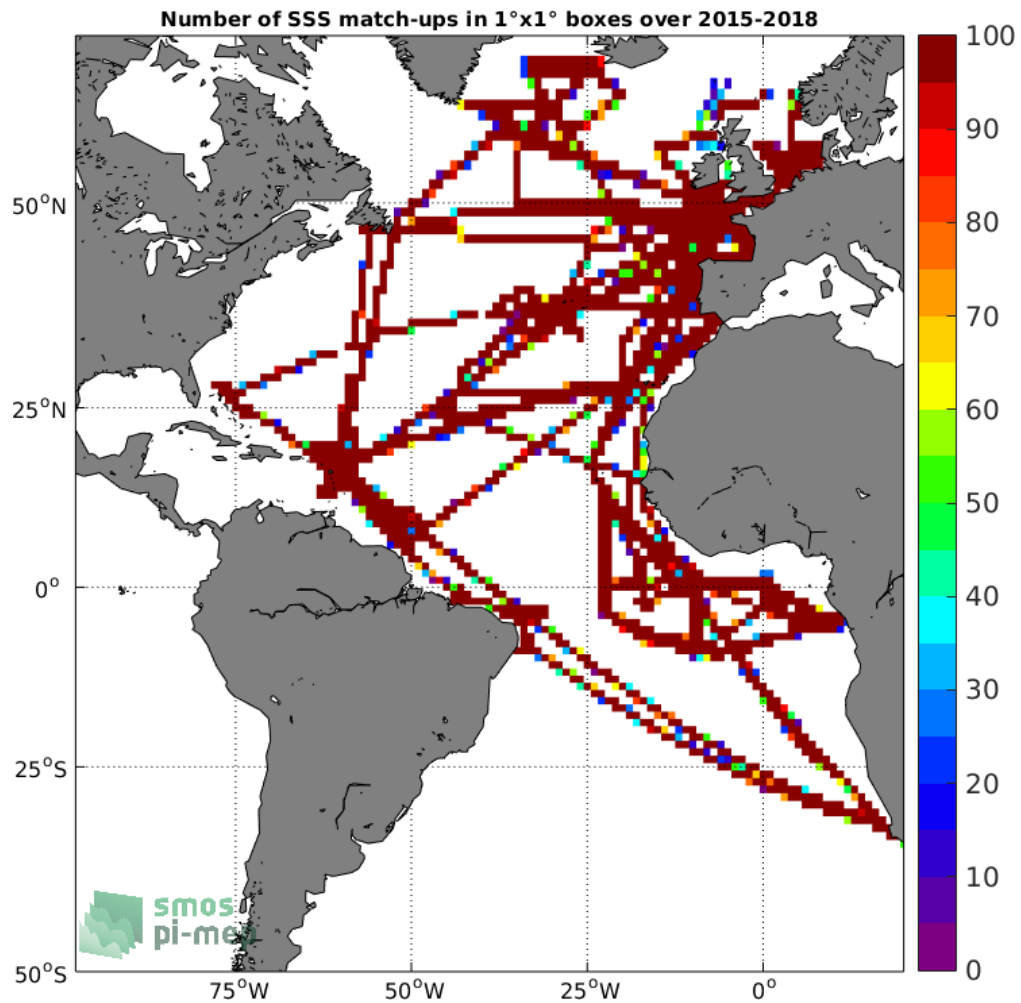
Figure 4: Number of SSS match-ups between TSG-GOSUD-Research-vessel SSS and the SMAP-L3-JPL-V4.3-MONTHLY-60KM SSS product for the Atlantic Ocean Pi-MEP region over 1°x1° boxes and for the full satellite product period.
